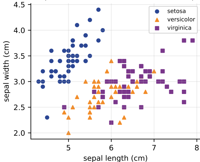
Sepal measurements — classes overlap
