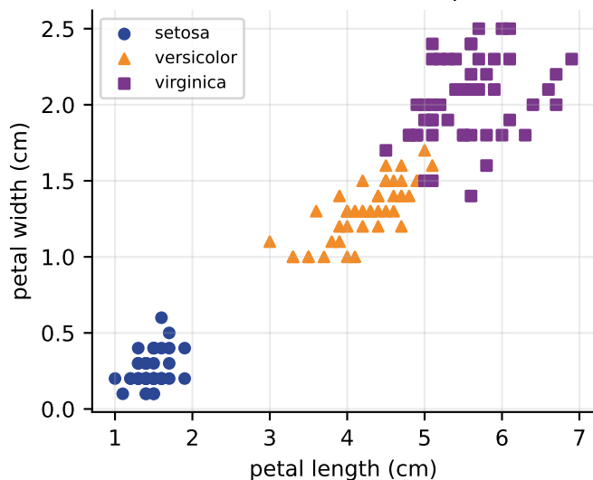
Petal measurements — setosa separates cleanly
