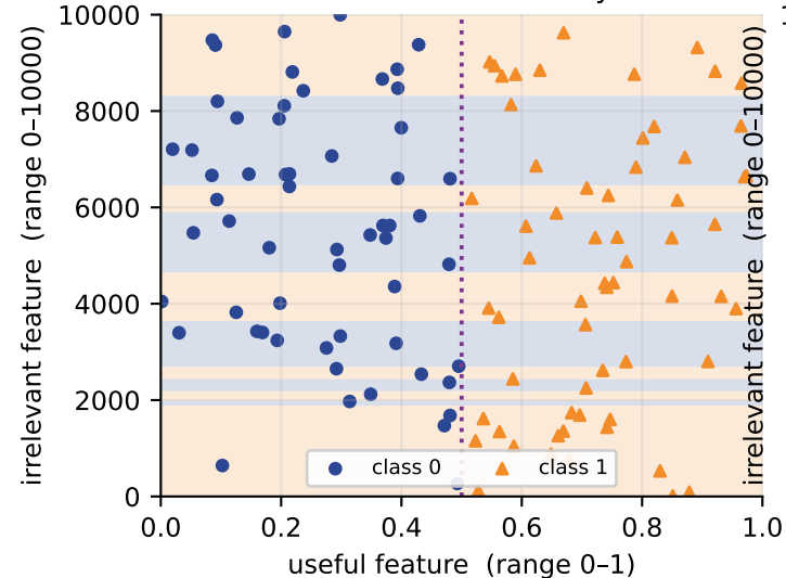
Unscaled — test accuracy 0.50
