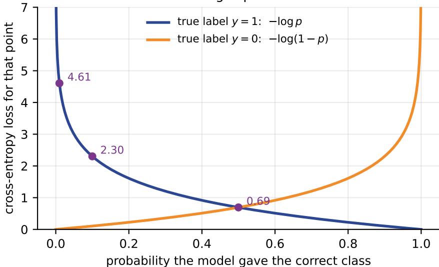
Confident and wrong is punished without limit
