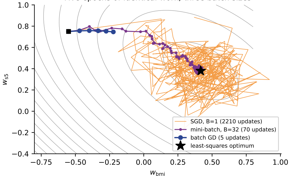
Five epochs of identical work, three batch sizes
