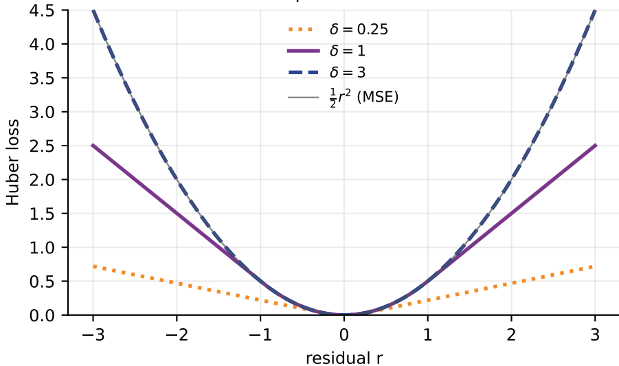
\delta sets where quadratic becomes linear
