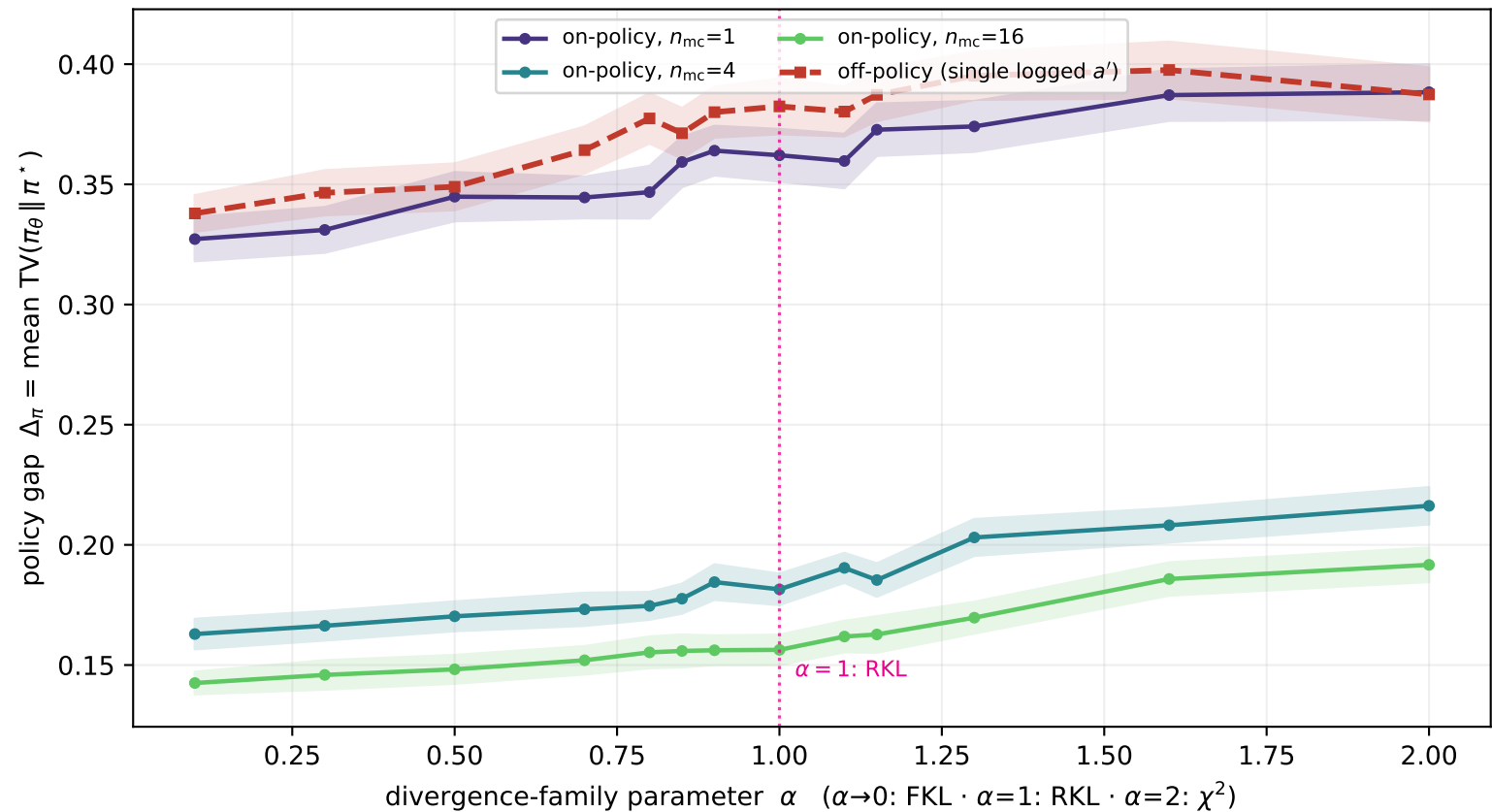
\alpha -family vs Monte-Carlo budget — layered MDP, 100 MDPs, \pm 95\% CI (temperature pinned to RKL@peak 0.7)
