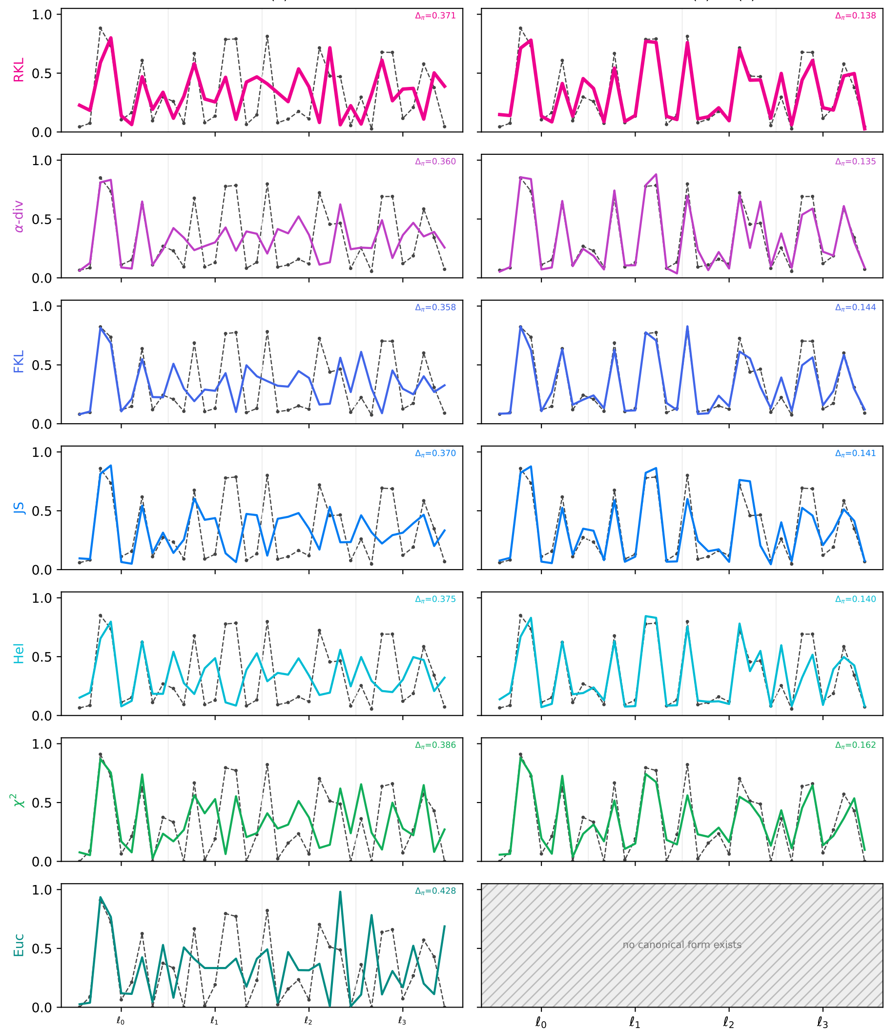
Amari f'(1) = 0
