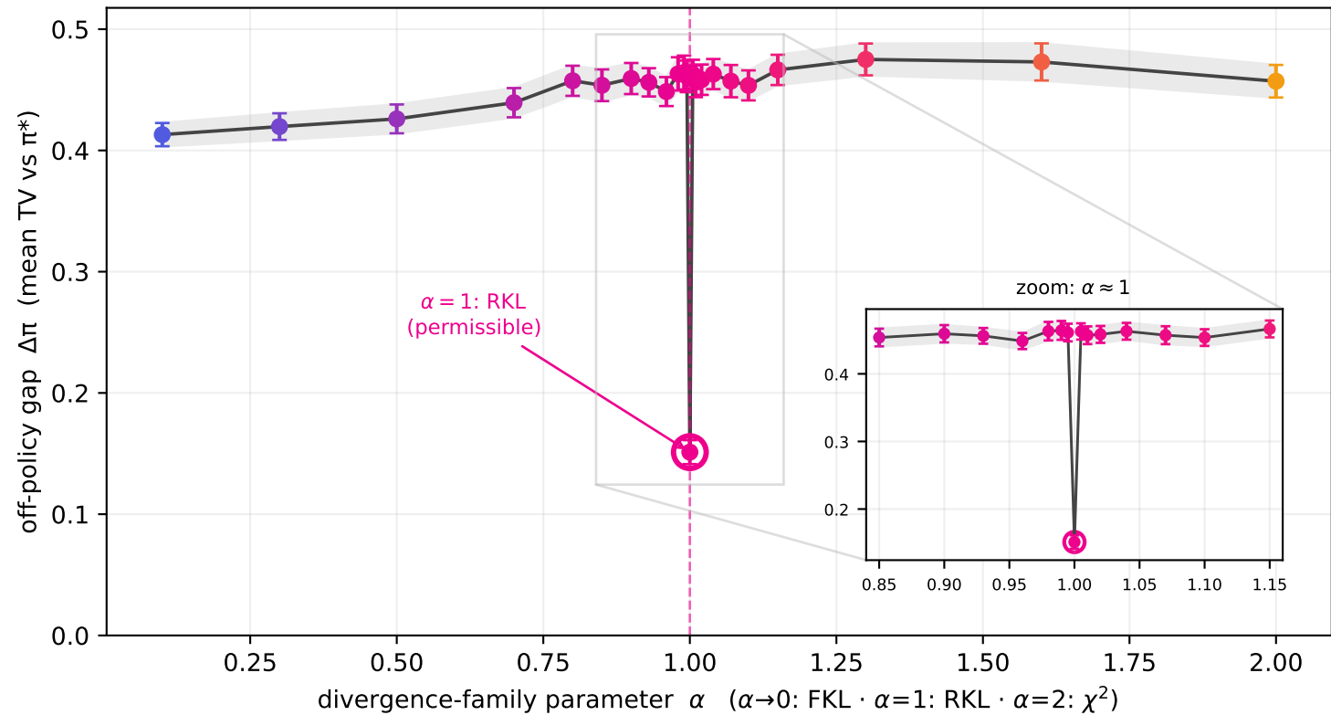
\alpha -div sweep · standard normalization f'(1) = 0
