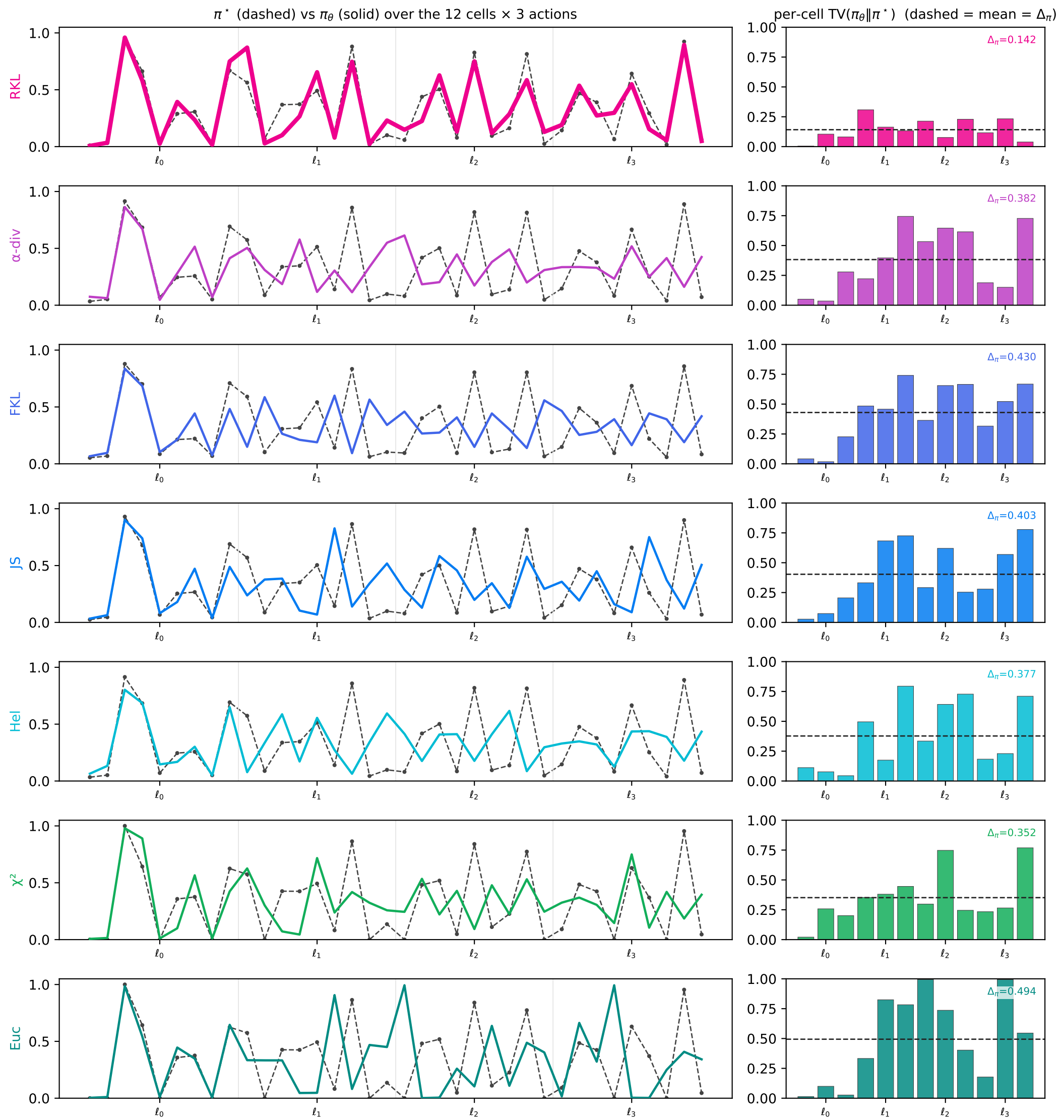
Per-(layer, state) anatomy — off-policy (single logged a' ), n_{mc}=1 , peak 0.7, MDP 0
