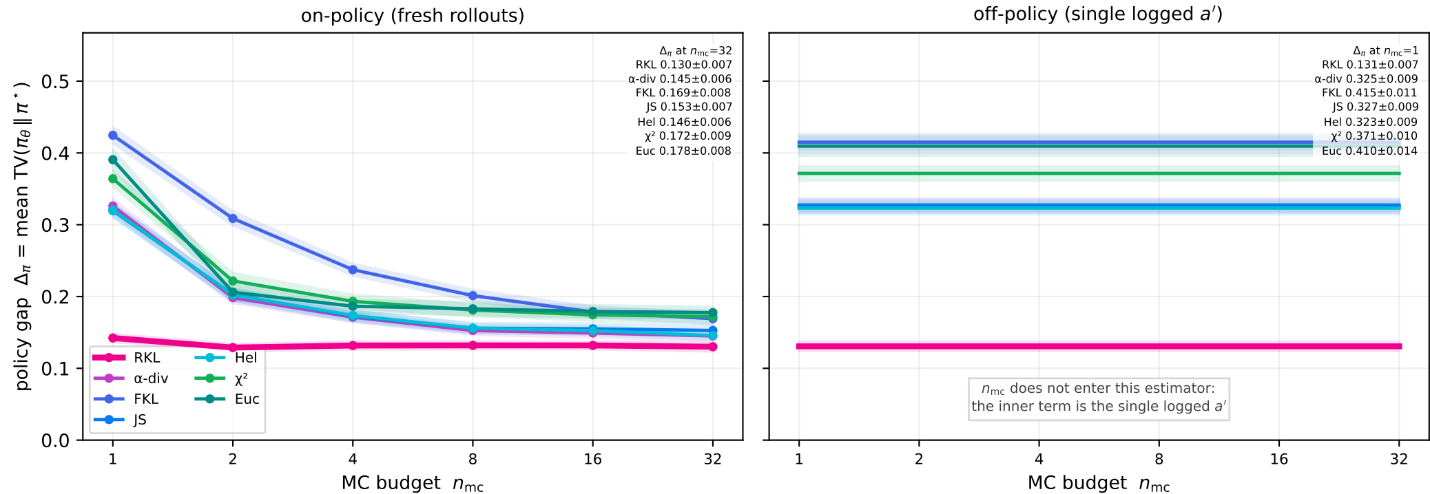
Recovery under a PEAKED reference \pi_{\text{ref}}=(0.6, 0.2, 0.2) — layered MDP, 100 MDPs, \pm 95\% CI
