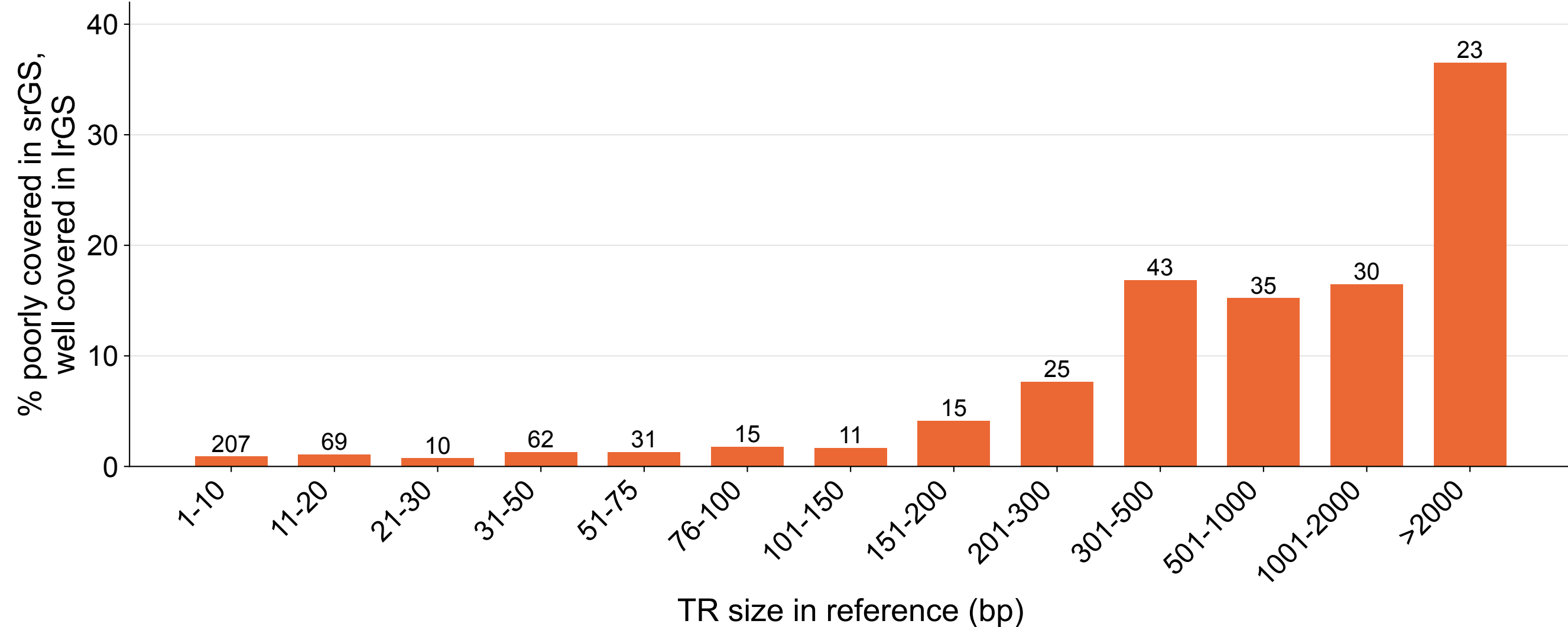
Proportion poorly covered by srGS only (srGS < 0.5x and lrGS \geq 0.7x of genome mean in any 100 bp bin)
