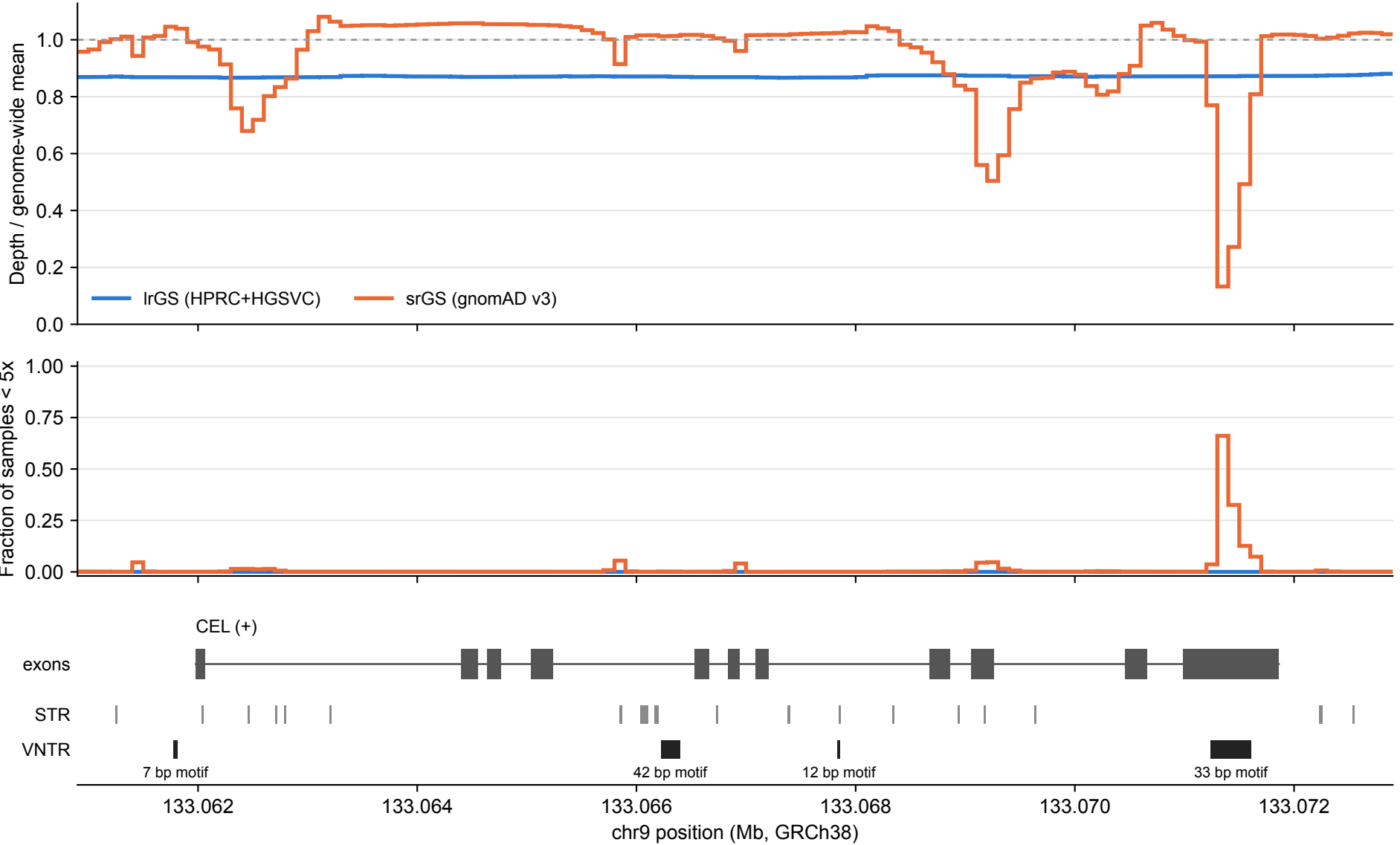
CEL: IrGS vs srGS coverage over tandem repeats (100 bp bins)
