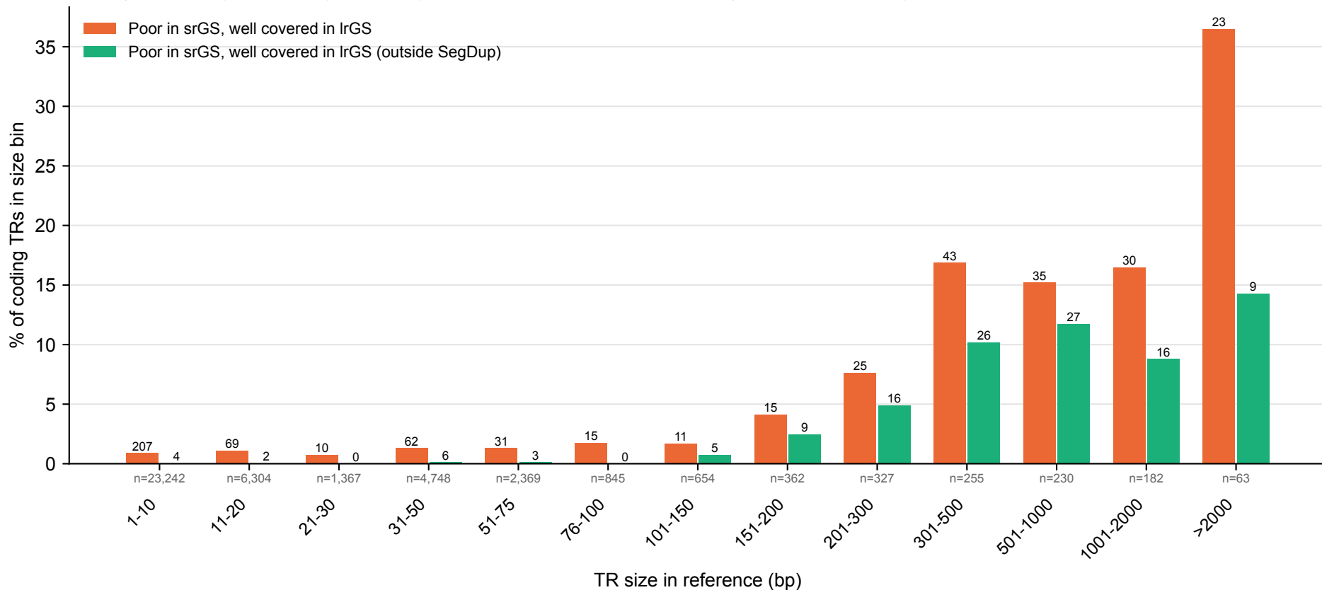
Coding TRs poorly covered by srGS only (srGS < 0.5x and lrGS >= 0.7x of genome mean in any 100 bp bin)
