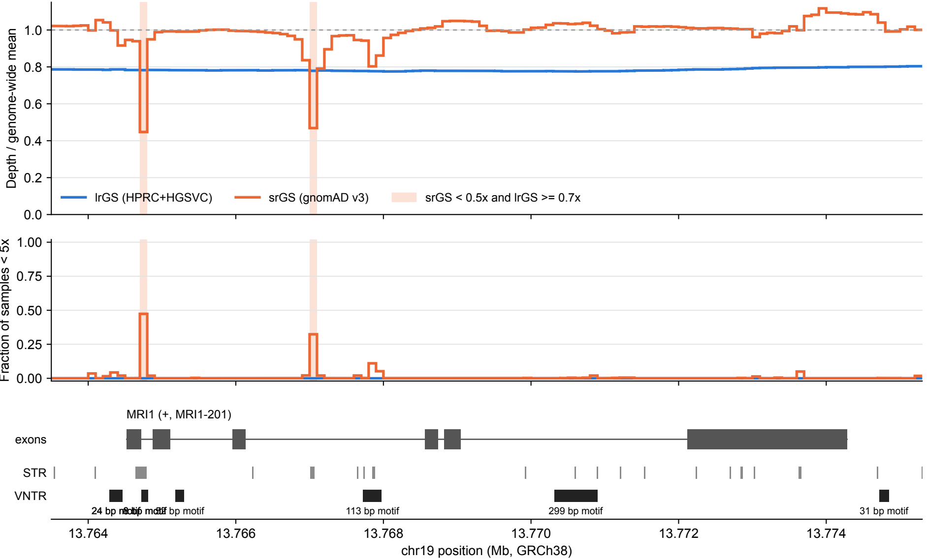
MRI1: IrGS vs srGS coverage over tandem repeats (100 bp bins)
