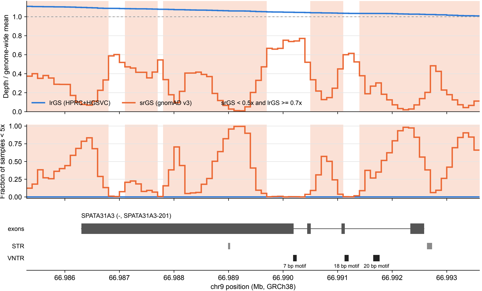
SPATA31A3: lrGS vs srGS coverage over tandem repeats (100 bp bins)
