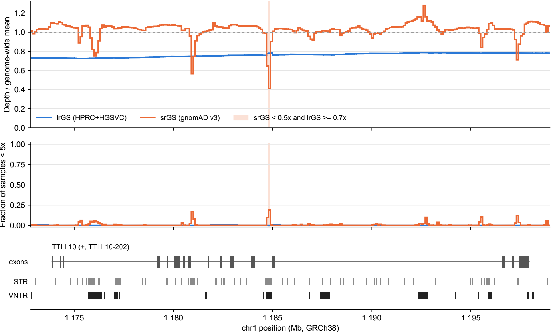
TTLL10: IrGS vs srGS coverage over tandem repeats (100 bp bins)
