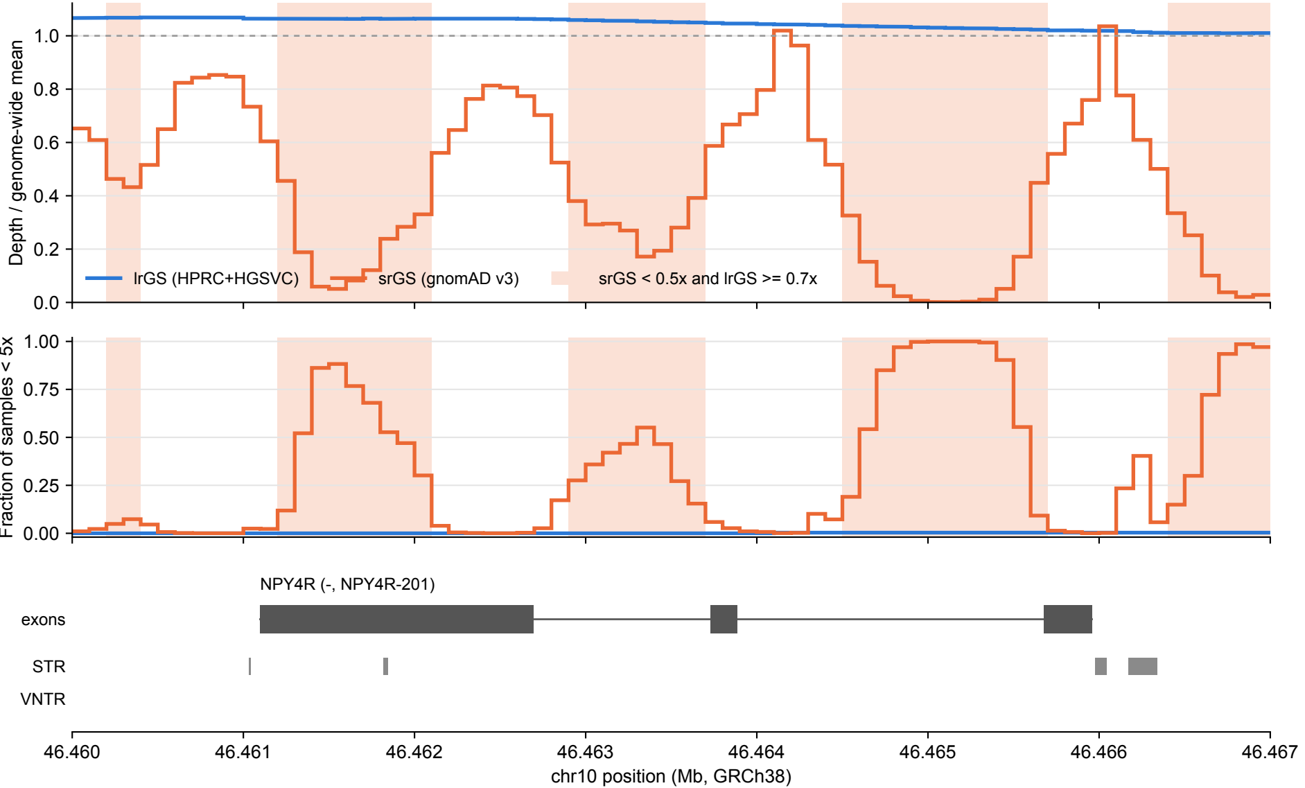
NPY4R: lrGS vs srGS coverage over tandem repeats (100 bp bins)
