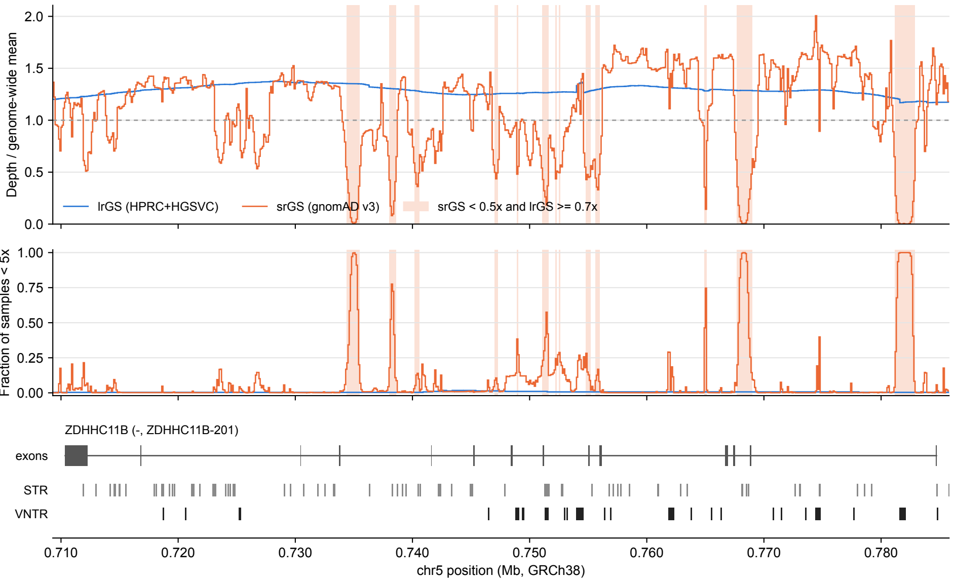
ZDHHC11B: lrGS vs srGS coverage over tandem repeats (100 bp bins)
