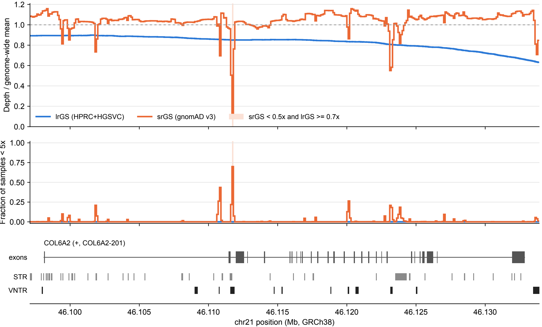
COL6A2: lrGS vs srGS coverage over tandem repeats (100 bp bins)
