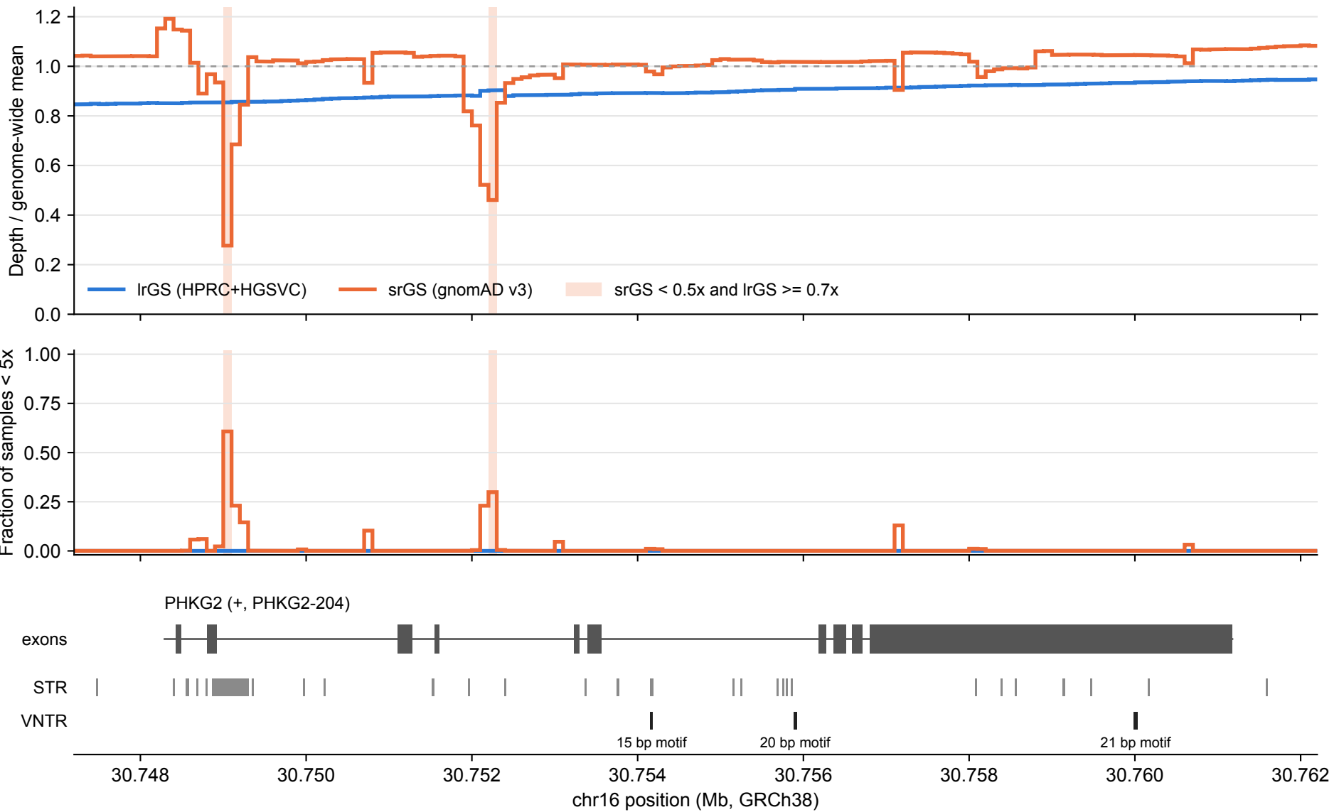
PHKG2: lrGS vs srGS coverage over tandem repeats (100 bp bins)
