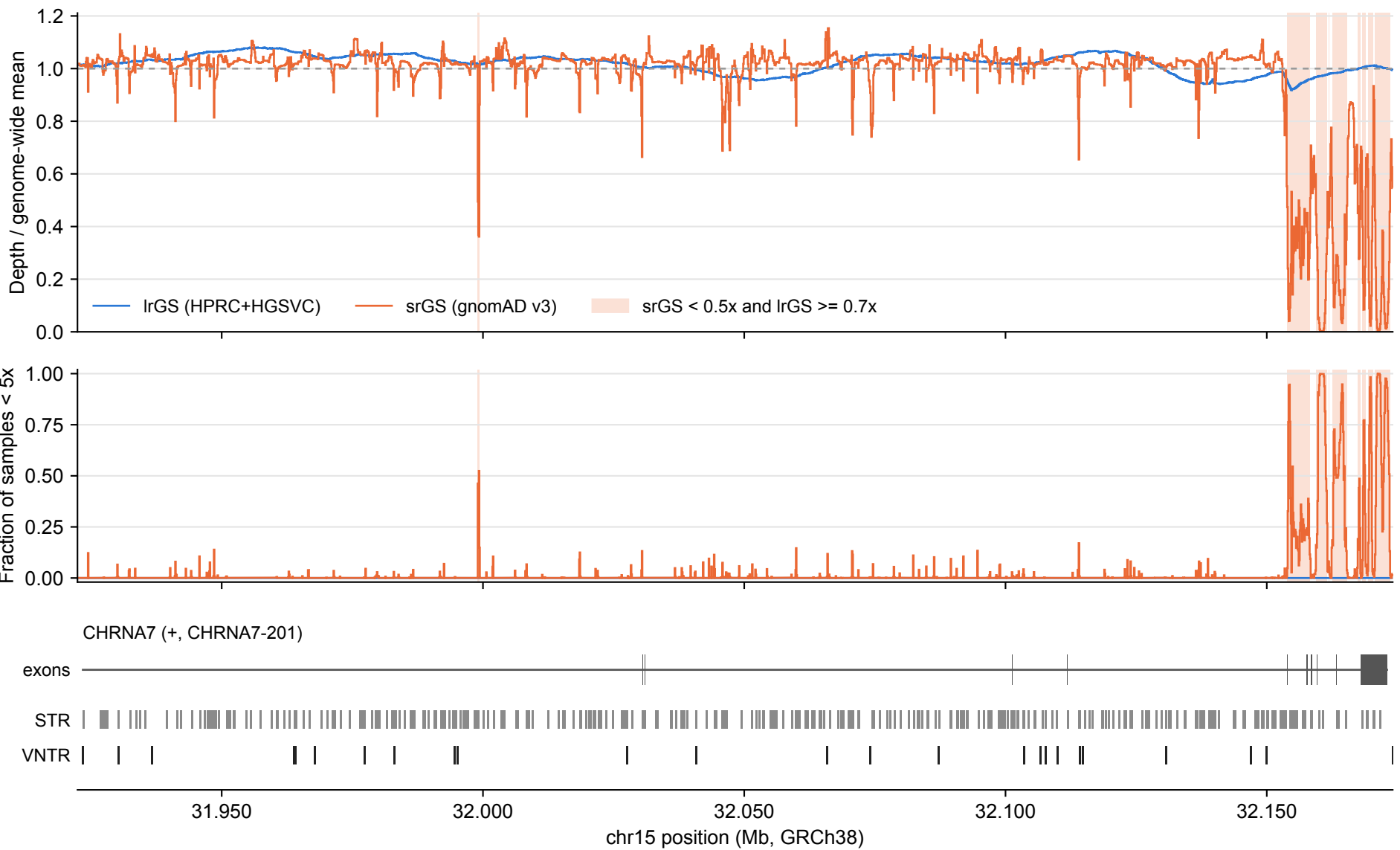
CHRNA7: lrGS vs srGS coverage over tandem repeats (100 bp bins)
