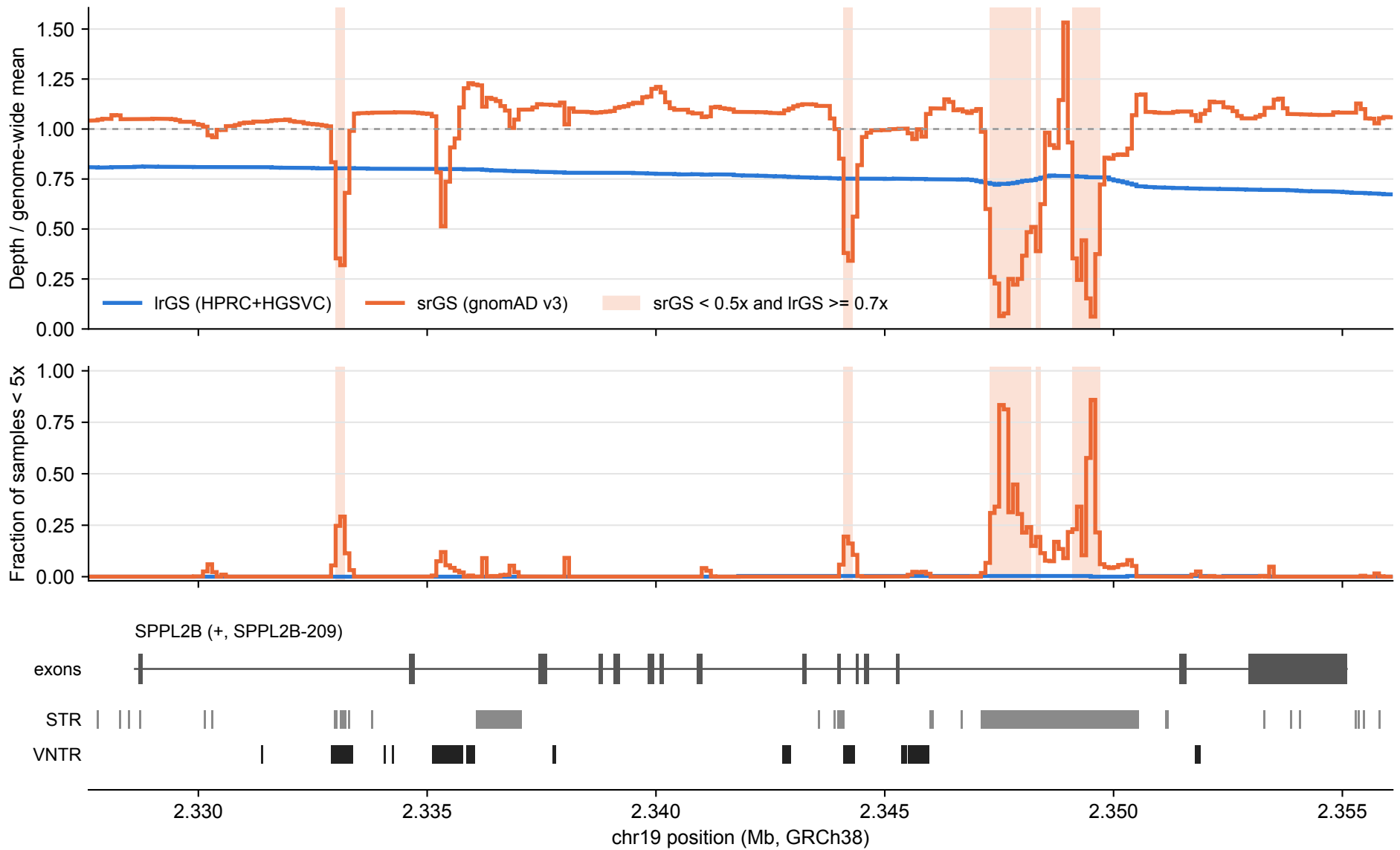
SPPL2B: lrGS vs srGS coverage over tandem repeats (100 bp bins)
