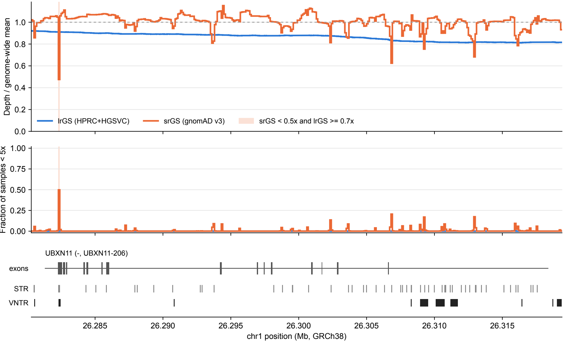
UBXN11: lrGS vs srGS coverage over tandem repeats (100 bp bins)
