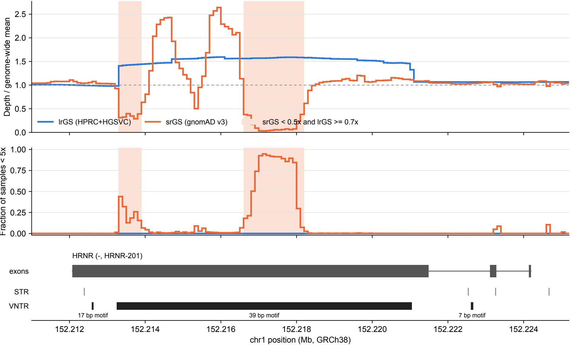
HRNR: lrGS vs srGS coverage over tandem repeats (100 bp bins)
