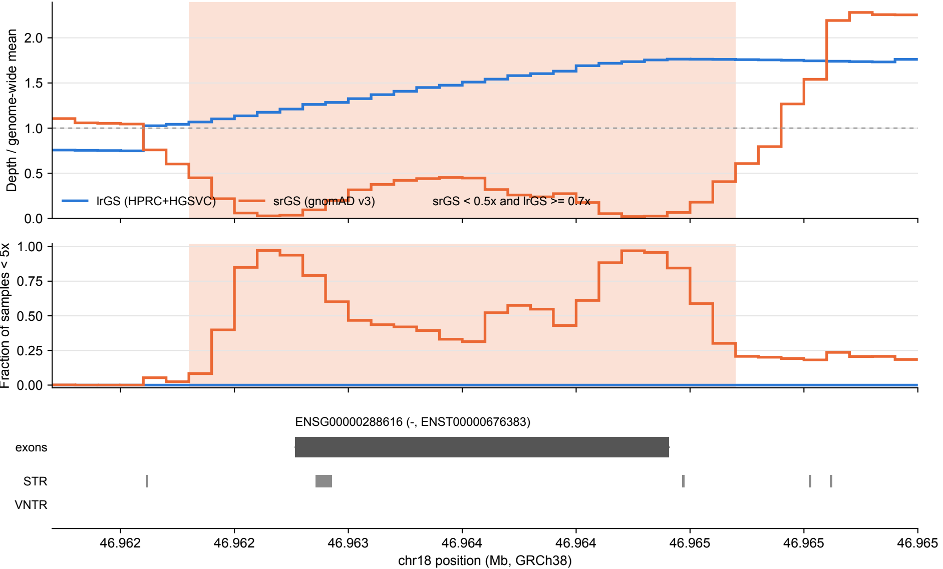
ENSG00000288616: lrGS vs srGS coverage over tandem repeats (100 bp bins)
