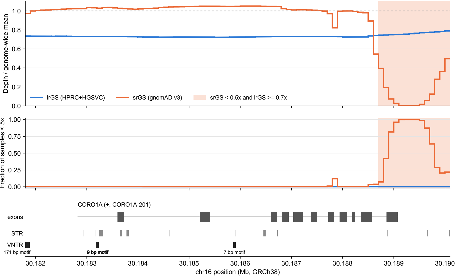
CORO1A: lrGS vs srGS coverage over tandem repeats (100 bp bins)
