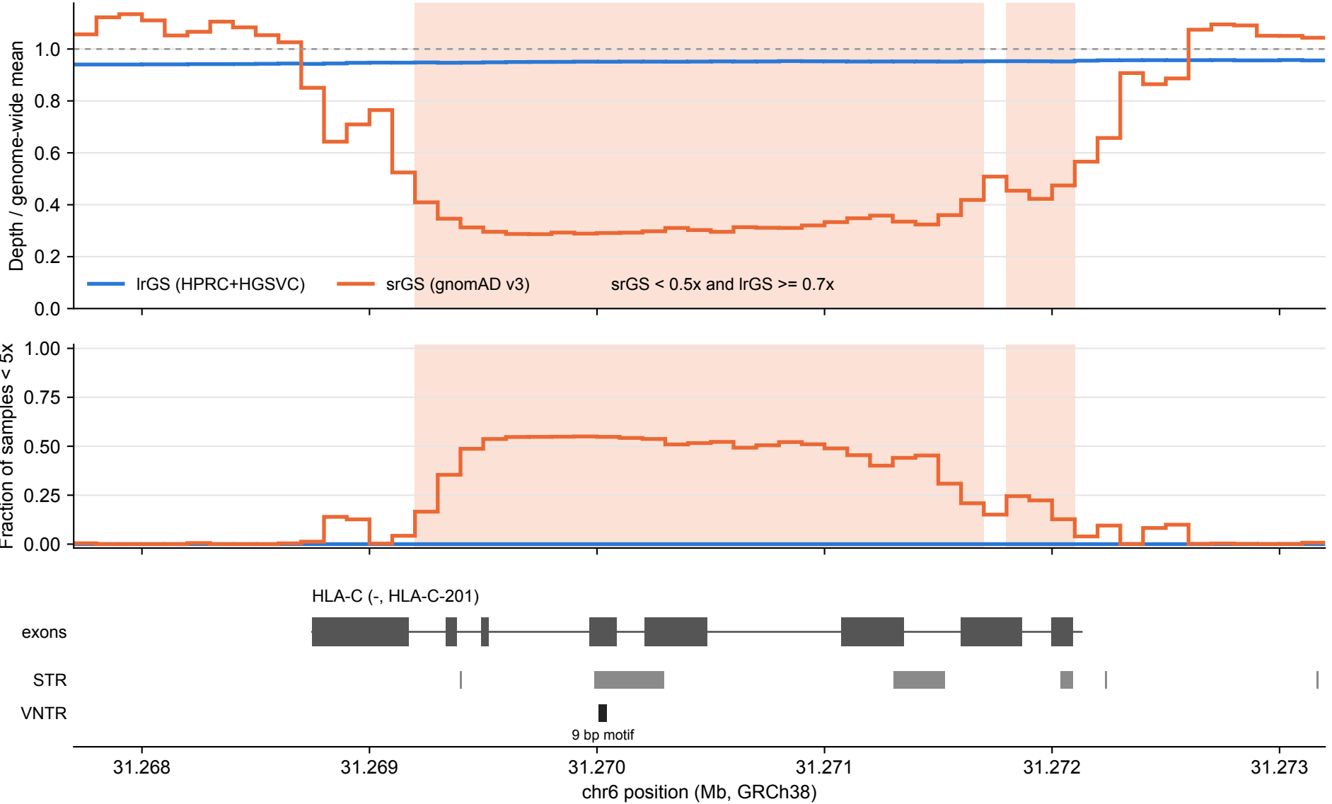
HLA-C: IrGS vs srGS coverage over tandem repeats (100 bp bins)
