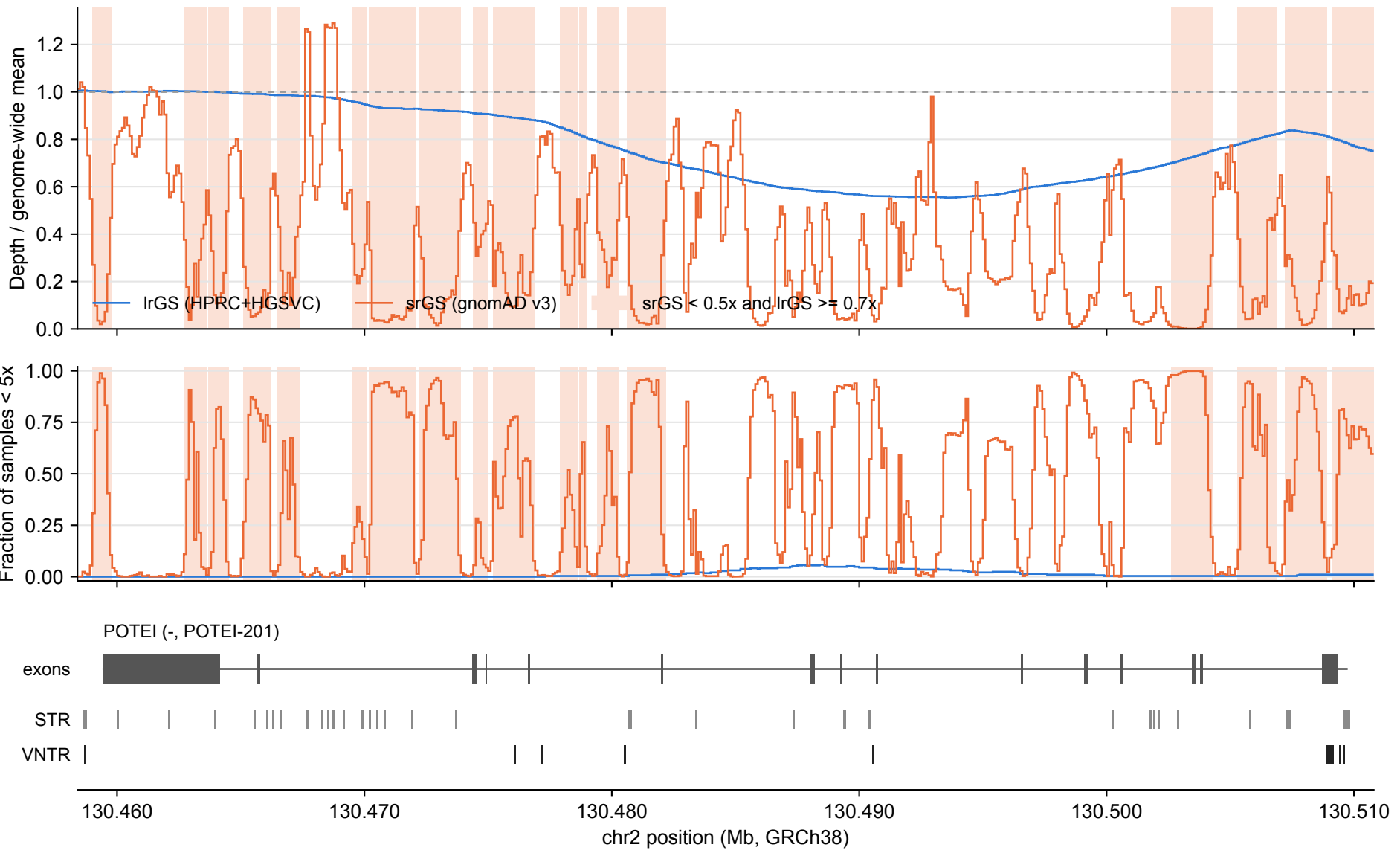
POTEI: IrGS vs srGS coverage over tandem repeats (100 bp bins)
