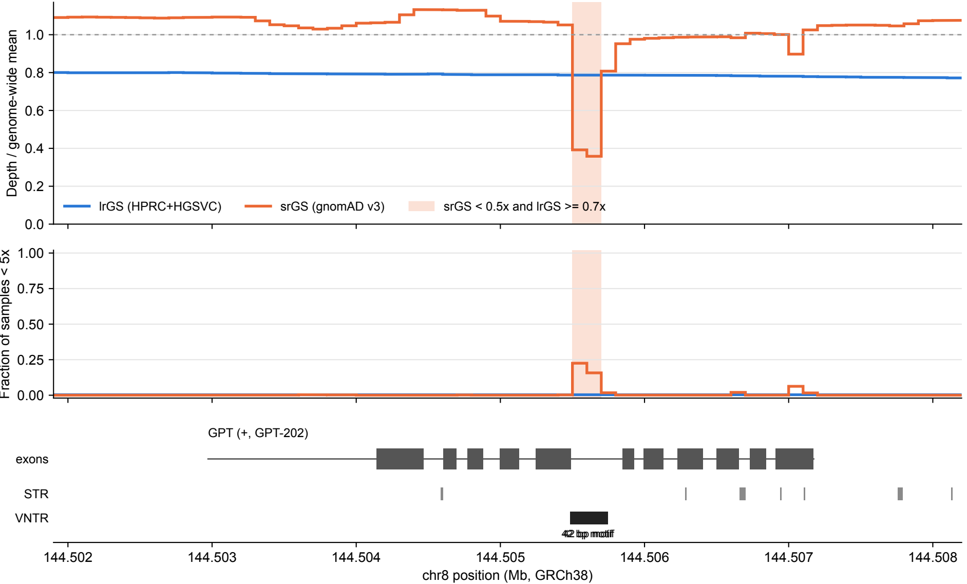
GPT: IrGS vs srGS coverage over tandem repeats (100 bp bins)
