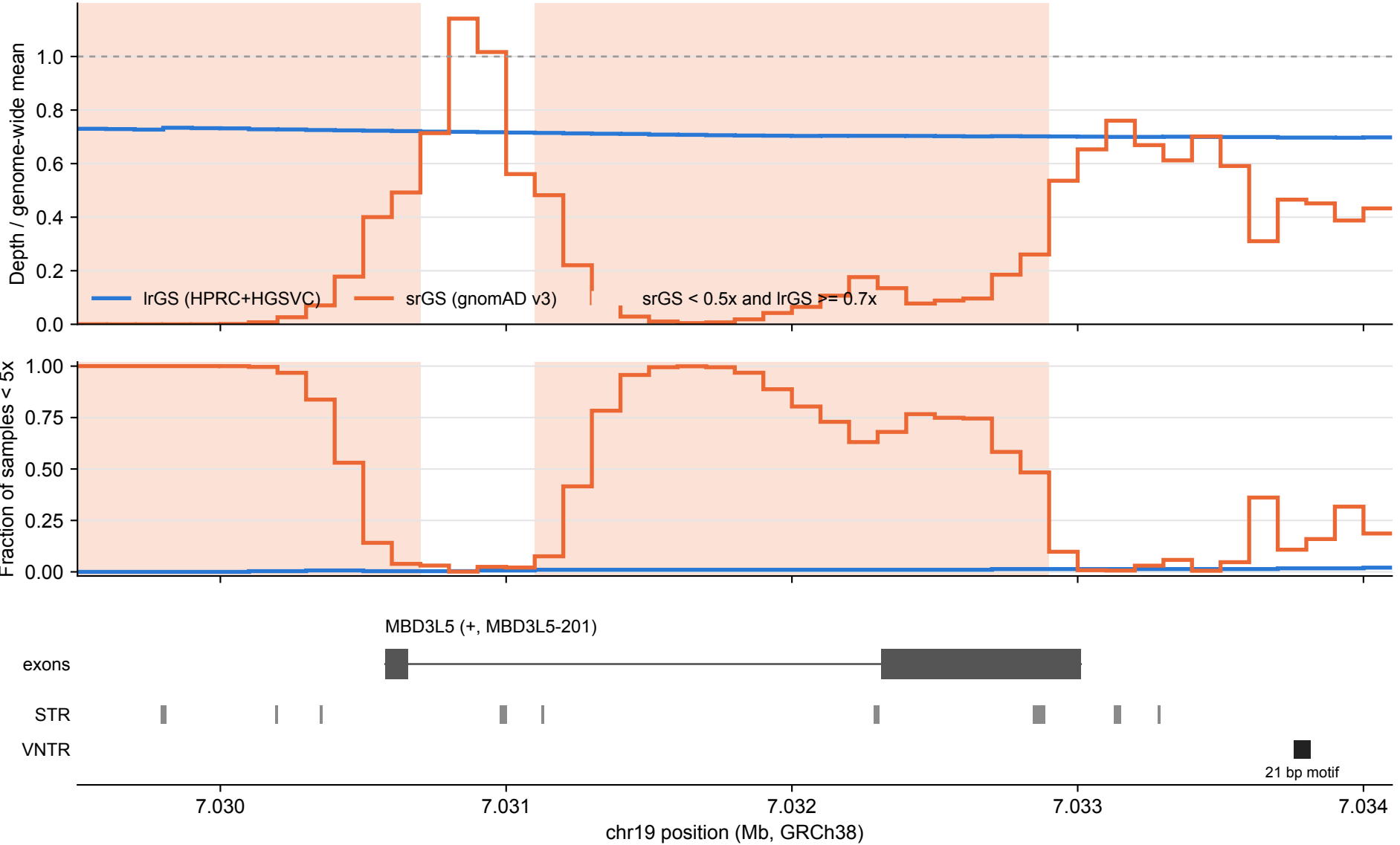
MBD3L5: lrGS vs srGS coverage over tandem repeats (100 bp bins)
