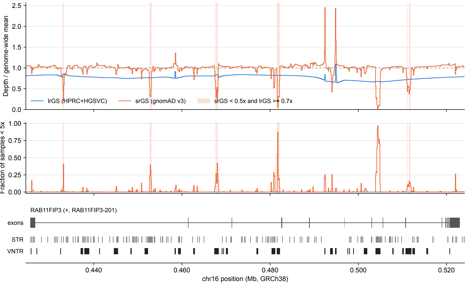
RAB11FIP3: lrGS vs srGS coverage over tandem repeats (100 bp bins)
