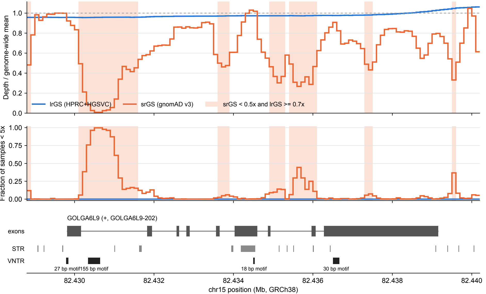
GOLGA6L9: lrGS vs srGS coverage over tandem repeats (100 bp bins)
