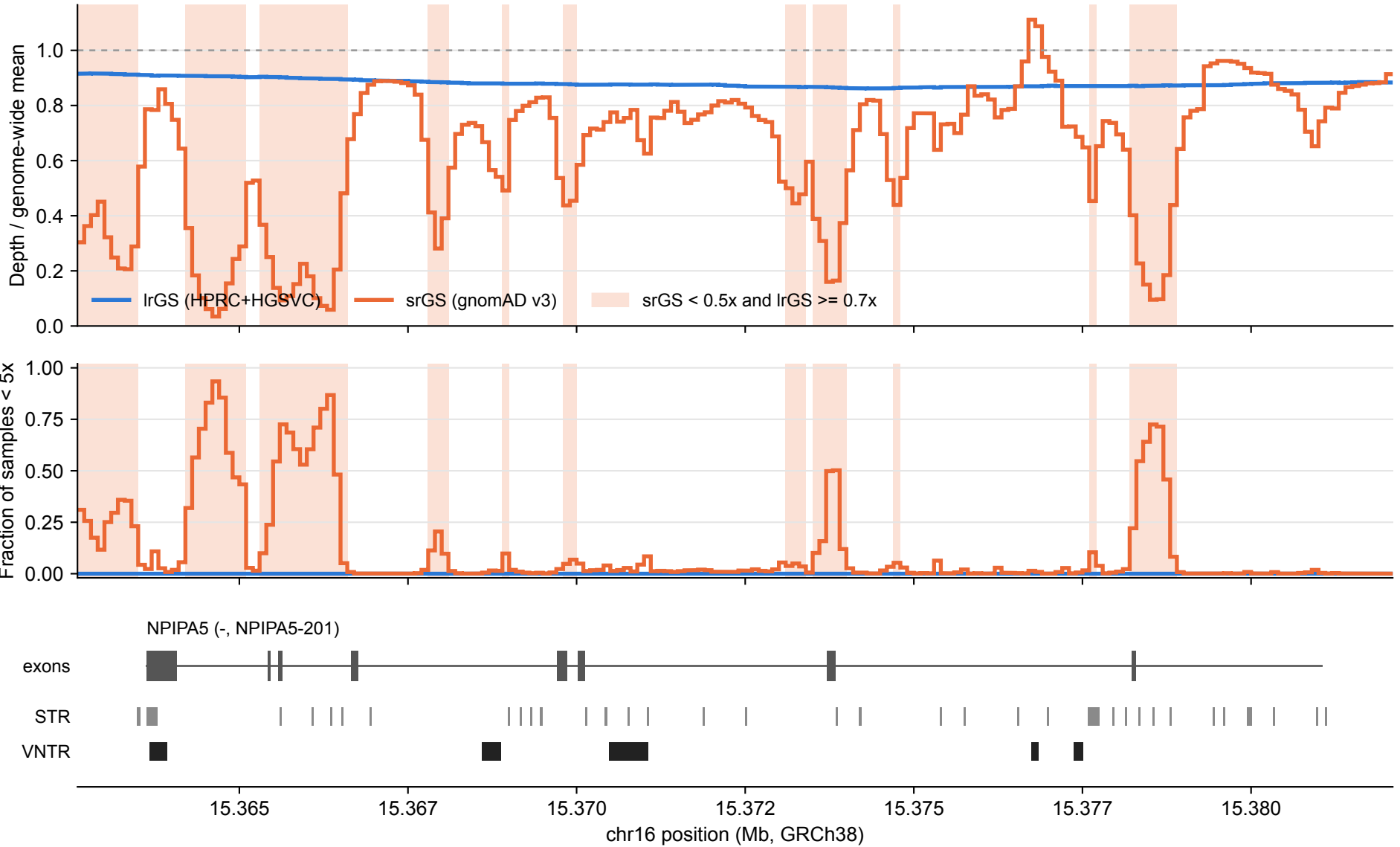
NPIPA5: IrGS vs srGS coverage over tandem repeats (100 bp bins)
