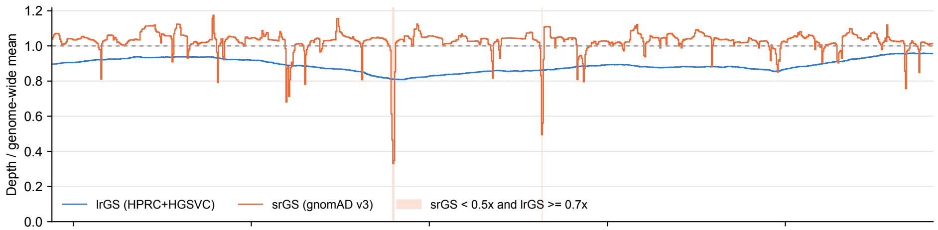
SNED1: lrGS vs srGS coverage over tandem repeats (100 bp bins)
