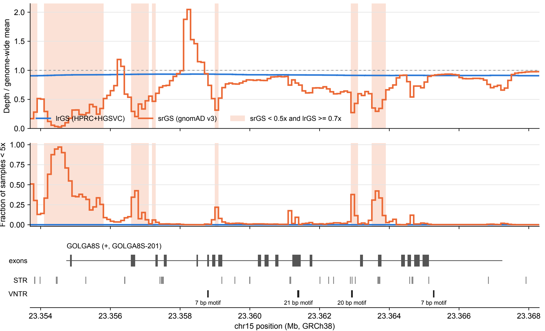
GOLGA8S: lrGS vs srGS coverage over tandem repeats (100 bp bins)
