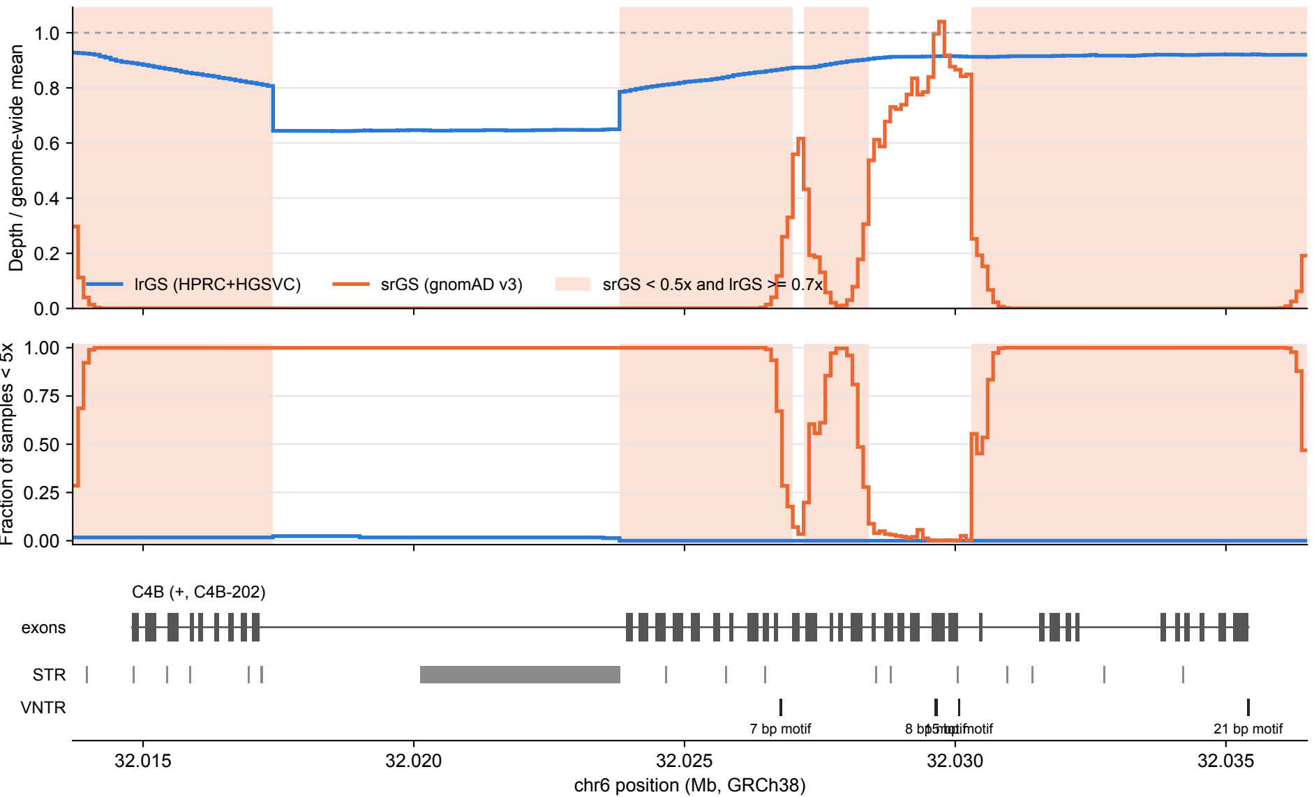
C4B: IrGS vs srGS coverage over tandem repeats (100 bp bins)
