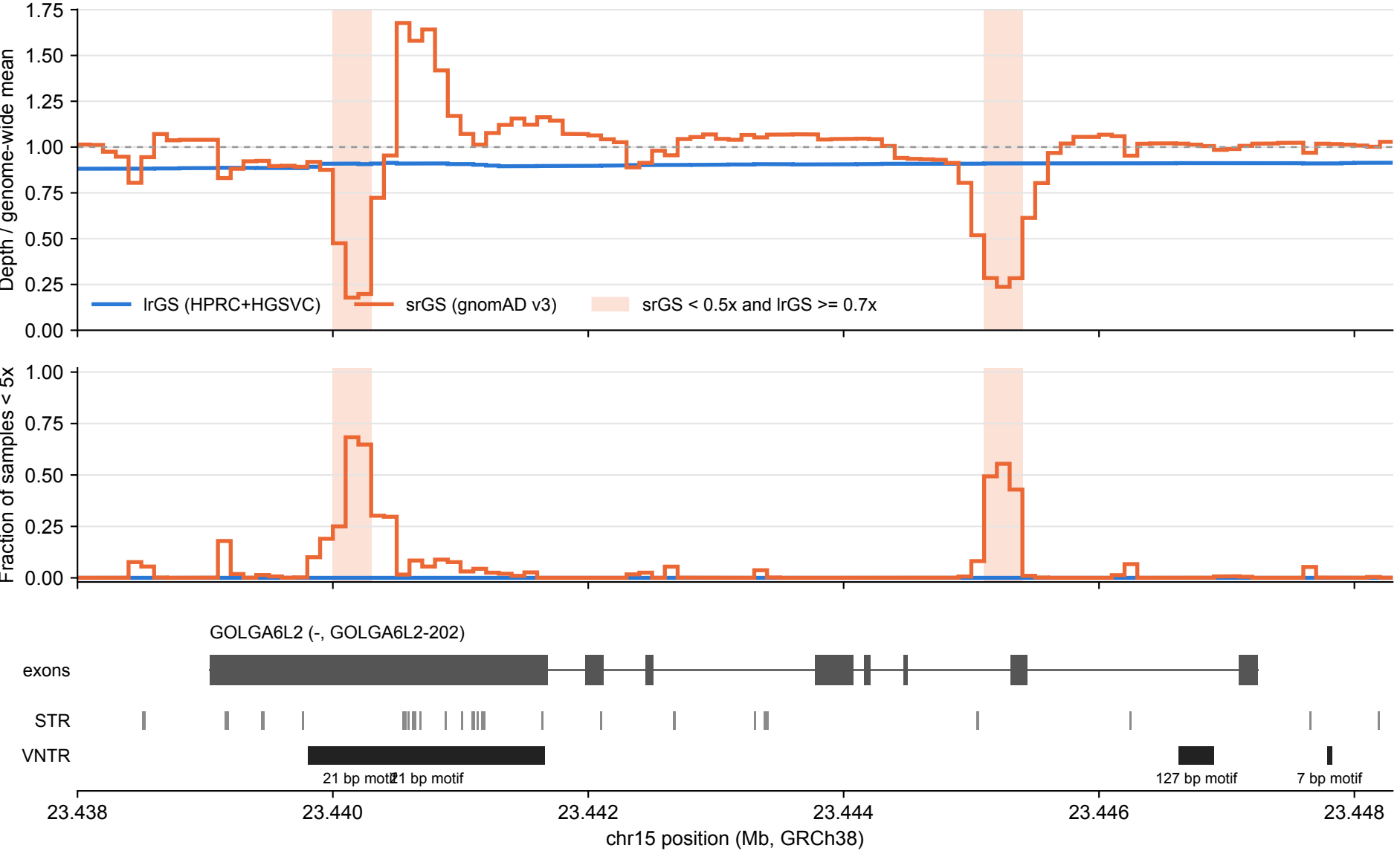
GOLGA6L2: lrGS vs srGS coverage over tandem repeats (100 bp bins)
