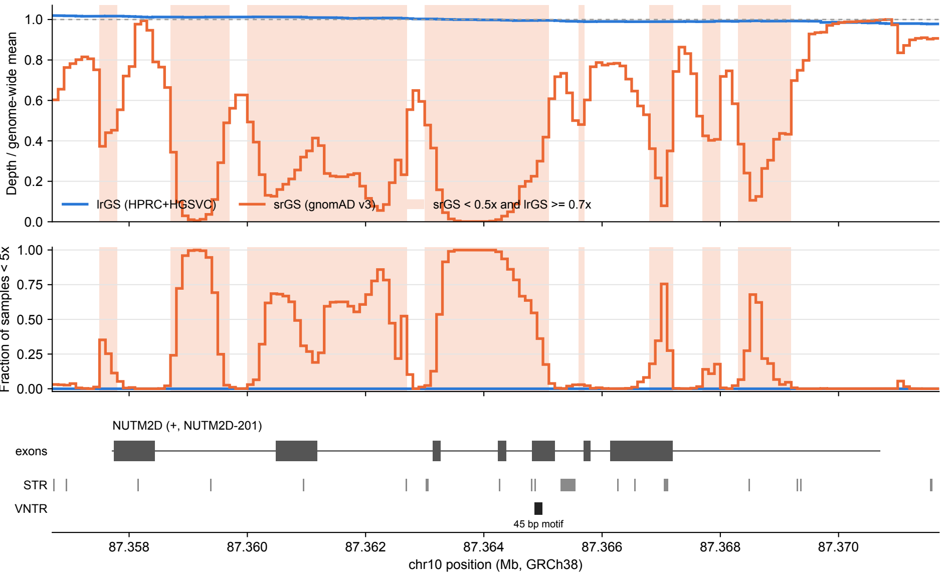
NUTM2D: lrGS vs srGS coverage over tandem repeats (100 bp bins)
