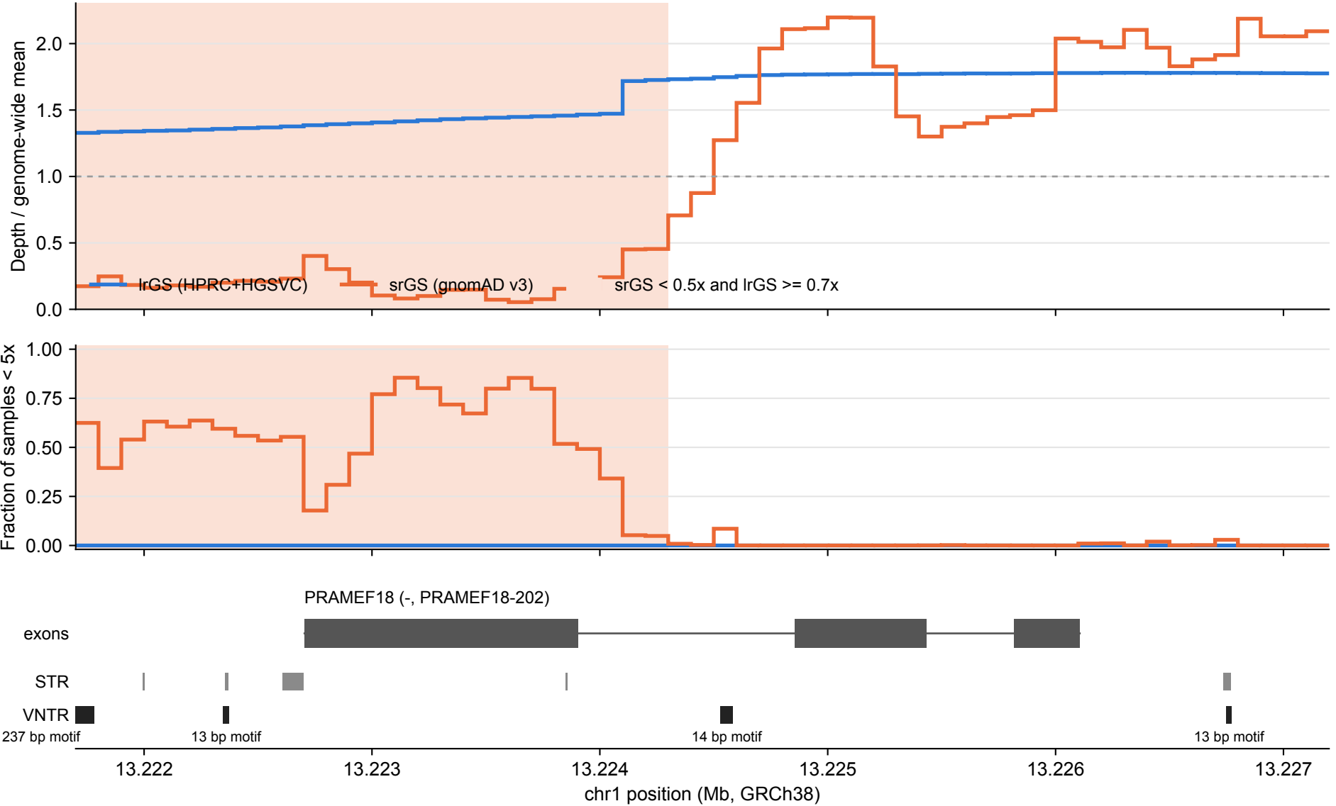
PRAMEF18: lrGS vs srGS coverage over tandem repeats (100 bp bins)
