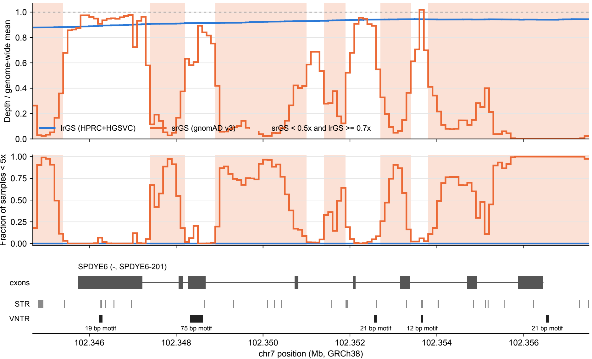
SPDYE6: lrGS vs srGS coverage over tandem repeats (100 bp bins)
