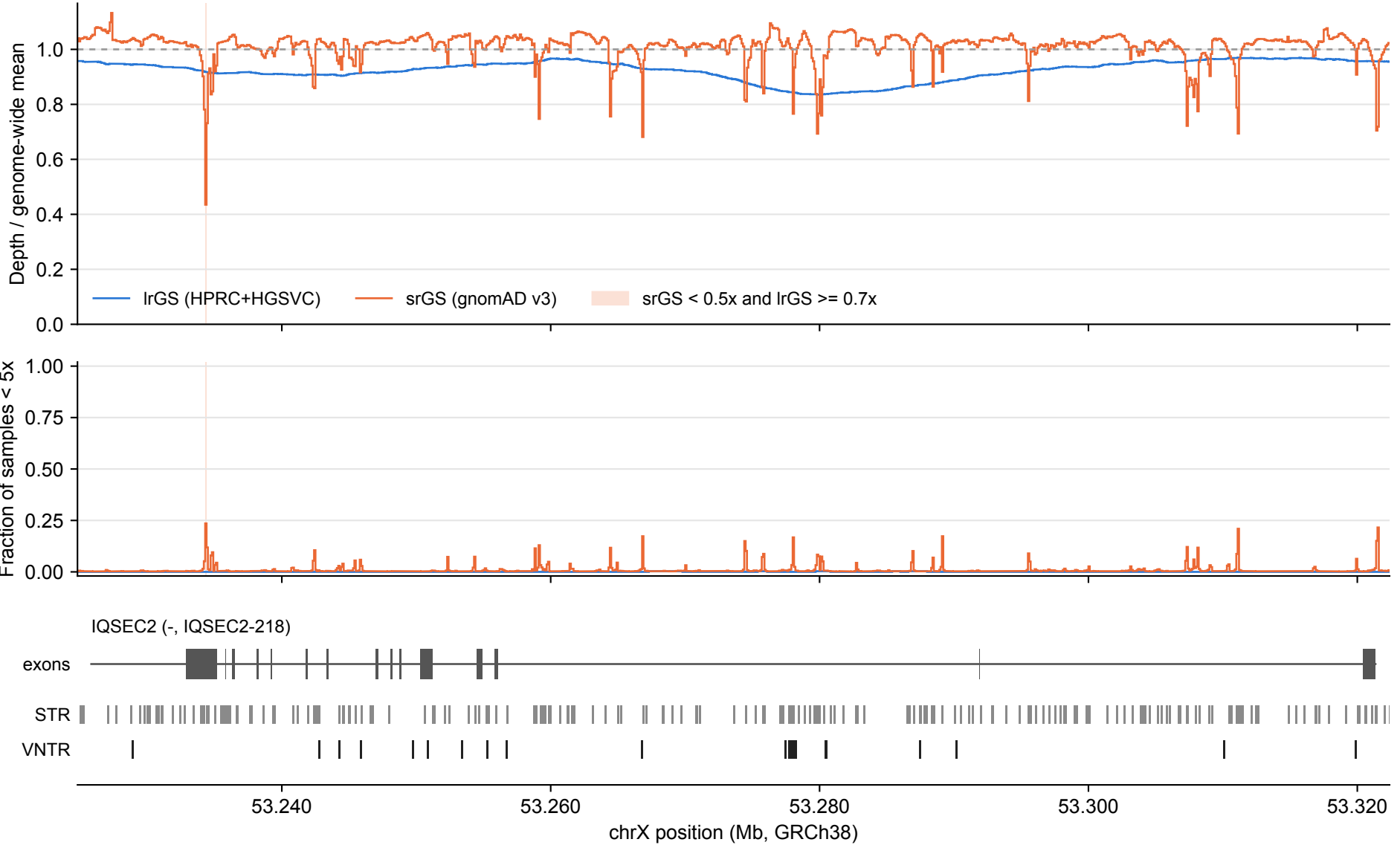
IQSEC2: IrGS vs srGS coverage over tandem repeats (100 bp bins)
