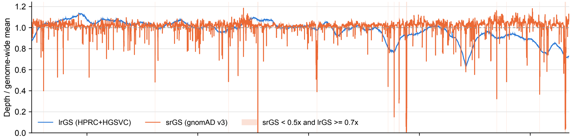
SDK1: IrGS vs srGS coverage over tandem repeats (100 bp bins)
