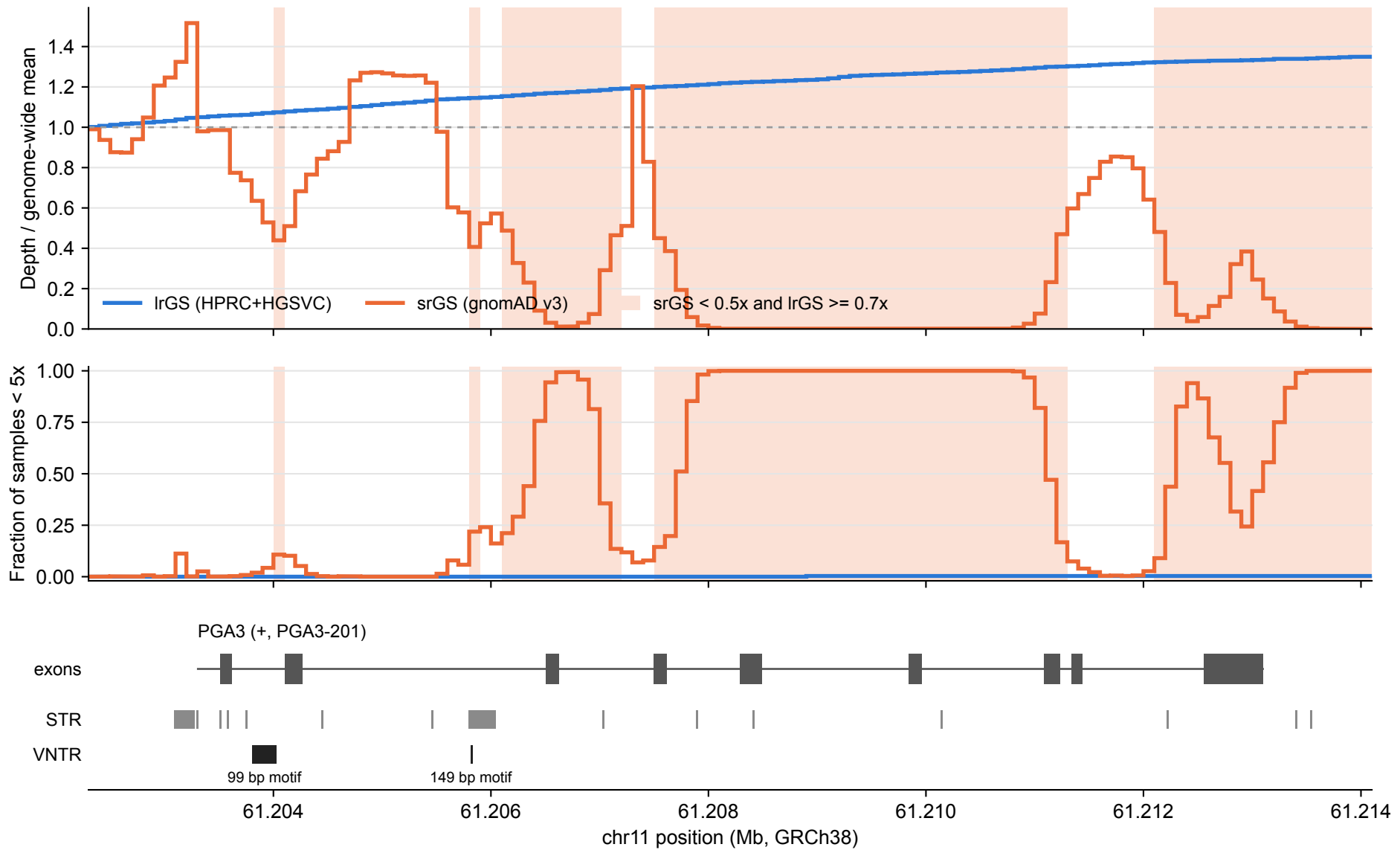
PGA3: IrGS vs srGS coverage over tandem repeats (100 bp bins)
