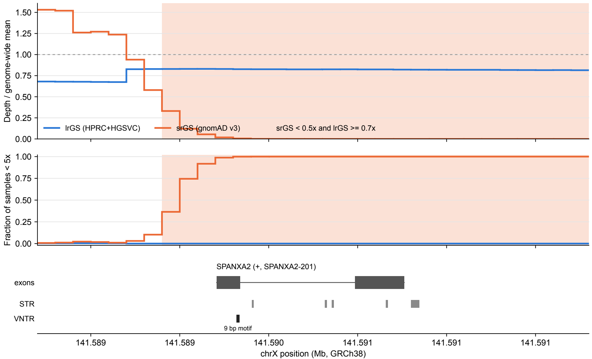
SPANXA2: lrGS vs srGS coverage over tandem repeats (100 bp bins)
