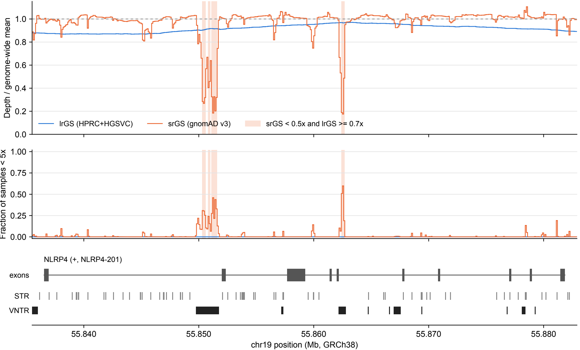
NLRP4: lrGS vs srGS coverage over tandem repeats (100 bp bins)
