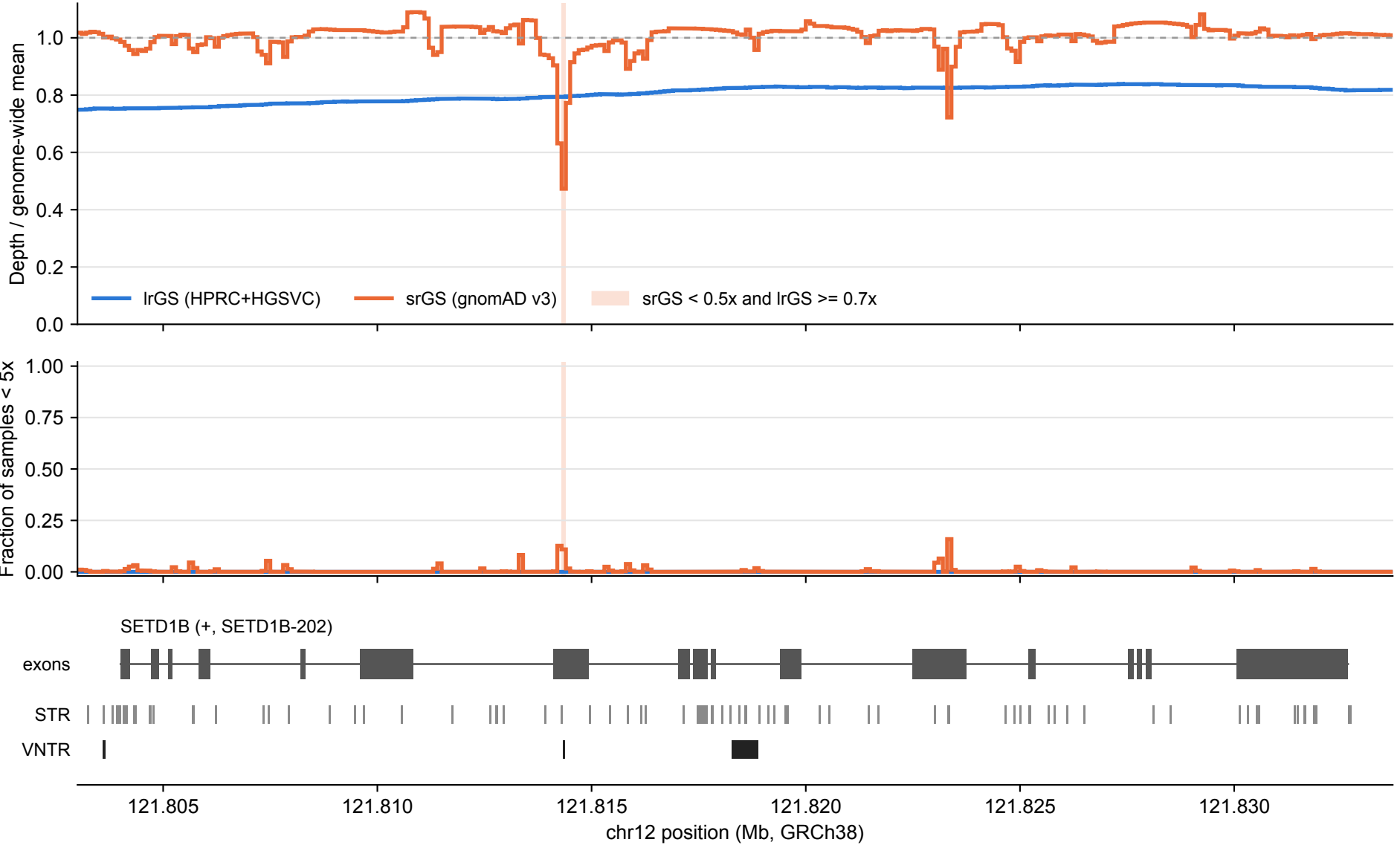
SETD1B: lrGS vs srGS coverage over tandem repeats (100 bp bins)
