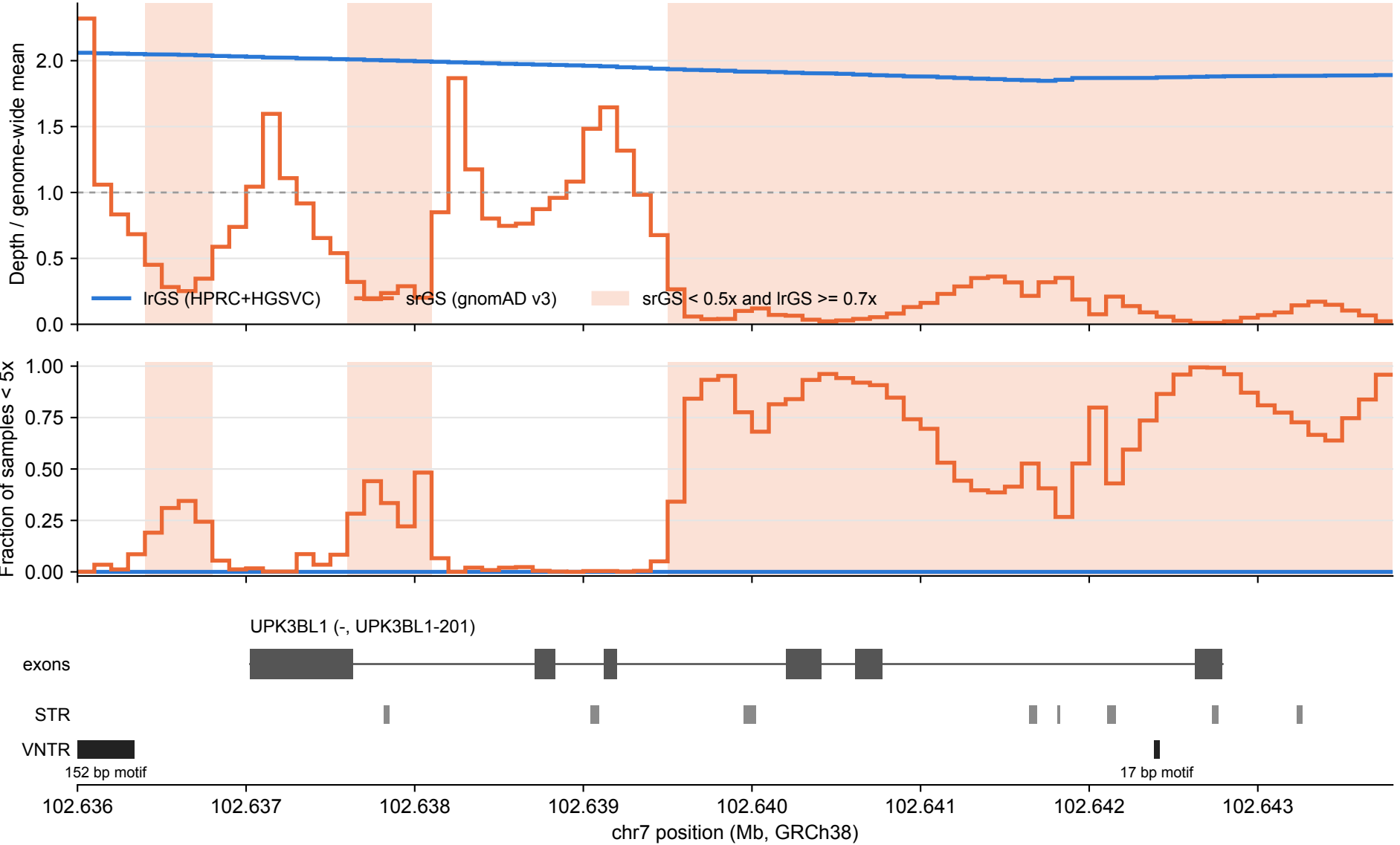
UPK3BL1: lrGS vs srGS coverage over tandem repeats (100 bp bins)
