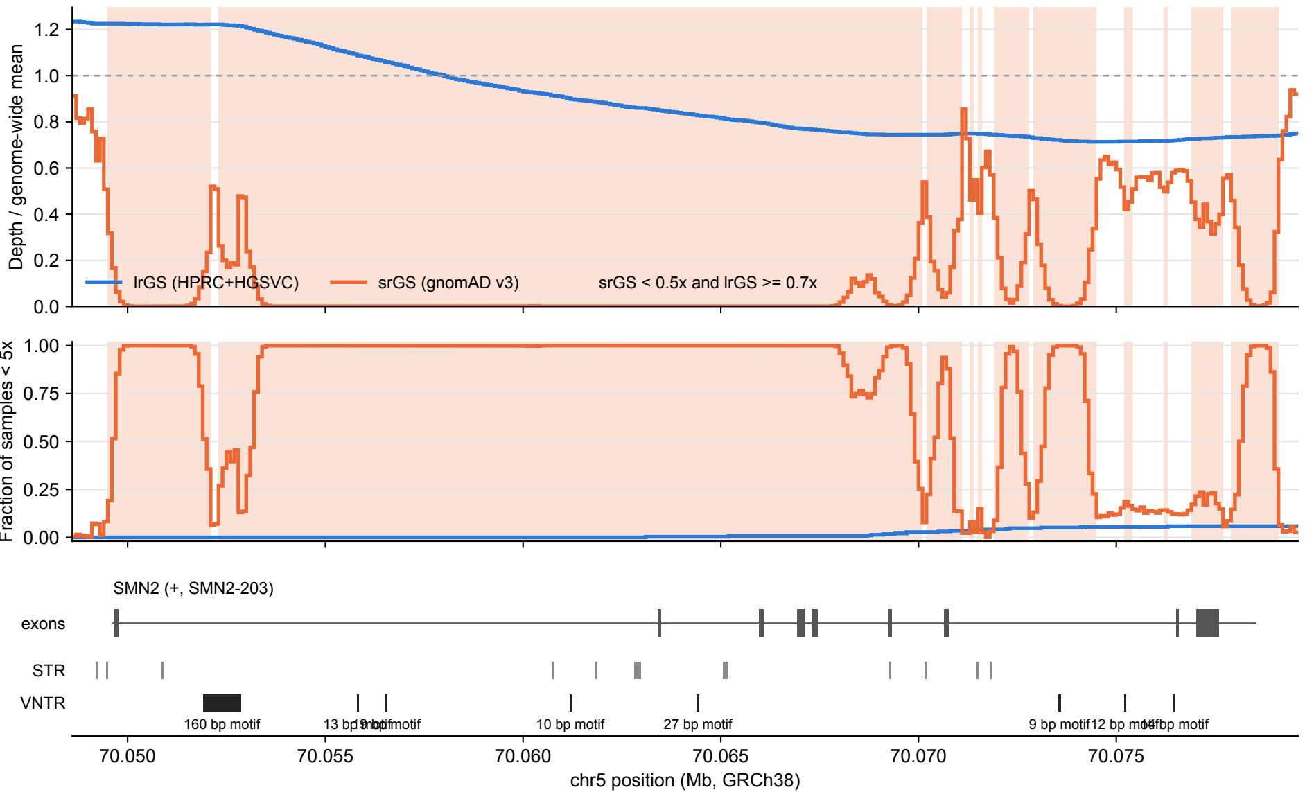
SMN2: lrGS vs srGS coverage over tandem repeats (100 bp bins)
