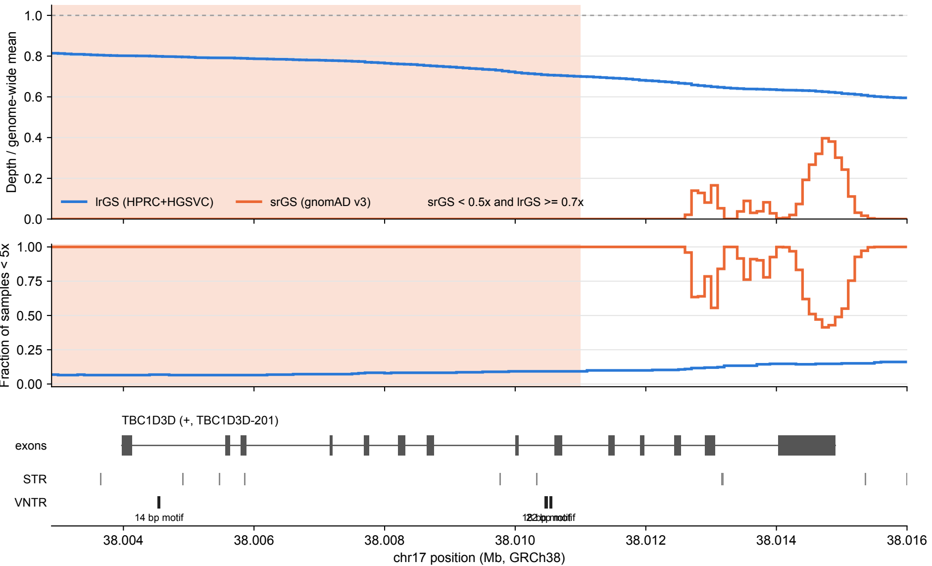
TBC1D3D: lrGS vs srGS coverage over tandem repeats (100 bp bins)
