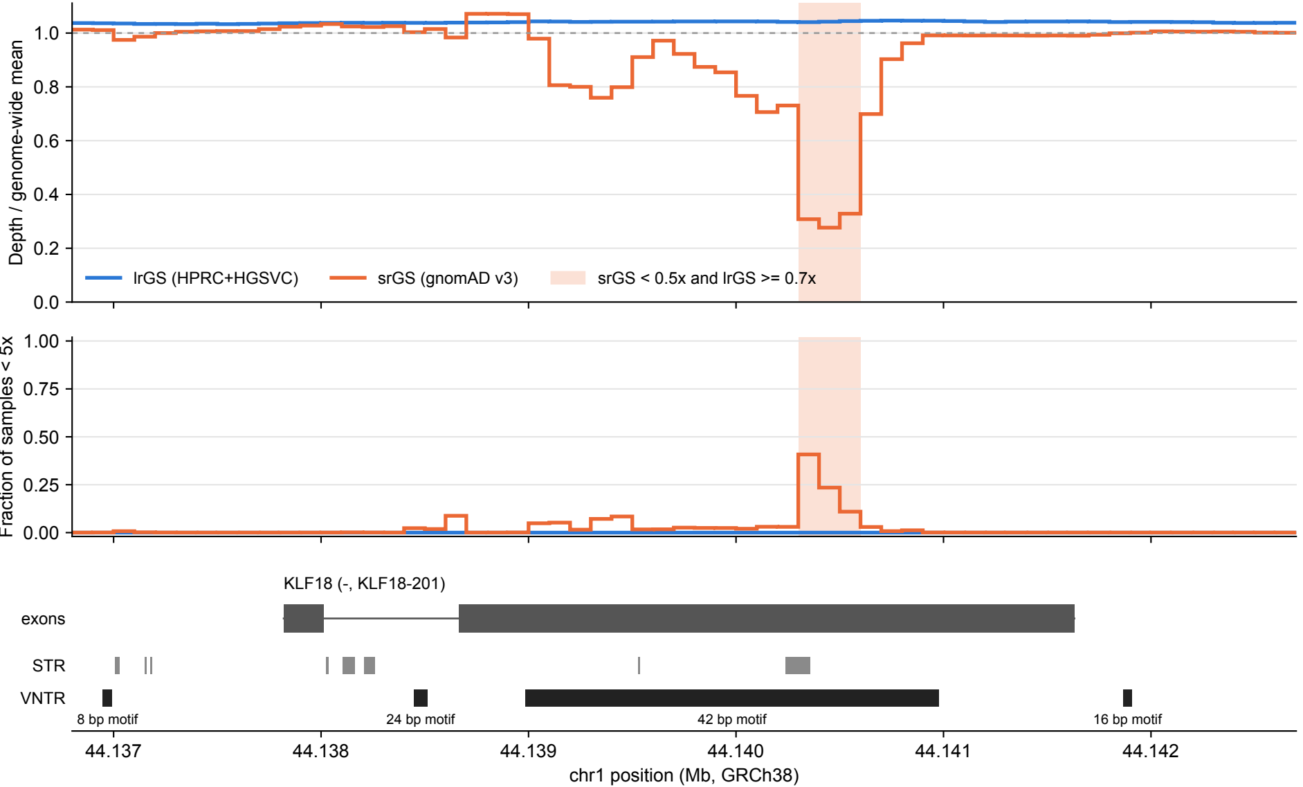
KLF18: lrGS vs srGS coverage over tandem repeats (100 bp bins)
