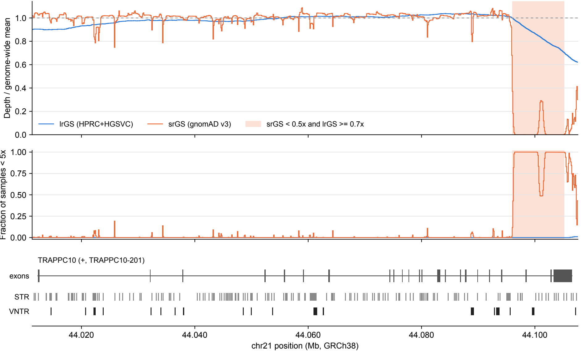
TRAPPC10: lrGS vs srGS coverage over tandem repeats (100 bp bins)
