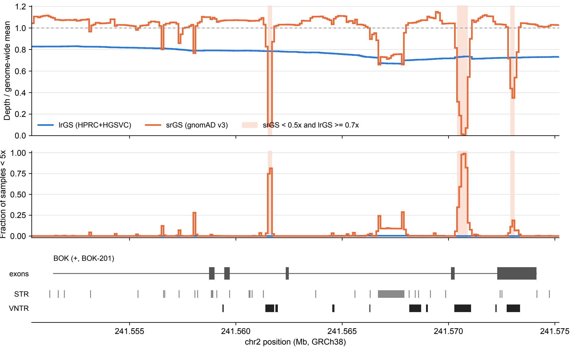
BOK: IrGS vs srGS coverage over tandem repeats (100 bp bins)
