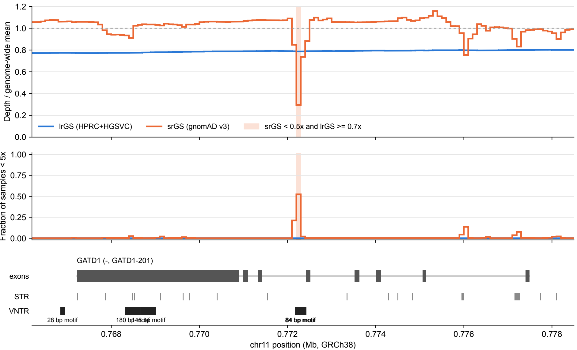
GATD1: IrGS vs srGS coverage over tandem repeats (100 bp bins)
