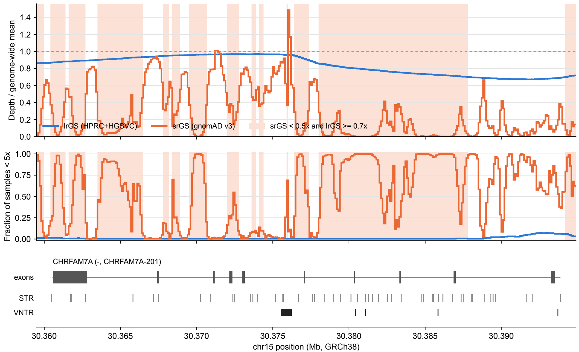
CHRFAM7A: lrGS vs srGS coverage over tandem repeats (100 bp bins)
