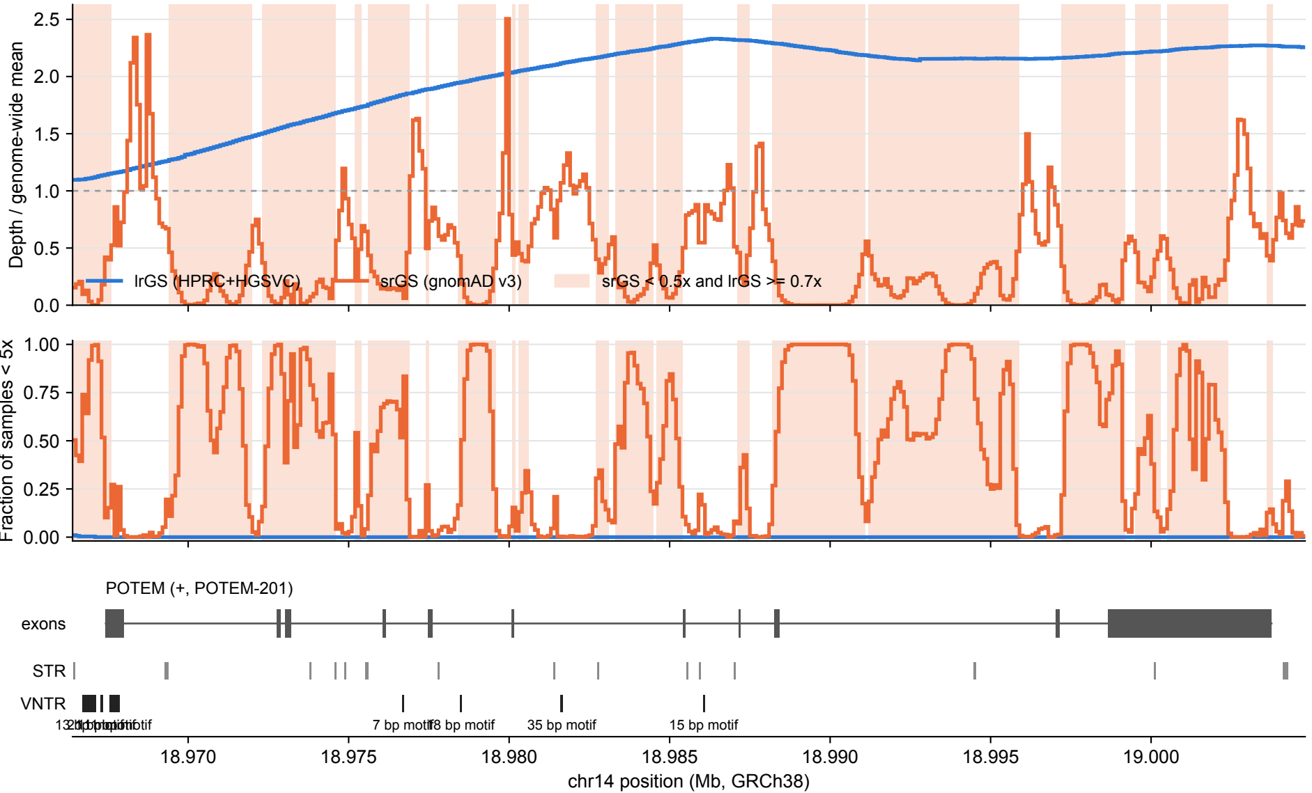
POTEM: IrGS vs srGS coverage over tandem repeats (100 bp bins)
