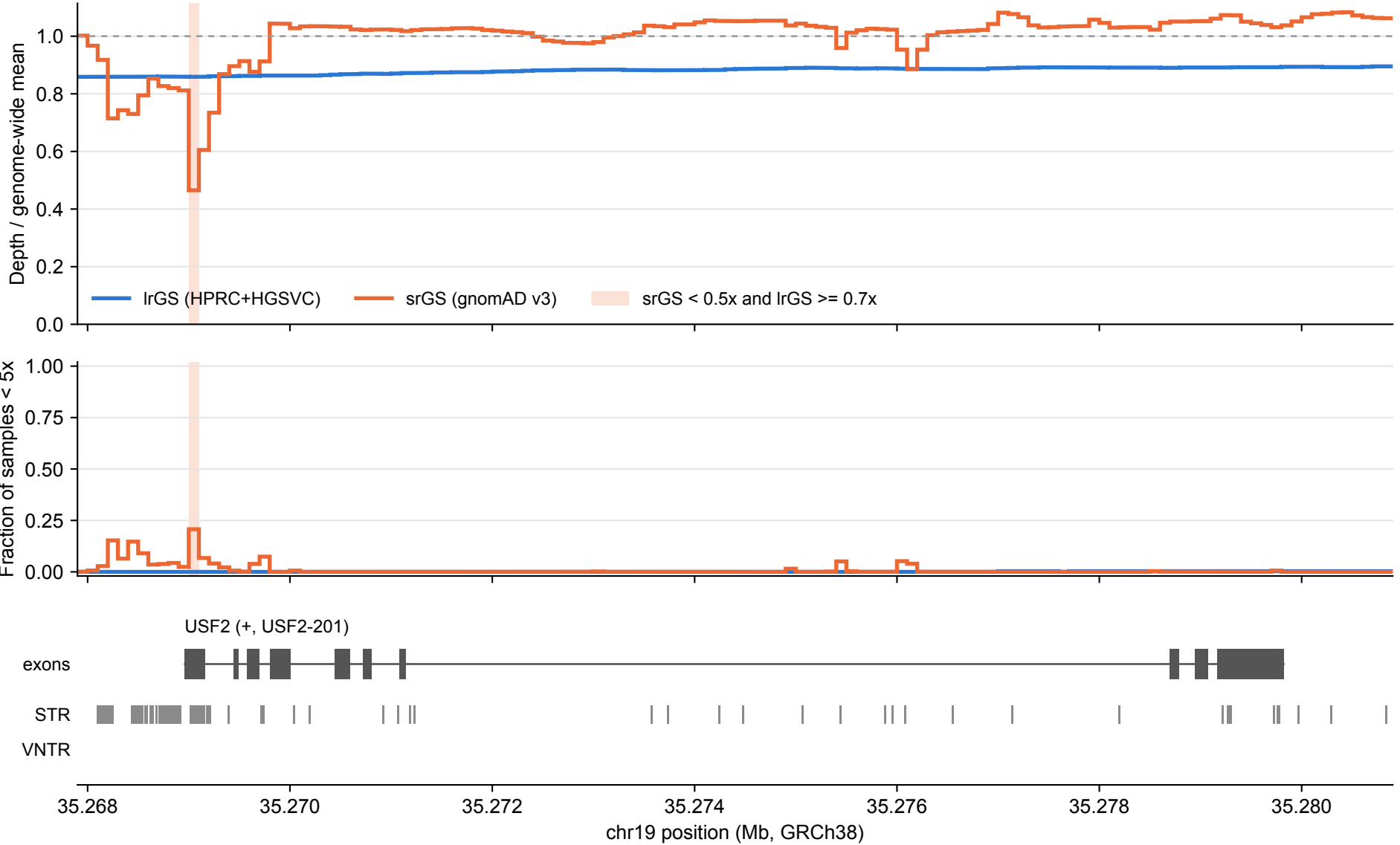
USF2: lrGS vs srGS coverage over tandem repeats (100 bp bins)
