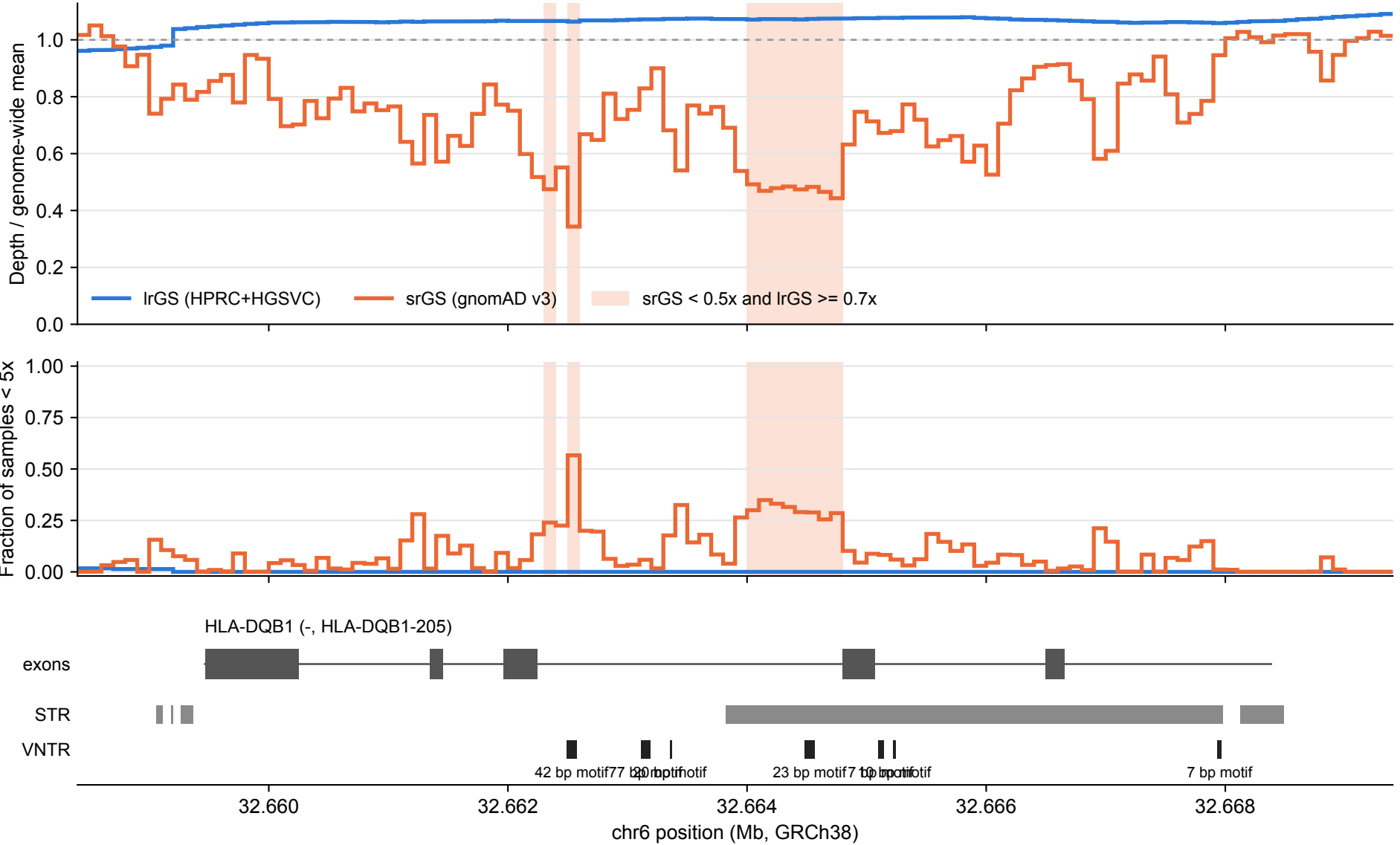
HLA-DQB1: lrGS vs srGS coverage over tandem repeats (100 bp bins)
