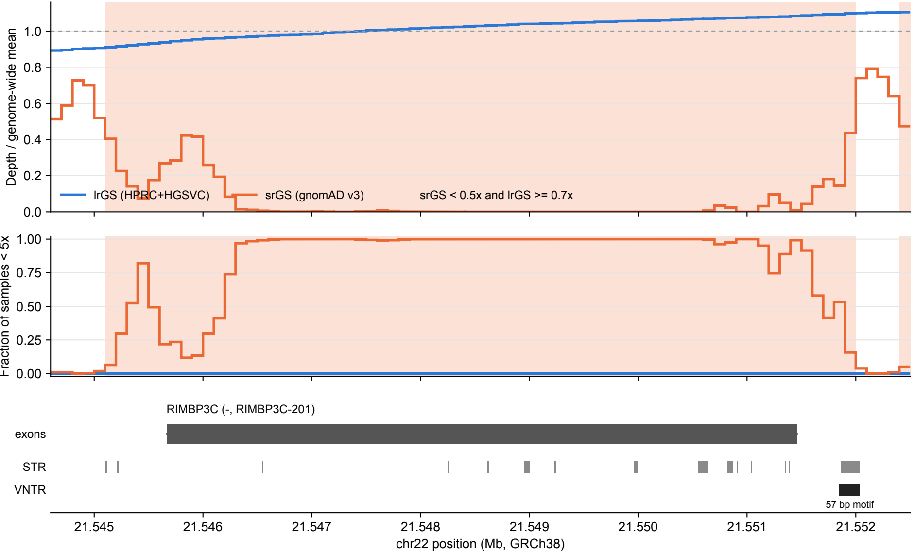
RIMBP3C: lrGS vs srGS coverage over tandem repeats (100 bp bins)
