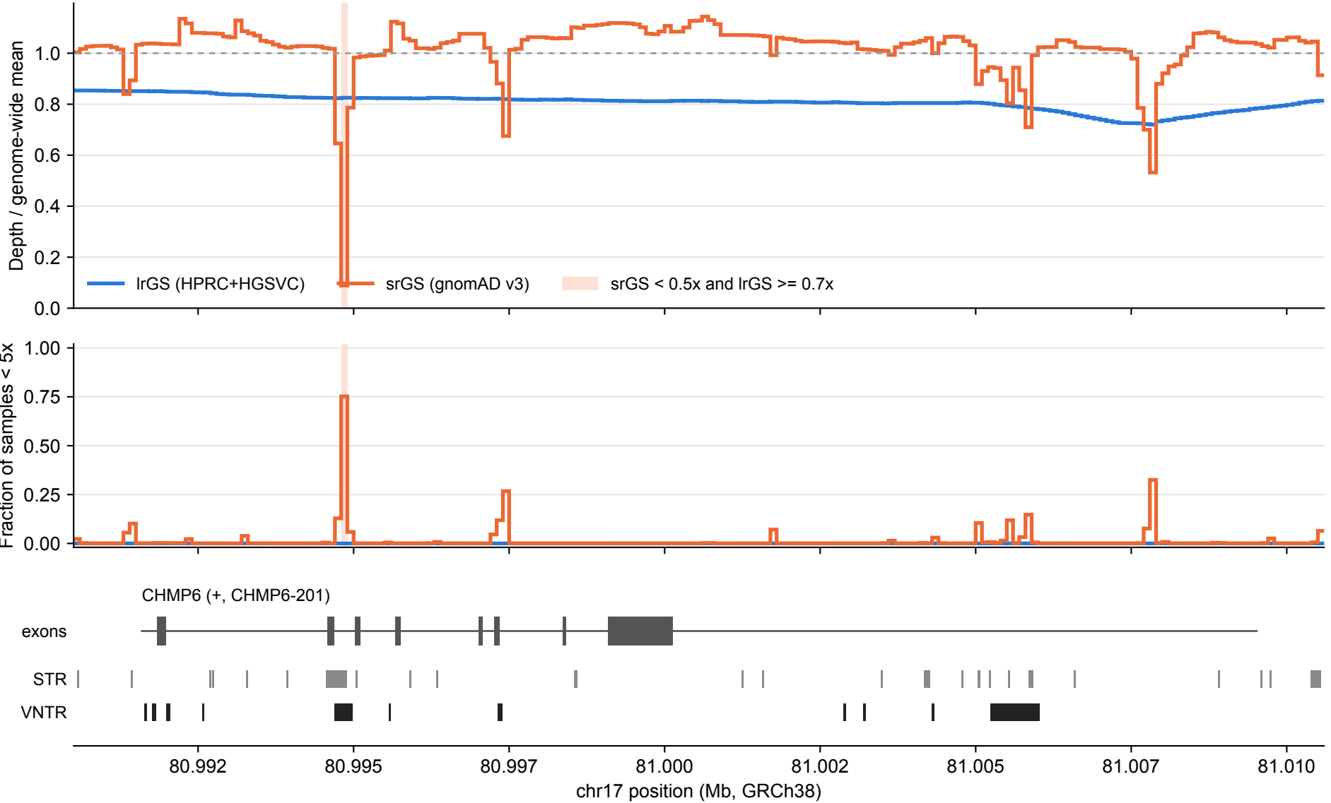
CHMP6: lrGS vs srGS coverage over tandem repeats (100 bp bins)
