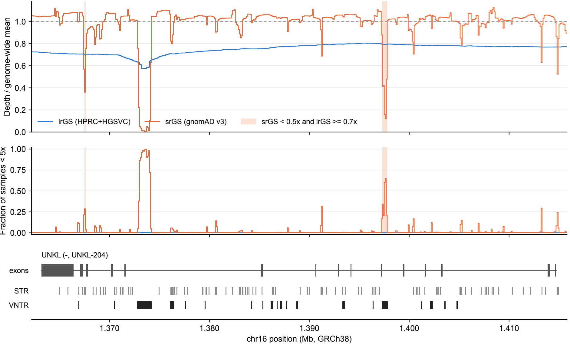
UNKL: lrGS vs srGS coverage over tandem repeats (100 bp bins)
