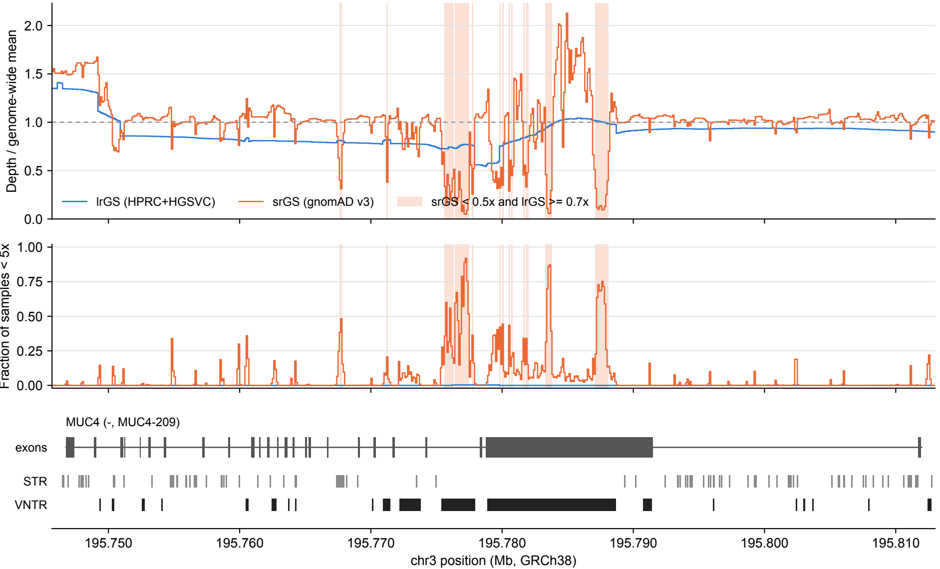
MUC4: IrGS vs srGS coverage over tandem repeats (100 bp bins)
