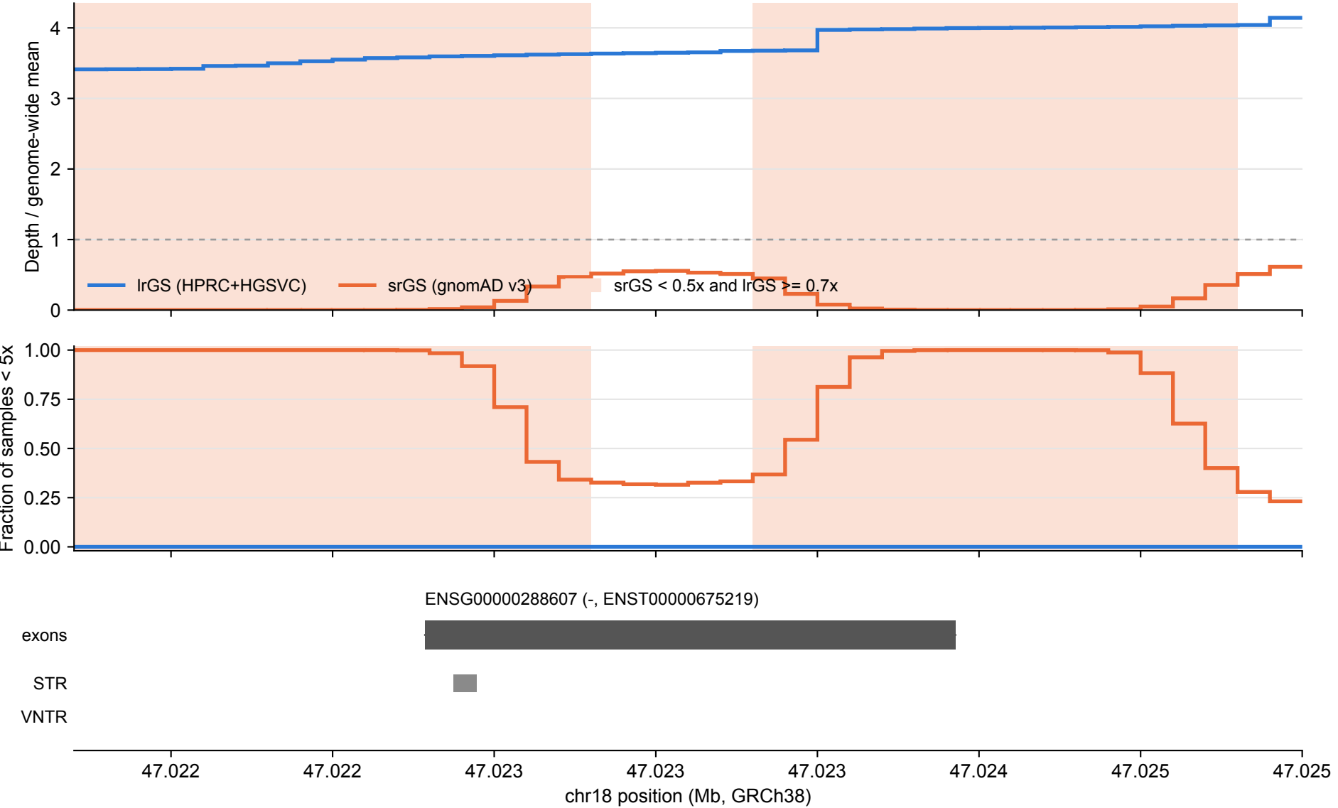
ENSG00000288607: lrGS vs srGS coverage over tandem repeats (100 bp bins)
