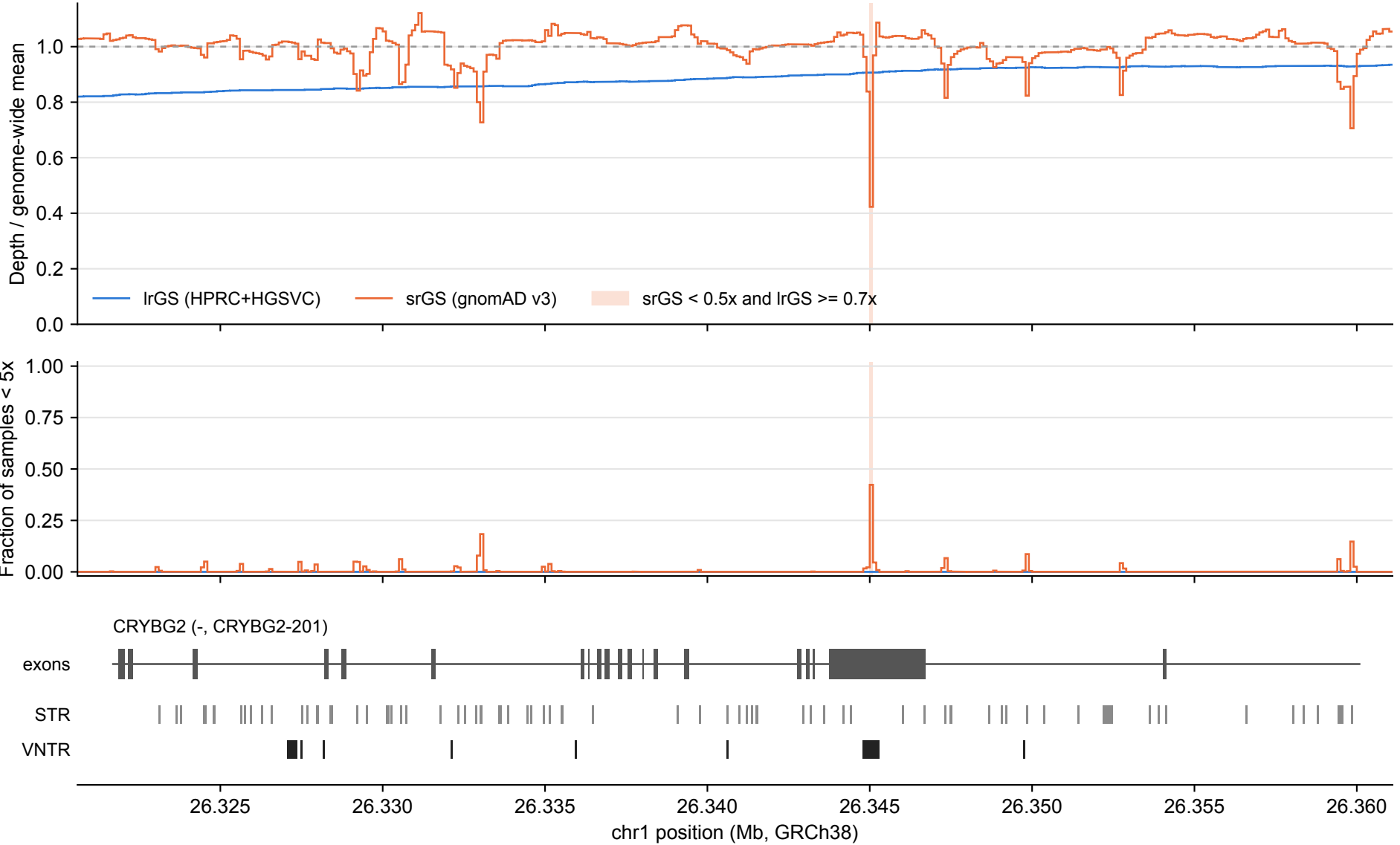
CRYBG2: lrGS vs srGS coverage over tandem repeats (100 bp bins)
