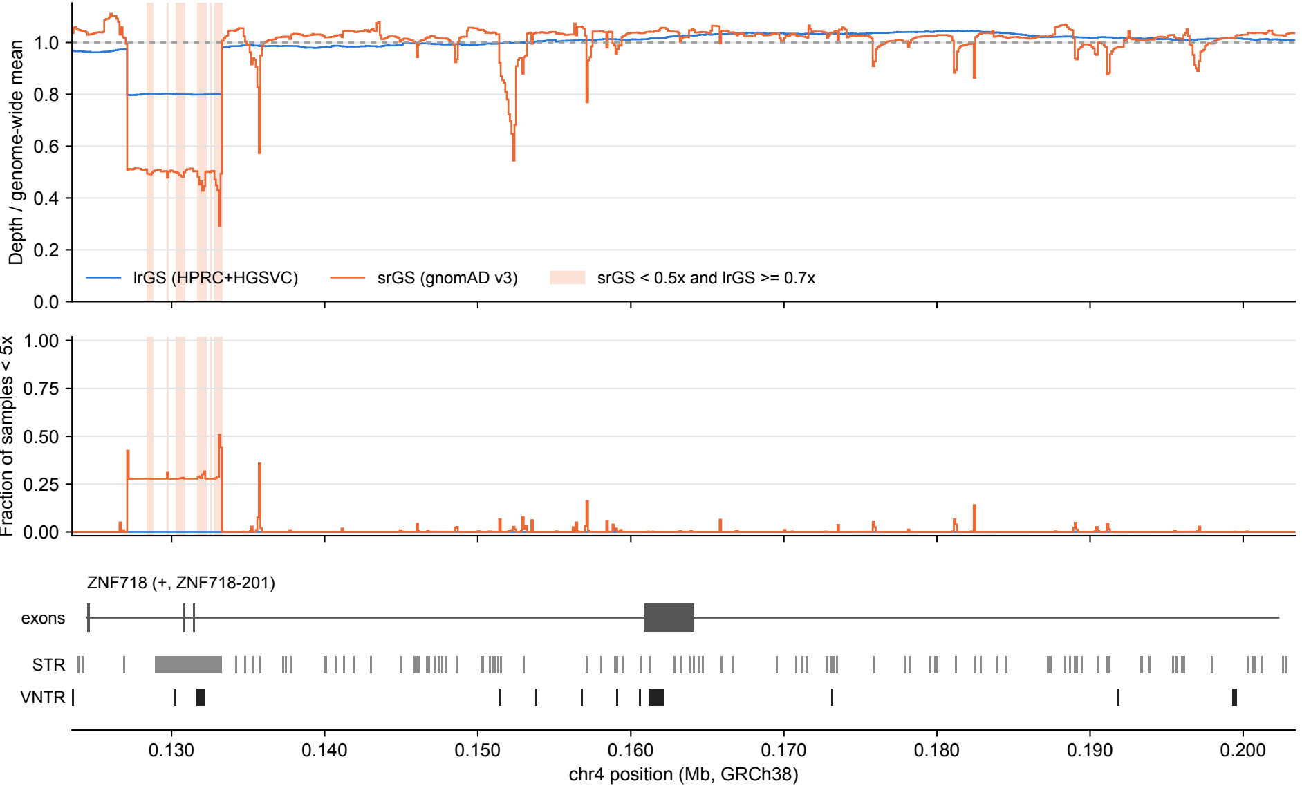
ZNF718: lrGS vs srGS coverage over tandem repeats (100 bp bins)
