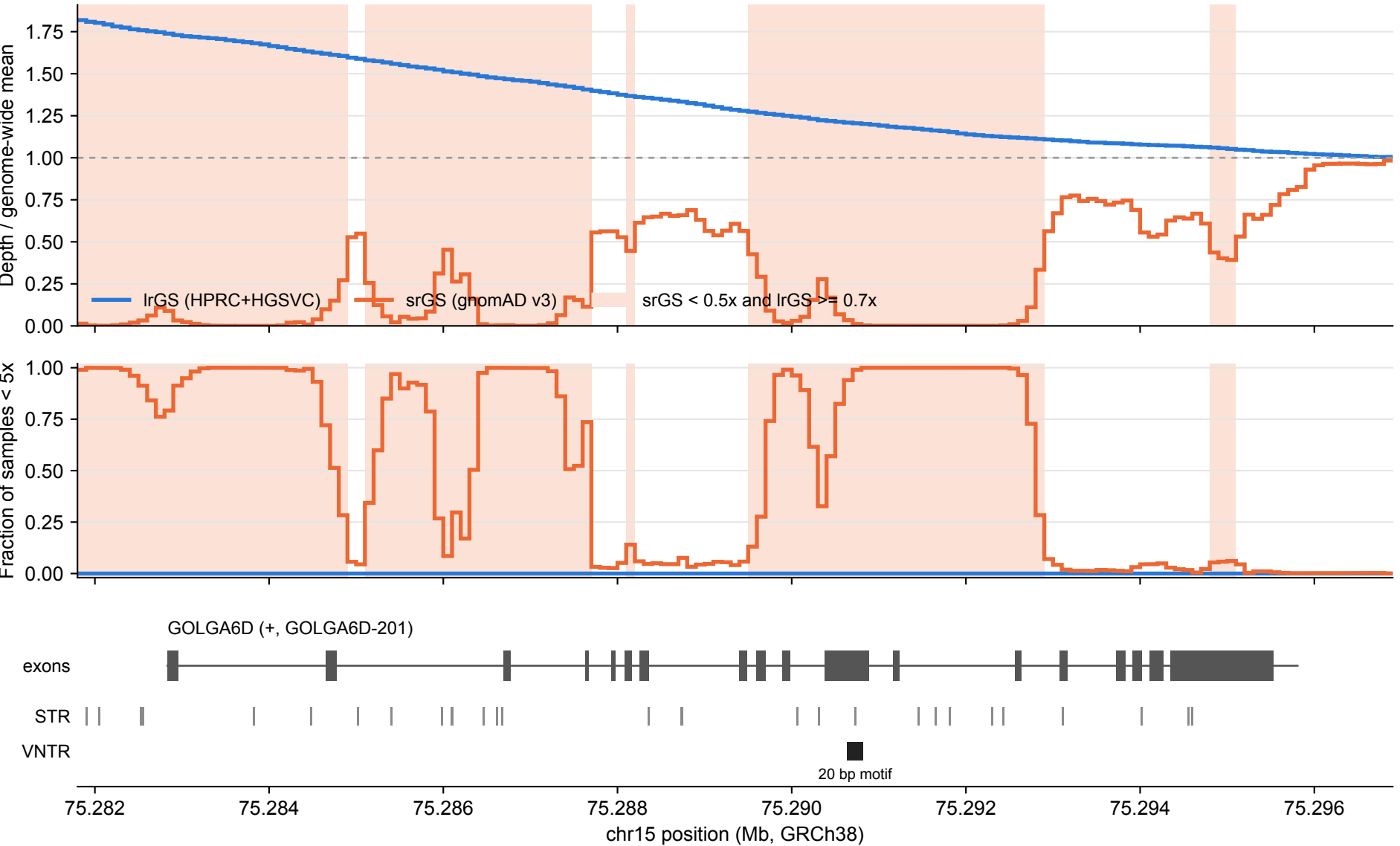
GOLGA6D: lrGS vs srGS coverage over tandem repeats (100 bp bins)
