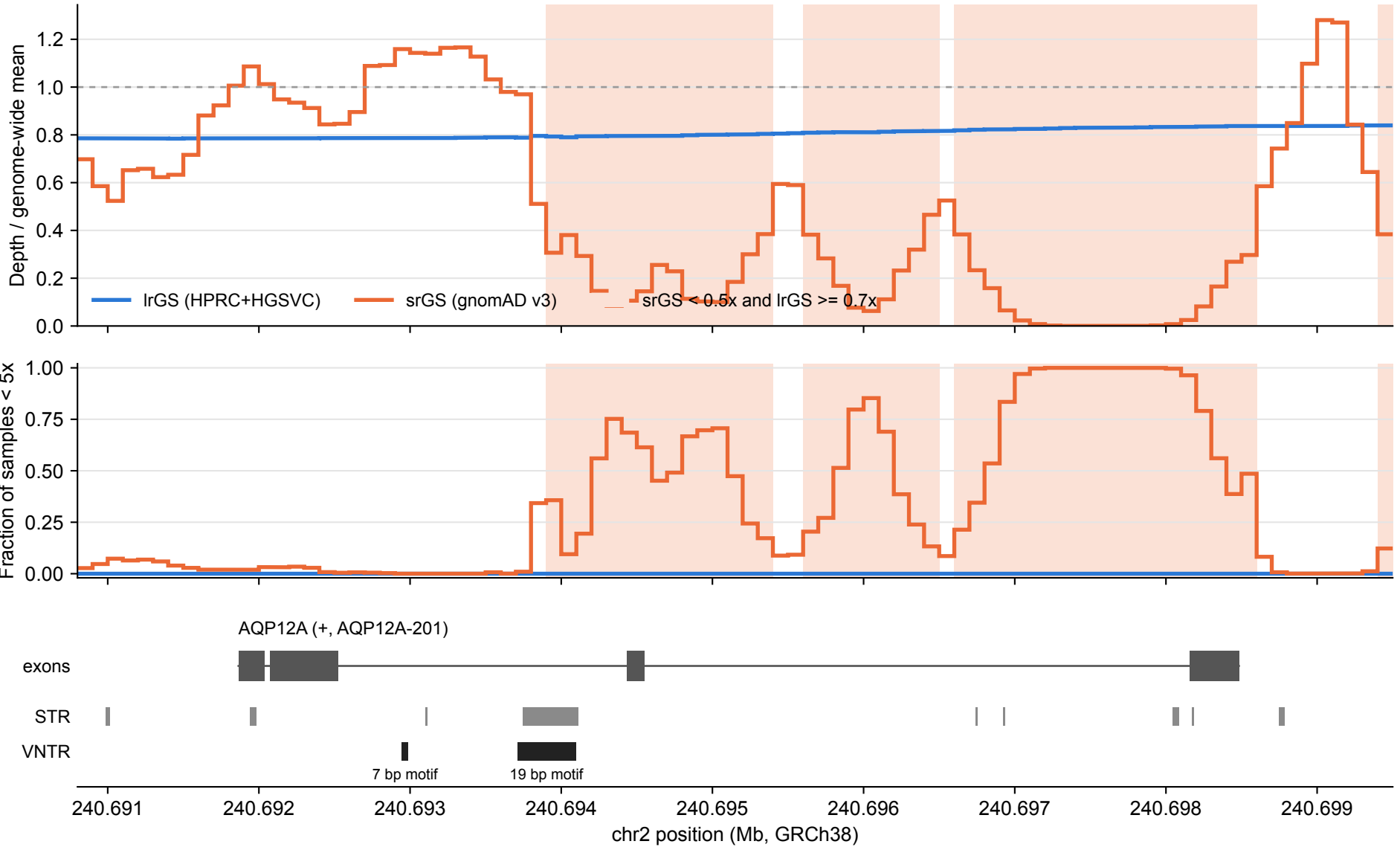
AQP12A: lrGS vs srGS coverage over tandem repeats (100 bp bins)
