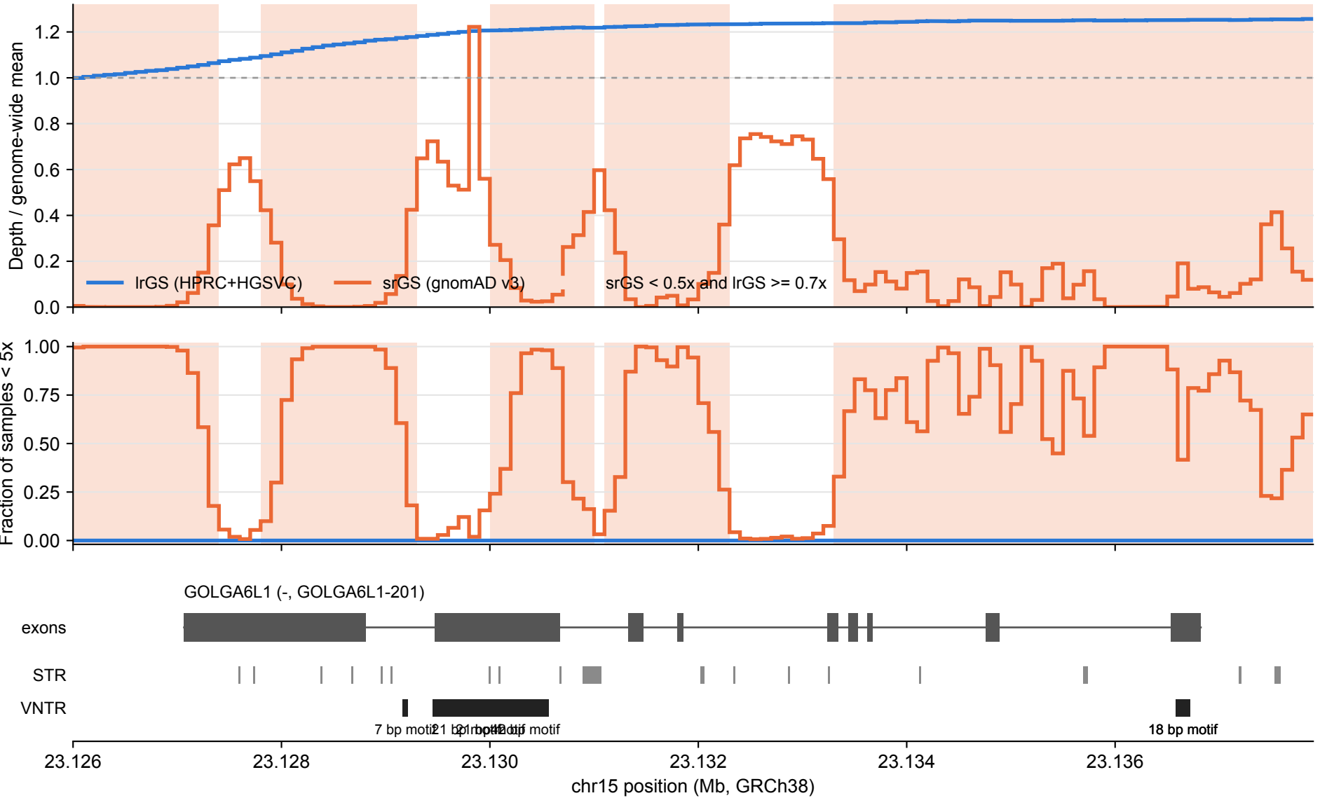
GOLGA6L1: lrGS vs srGS coverage over tandem repeats (100 bp bins)
