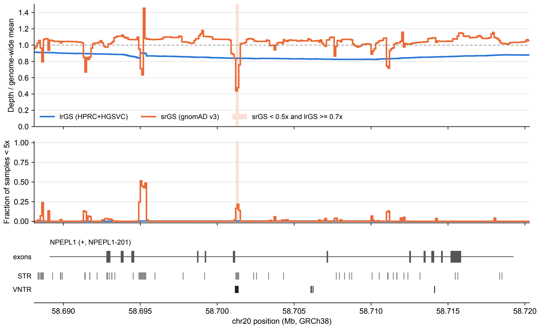
NPEPL1: lrGS vs srGS coverage over tandem repeats (100 bp bins)
