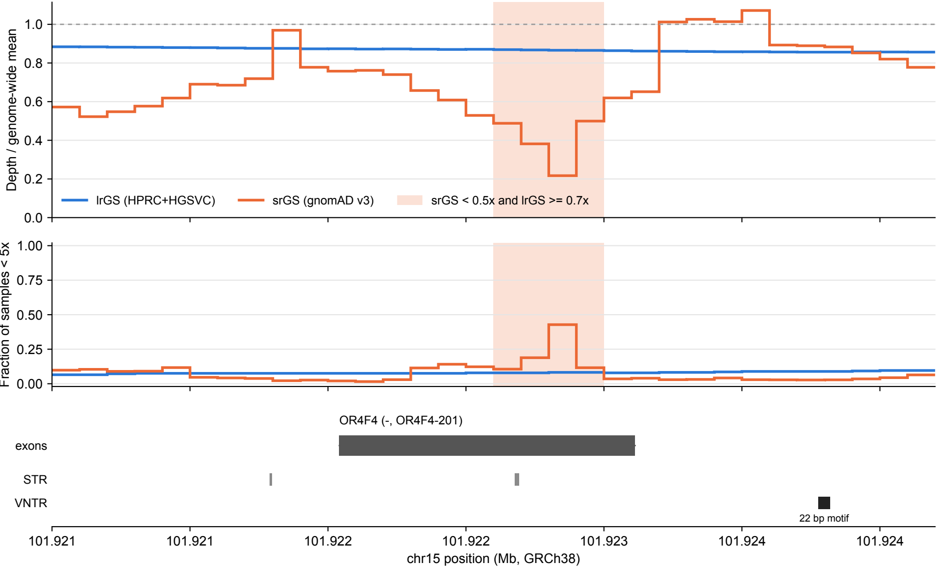
OR4F4: lrGS vs srGS coverage over tandem repeats (100 bp bins)
