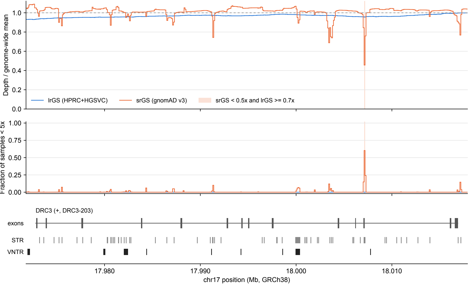
DRC3: lrGS vs srGS coverage over tandem repeats (100 bp bins)
