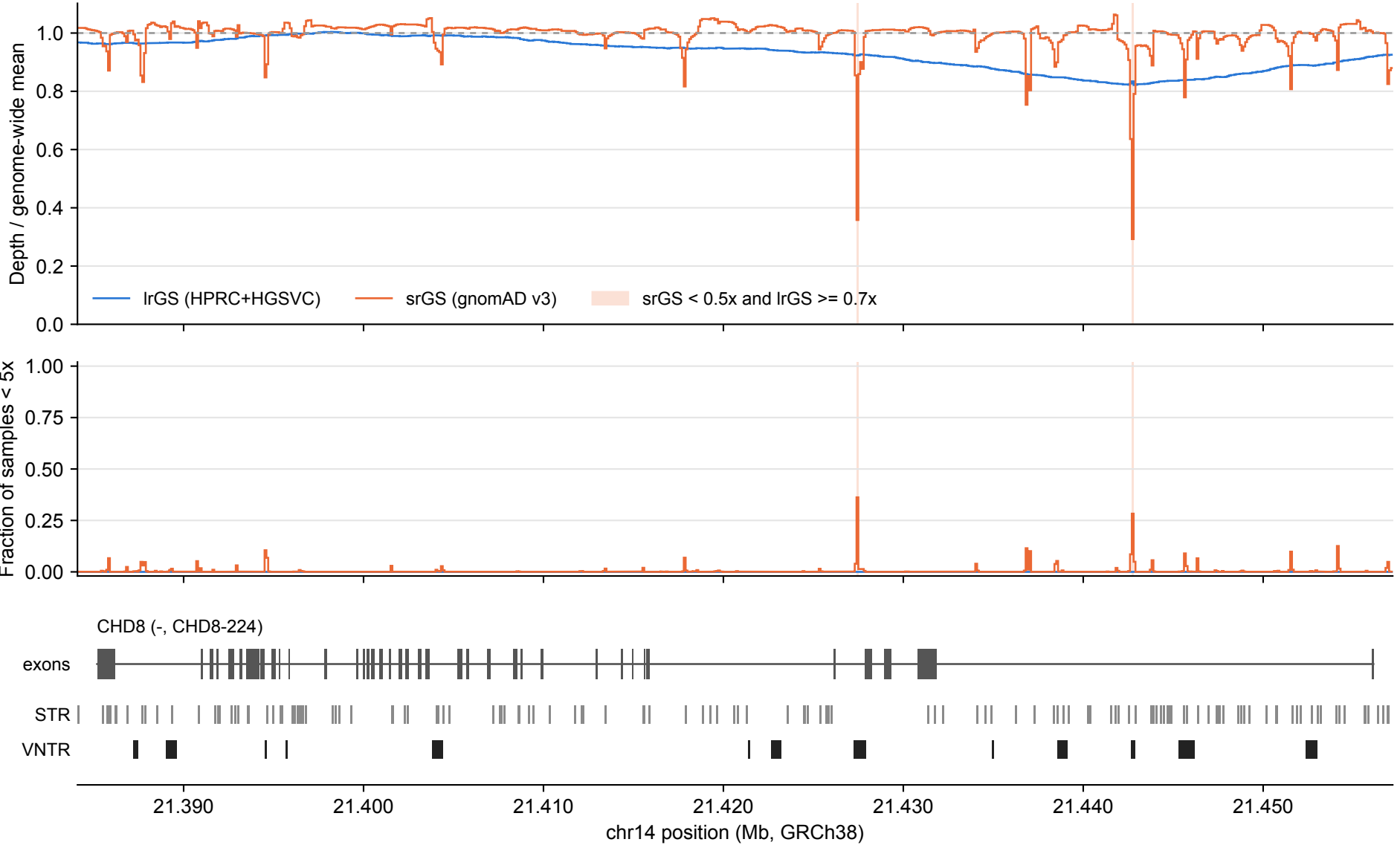
CHD8: lrGS vs srGS coverage over tandem repeats (100 bp bins)
