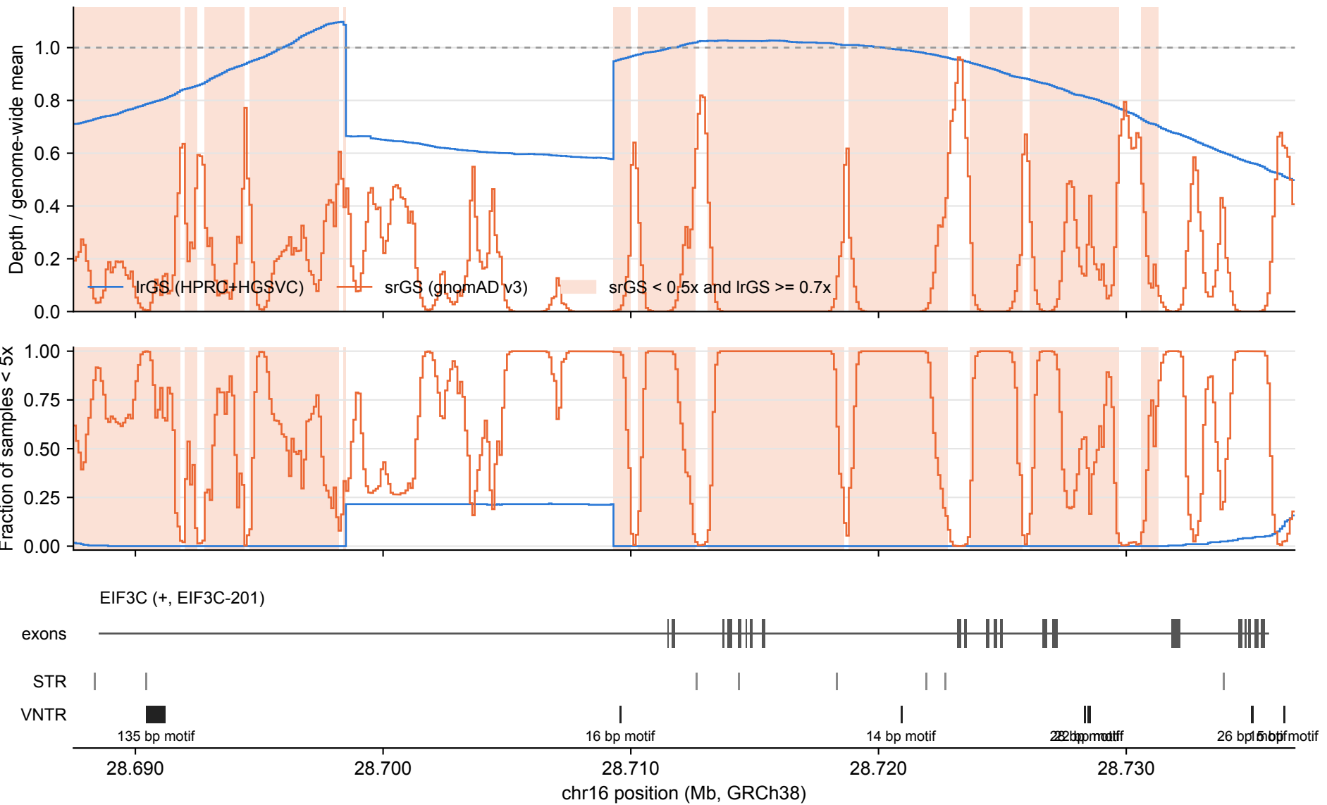
EIF3C: lrGS vs srGS coverage over tandem repeats (100 bp bins)
