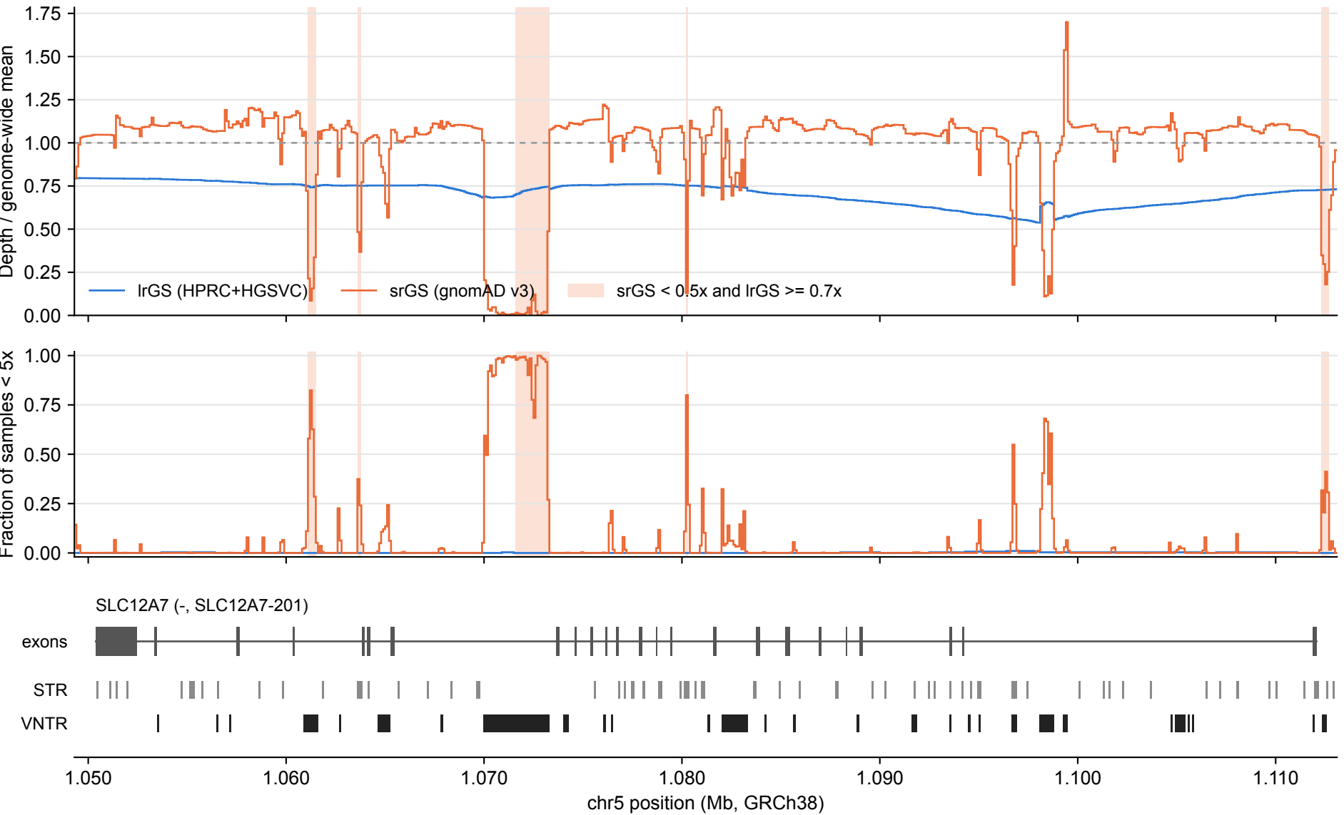
SLC12A7: lrGS vs srGS coverage over tandem repeats (100 bp bins)
