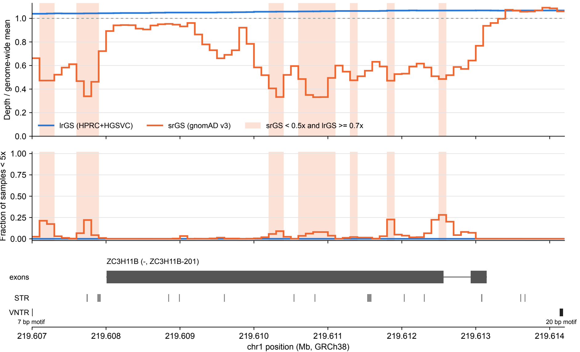
ZC3H11B: lrGS vs srGS coverage over tandem repeats (100 bp bins)
