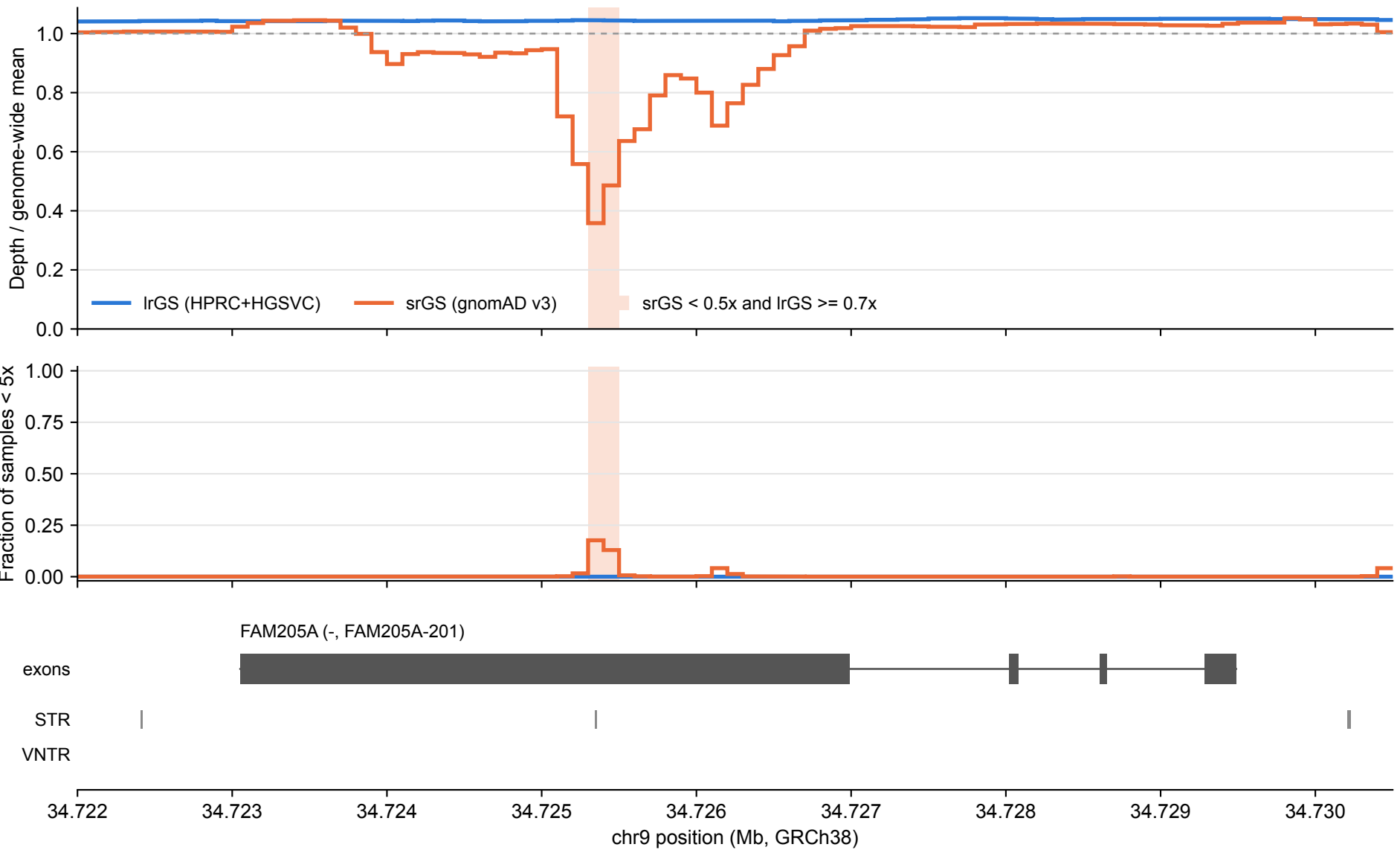
FAM205A: lrGS vs srGS coverage over tandem repeats (100 bp bins)
