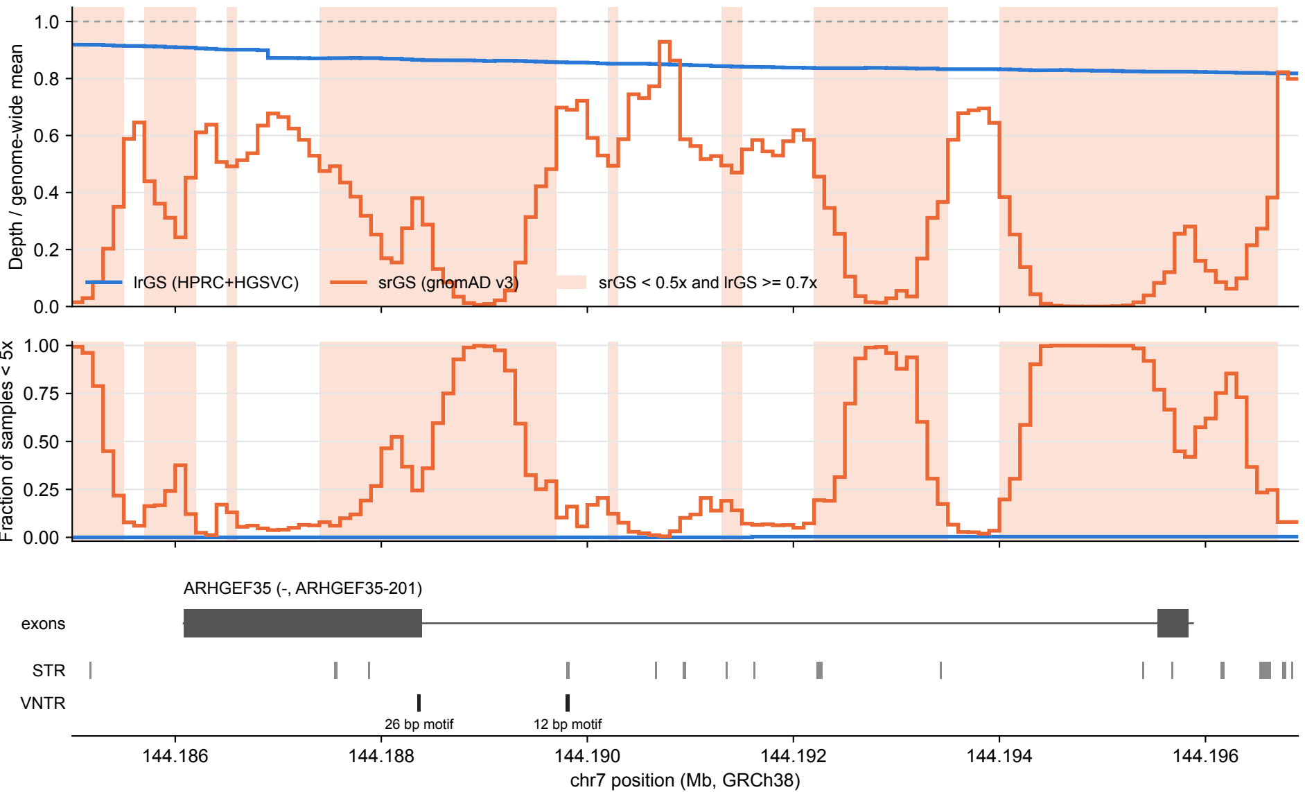
ARHGEF35: lrGS vs srGS coverage over tandem repeats (100 bp bins)
