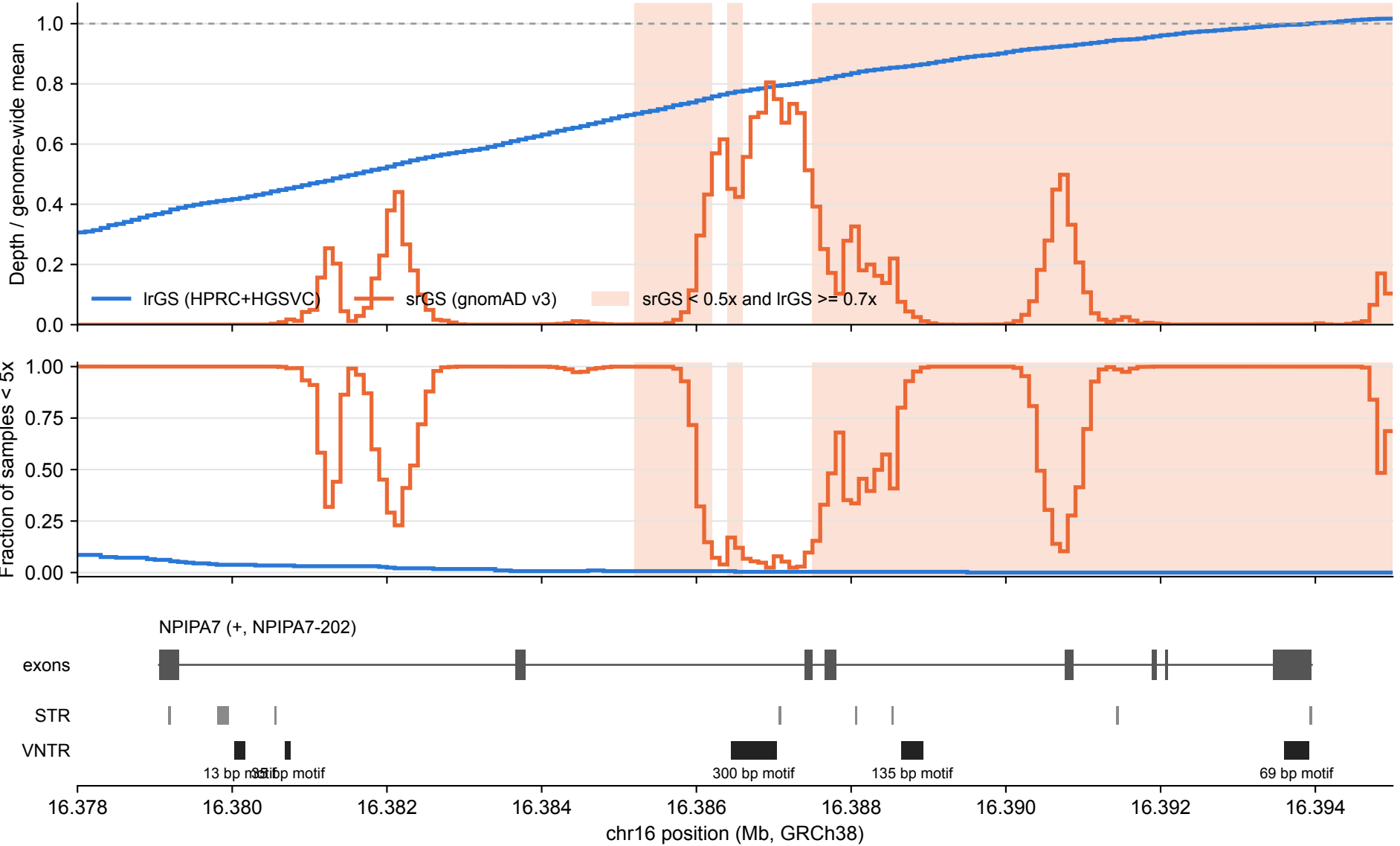
NPIPA7: IrGS vs srGS coverage over tandem repeats (100 bp bins)
