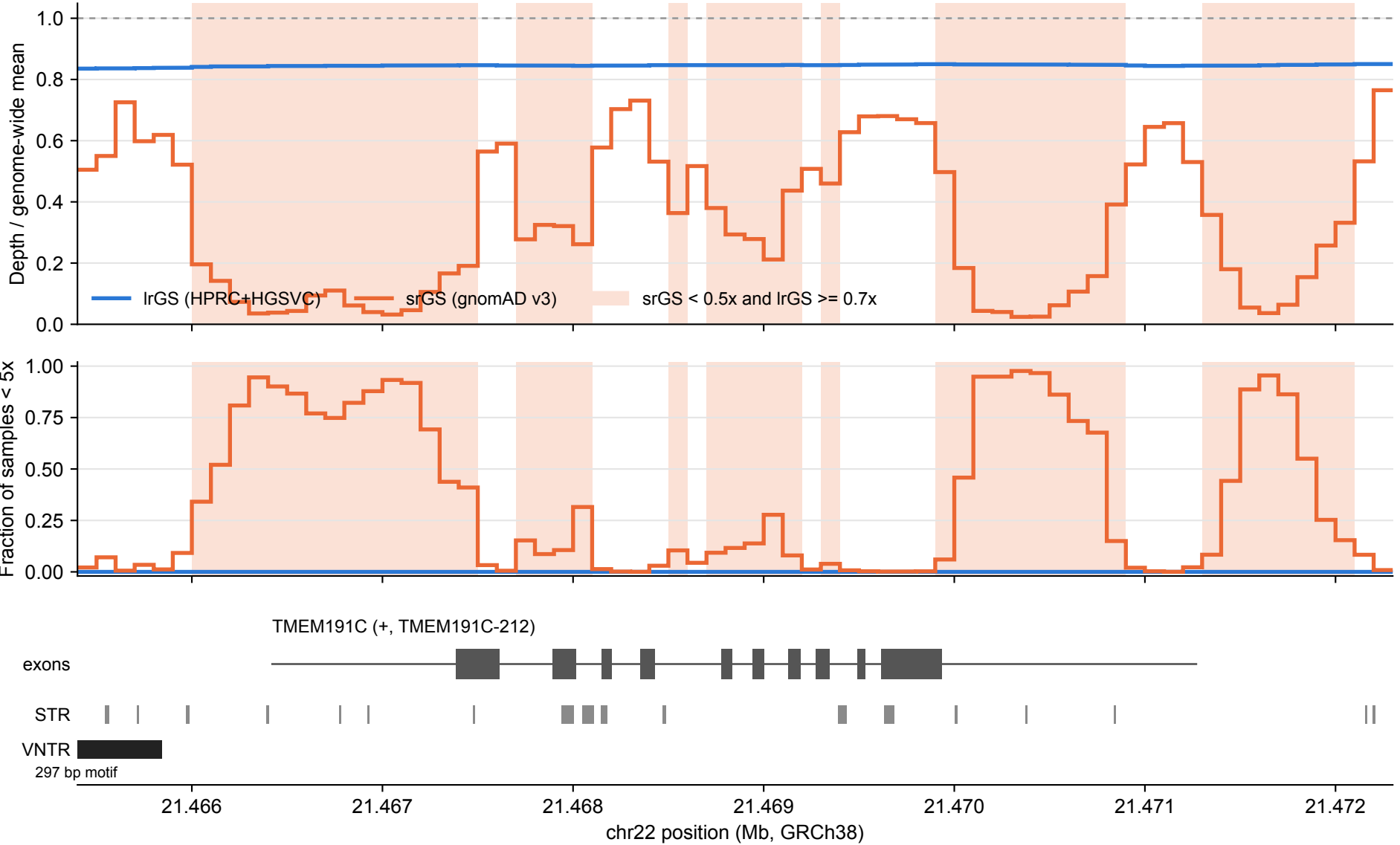
TMEM191C: lrGS vs srGS coverage over tandem repeats (100 bp bins)
