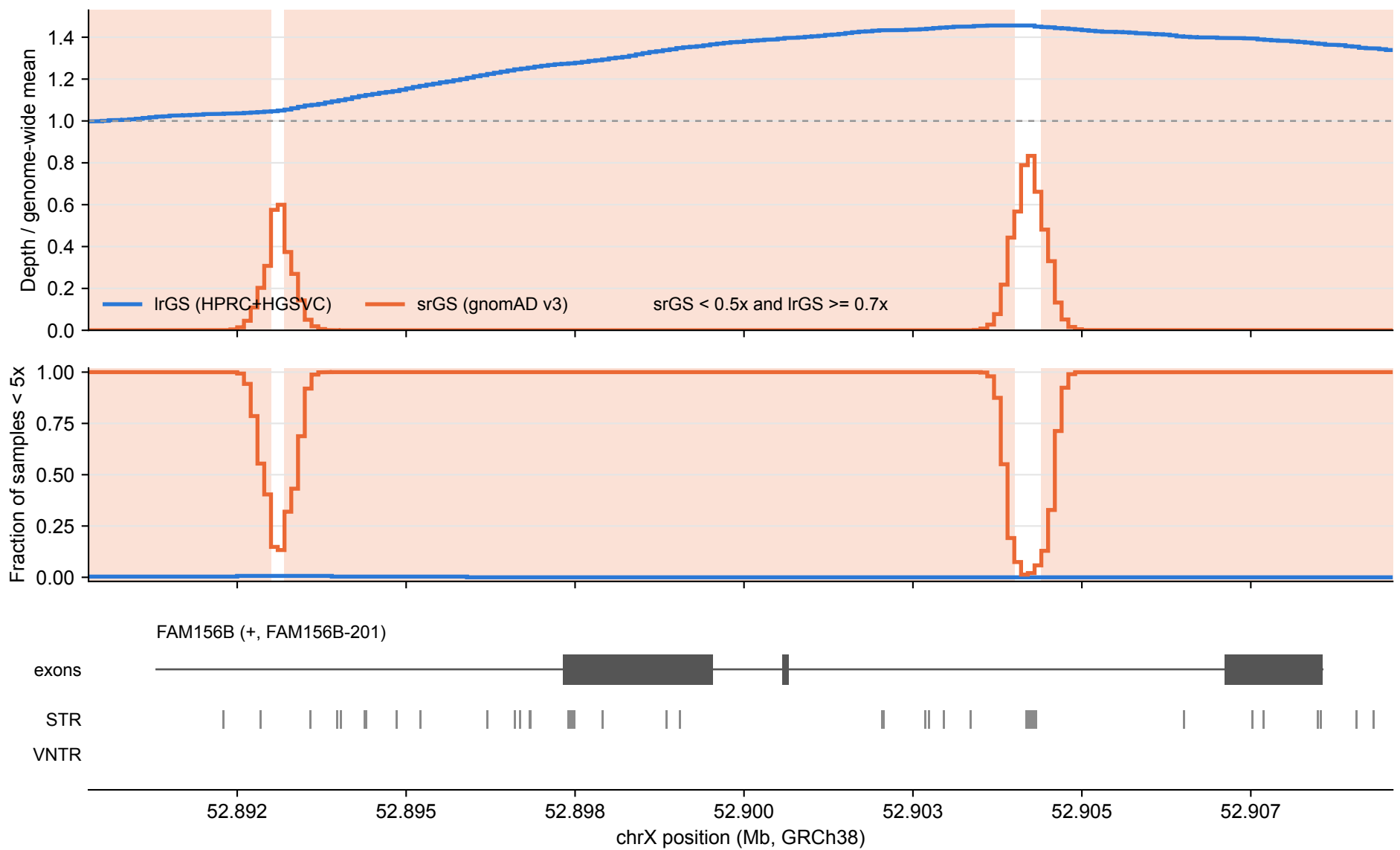
FAM156B: lrGS vs srGS coverage over tandem repeats (100 bp bins)
