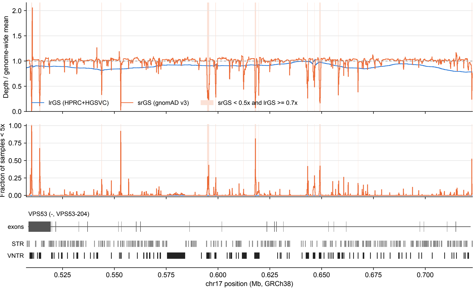
VPS53: lrGS vs srGS coverage over tandem repeats (100 bp bins)
