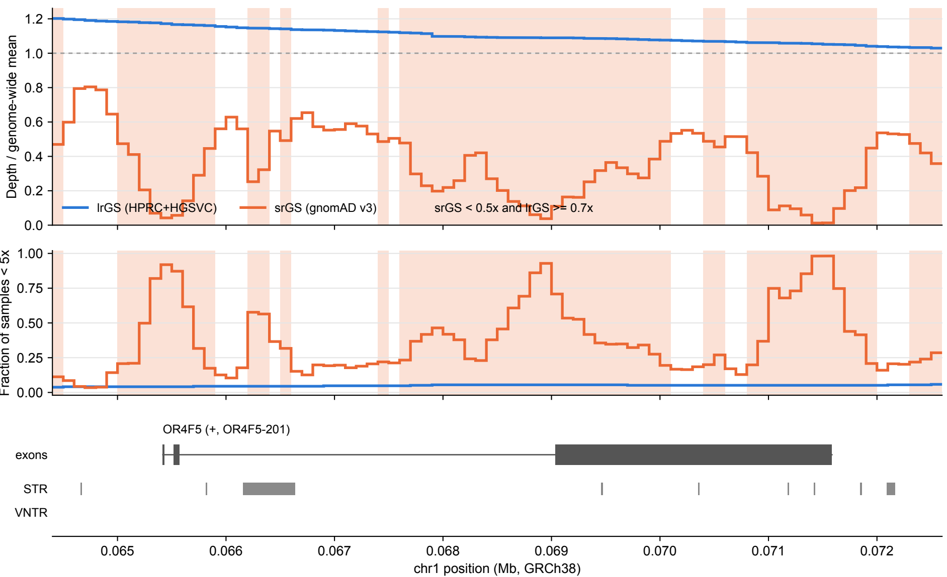
OR4F5: lrGS vs srGS coverage over tandem repeats (100 bp bins)
