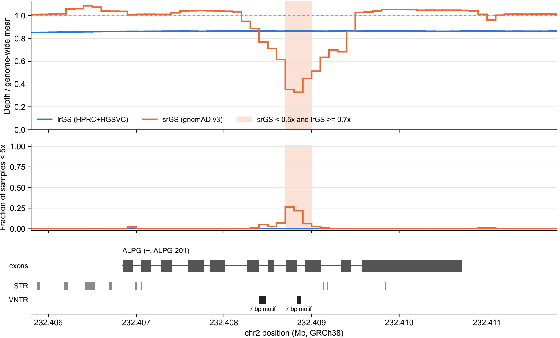
ALPG: IrGS vs srGS coverage over tandem repeats (100 bp bins)
