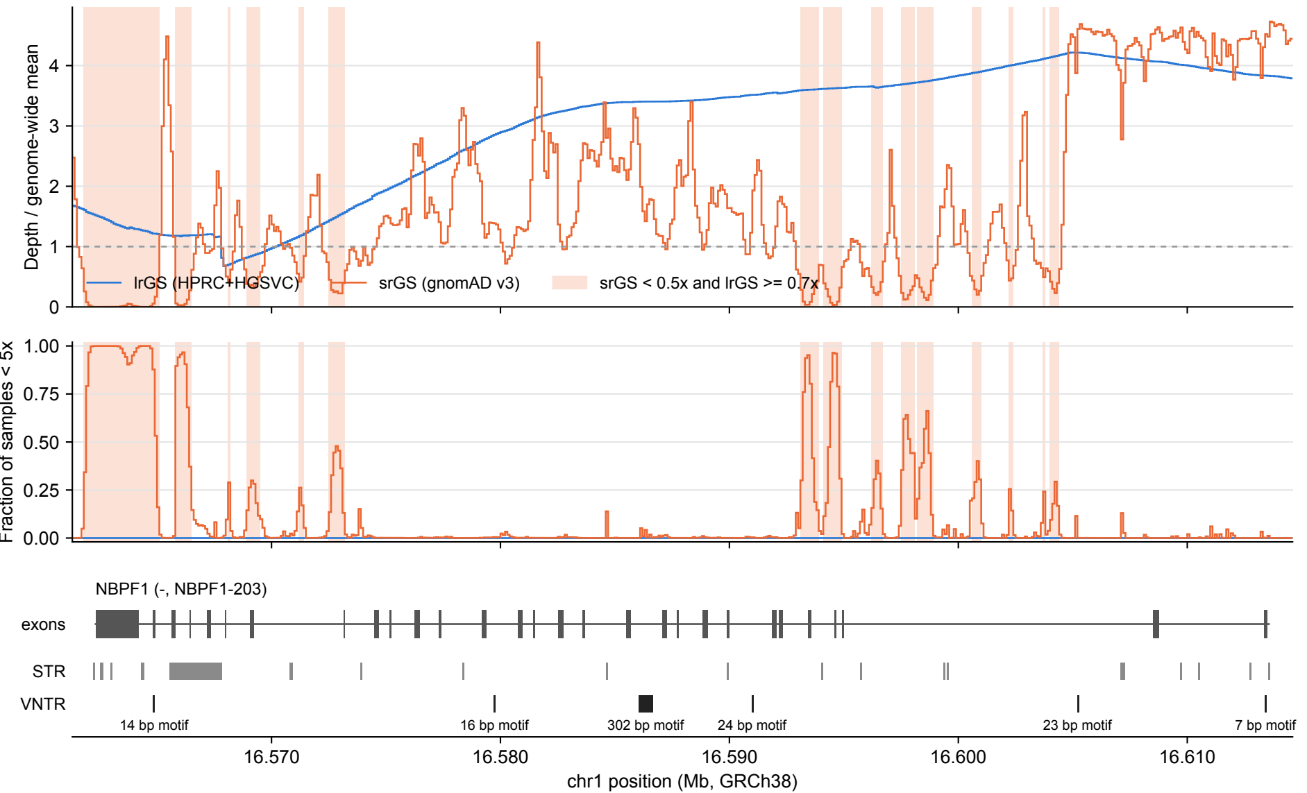
NBPF1: lrGS vs srGS coverage over tandem repeats (100 bp bins)
