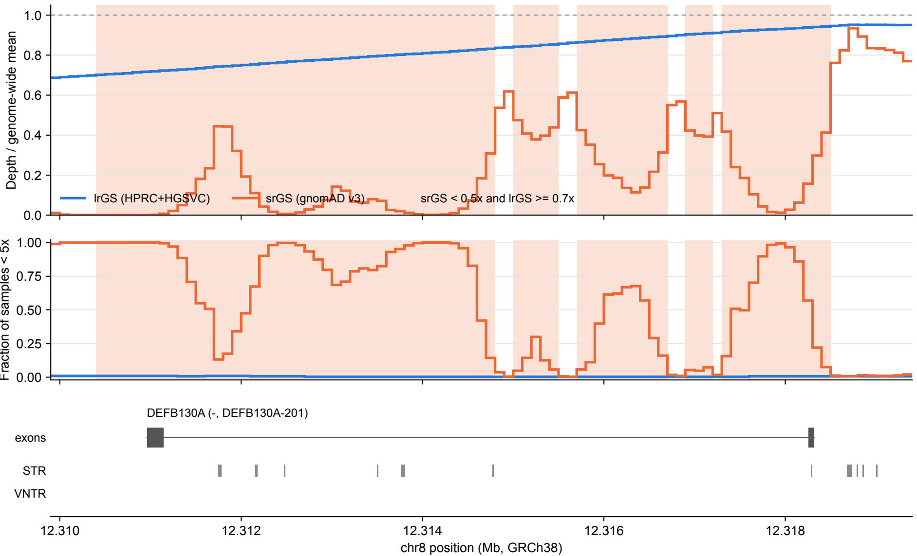
DEFB130A: lrGS vs srGS coverage over tandem repeats (100 bp bins)
