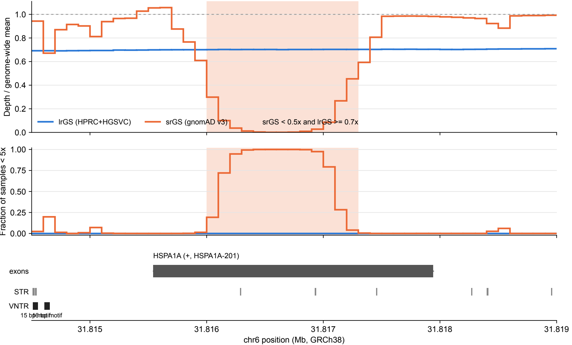
HSPA1A: IrGS vs srGS coverage over tandem repeats (100 bp bins)
