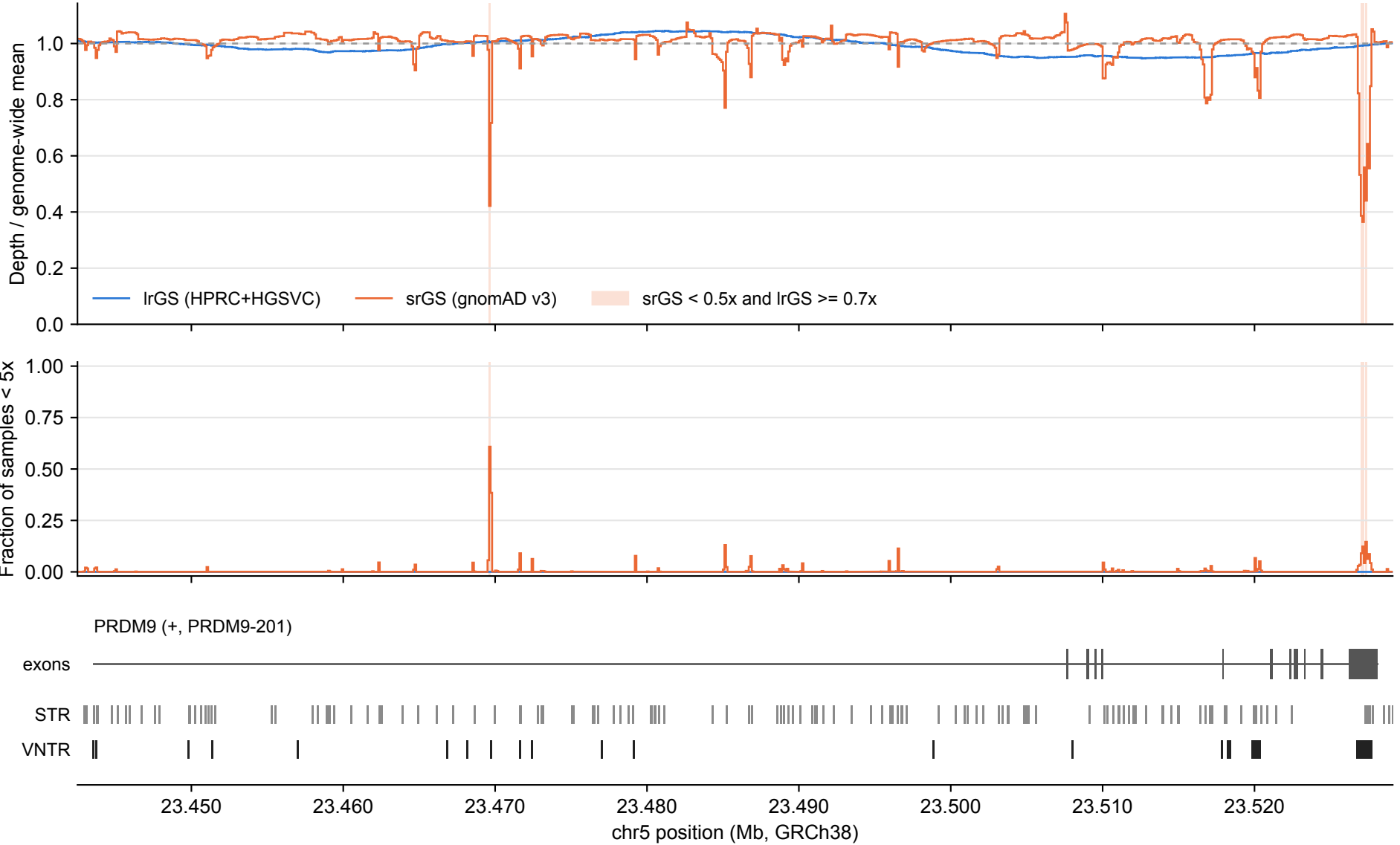
PRDM9: lrGS vs srGS coverage over tandem repeats (100 bp bins)
