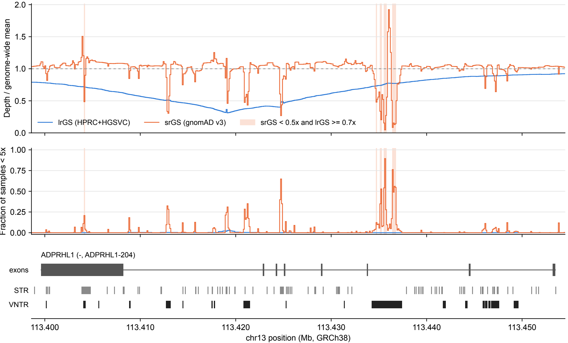
ADPRHL1: lrGS vs srGS coverage over tandem repeats (100 bp bins)
