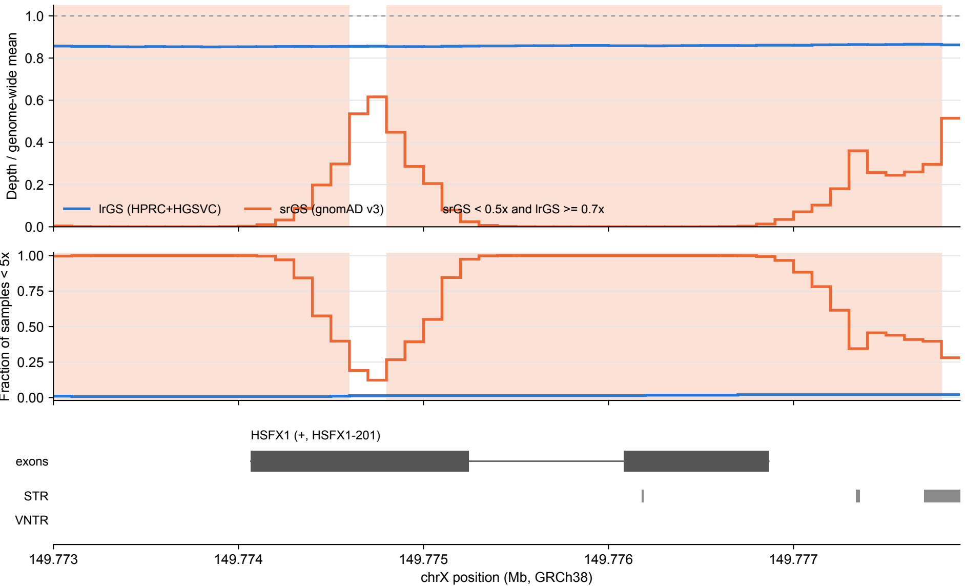
HSFX1: lrGS vs srGS coverage over tandem repeats (100 bp bins)
