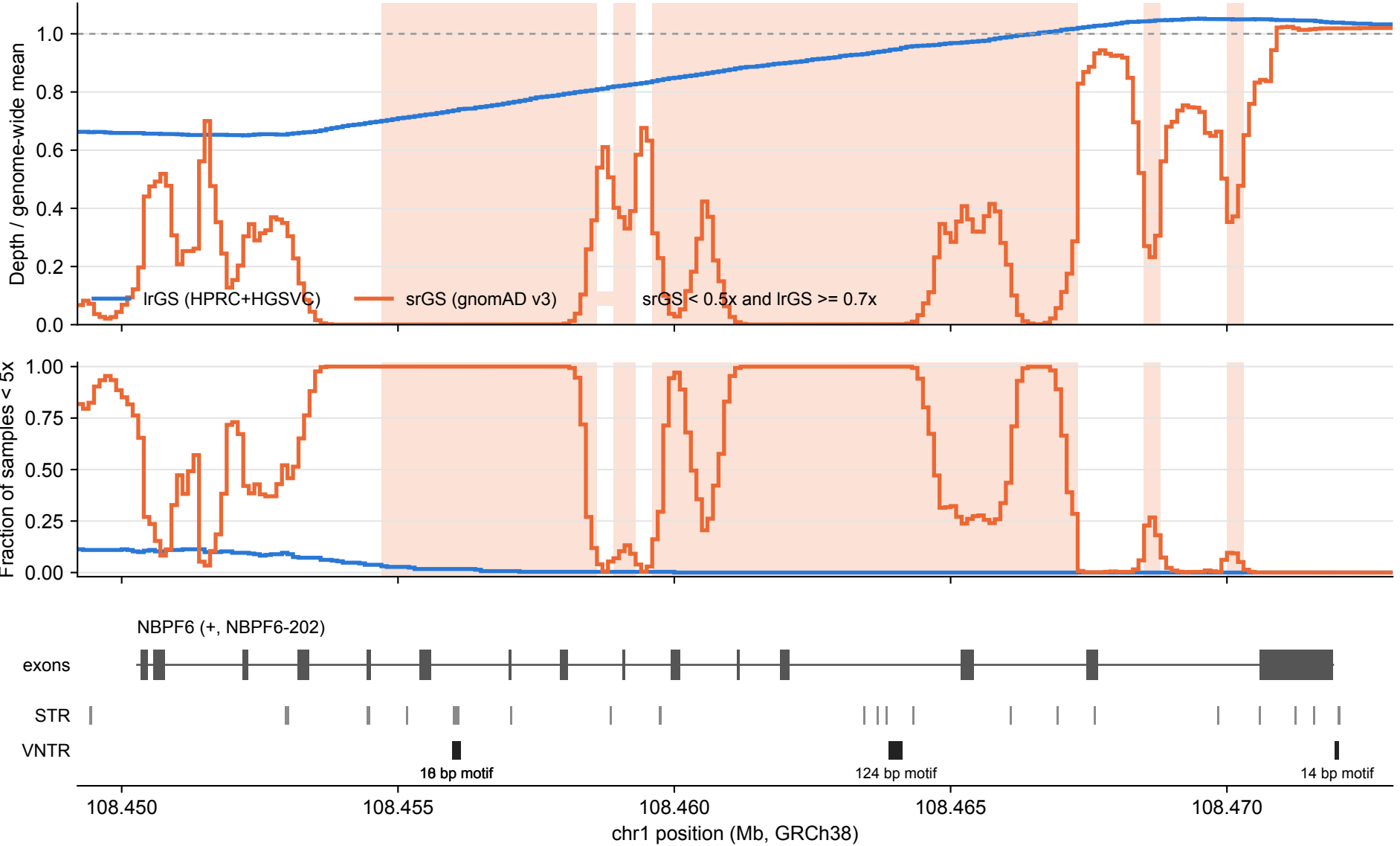
NBPF6: IrGS vs srGS coverage over tandem repeats (100 bp bins)
