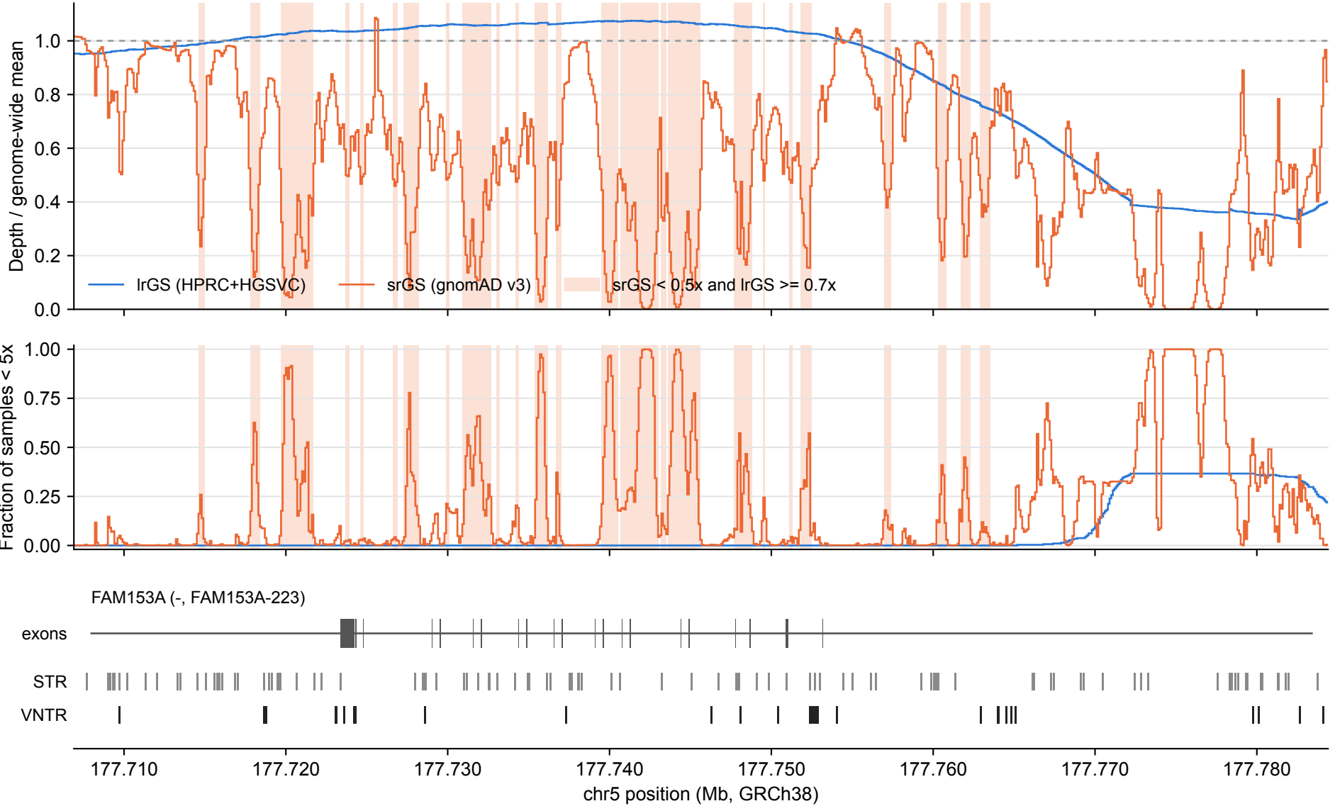
FAM153A: IrGS vs srGS coverage over tandem repeats (100 bp bins)
