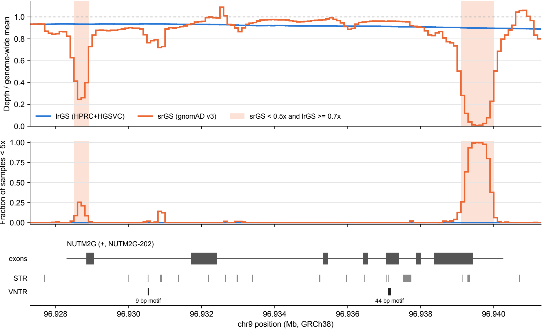
NUTM2G: lrGS vs srGS coverage over tandem repeats (100 bp bins)
