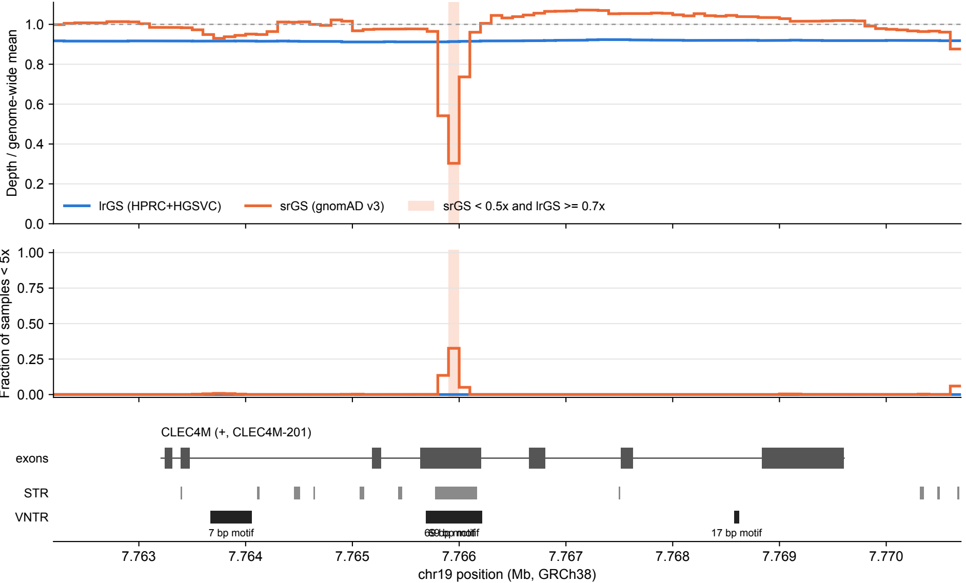
CLEC4M: lrGS vs srGS coverage over tandem repeats (100 bp bins)
