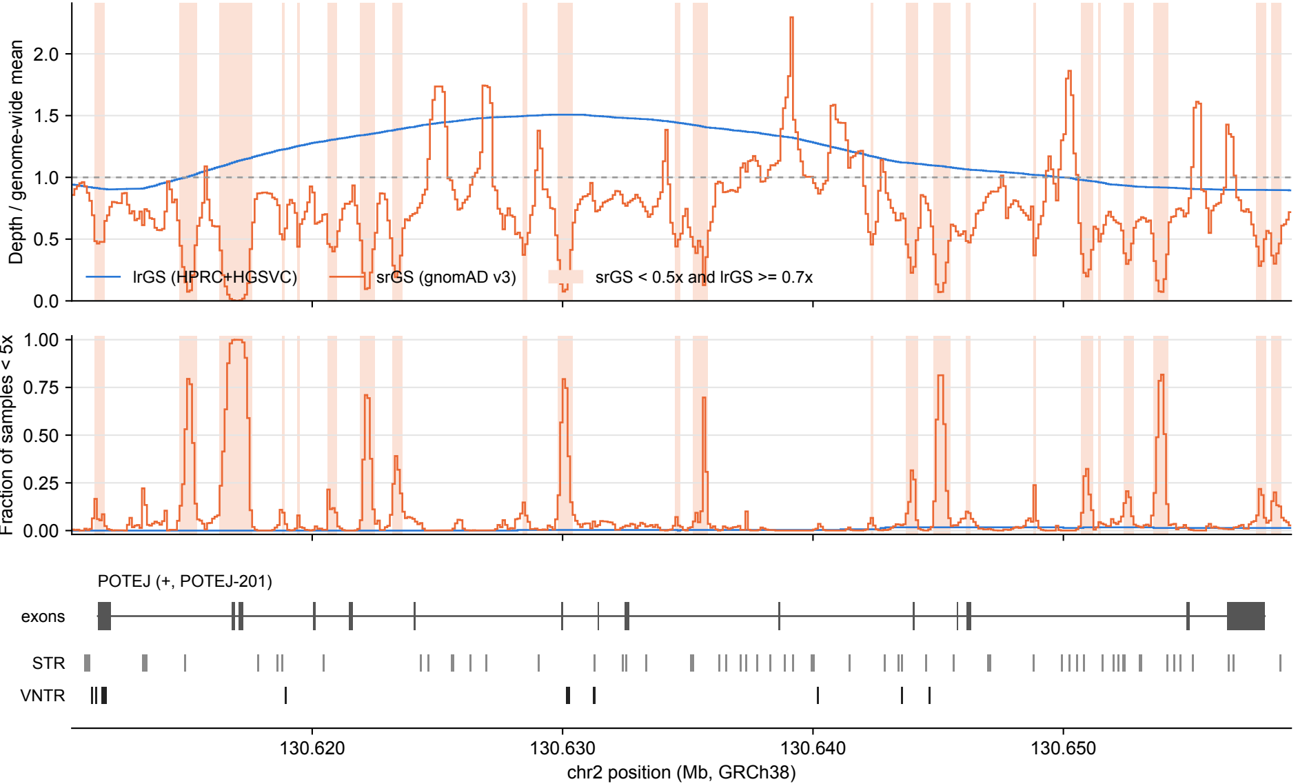
POTEJ: IrGS vs srGS coverage over tandem repeats (100 bp bins)
