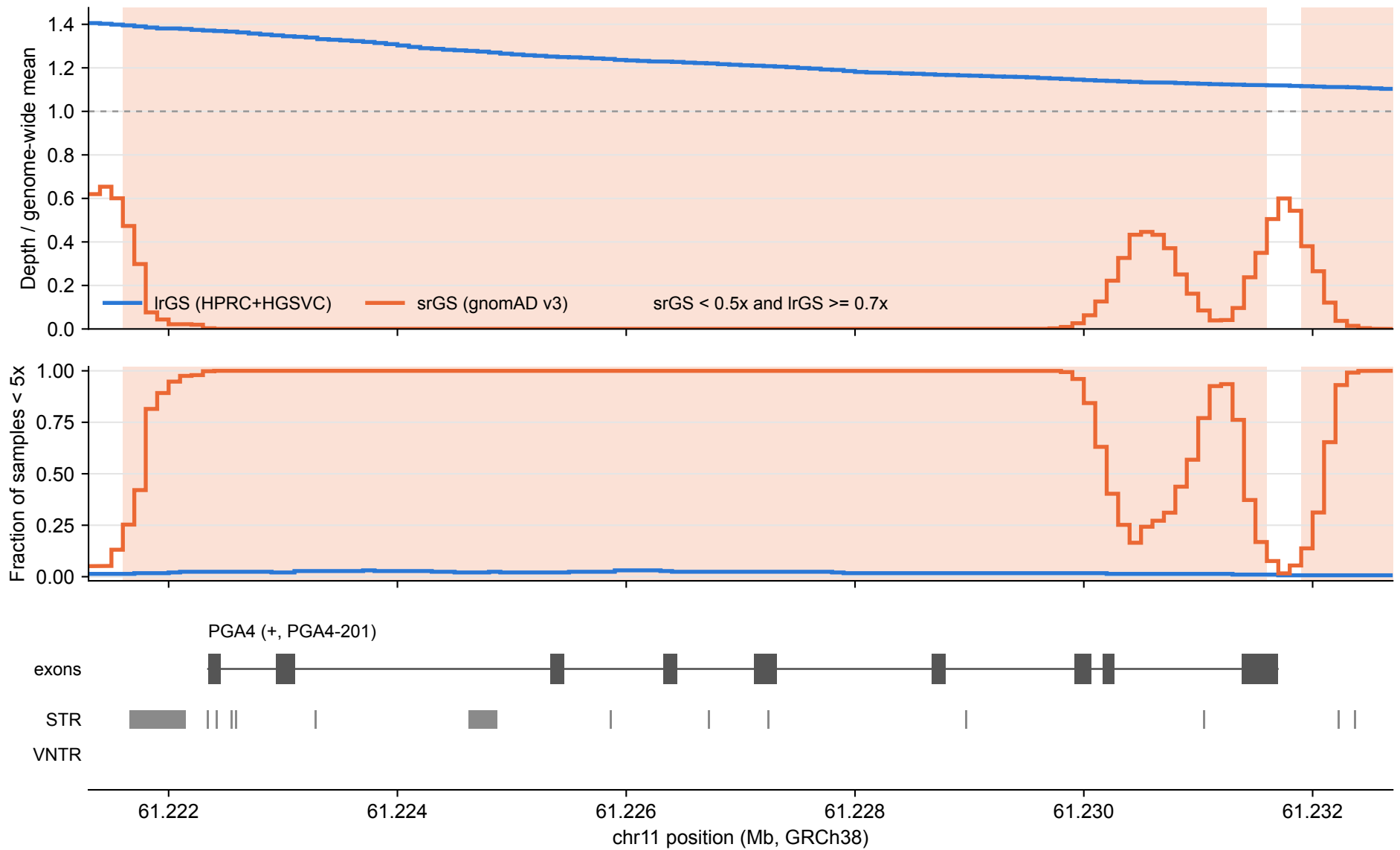
PGA4: lrGS vs srGS coverage over tandem repeats (100 bp bins)
