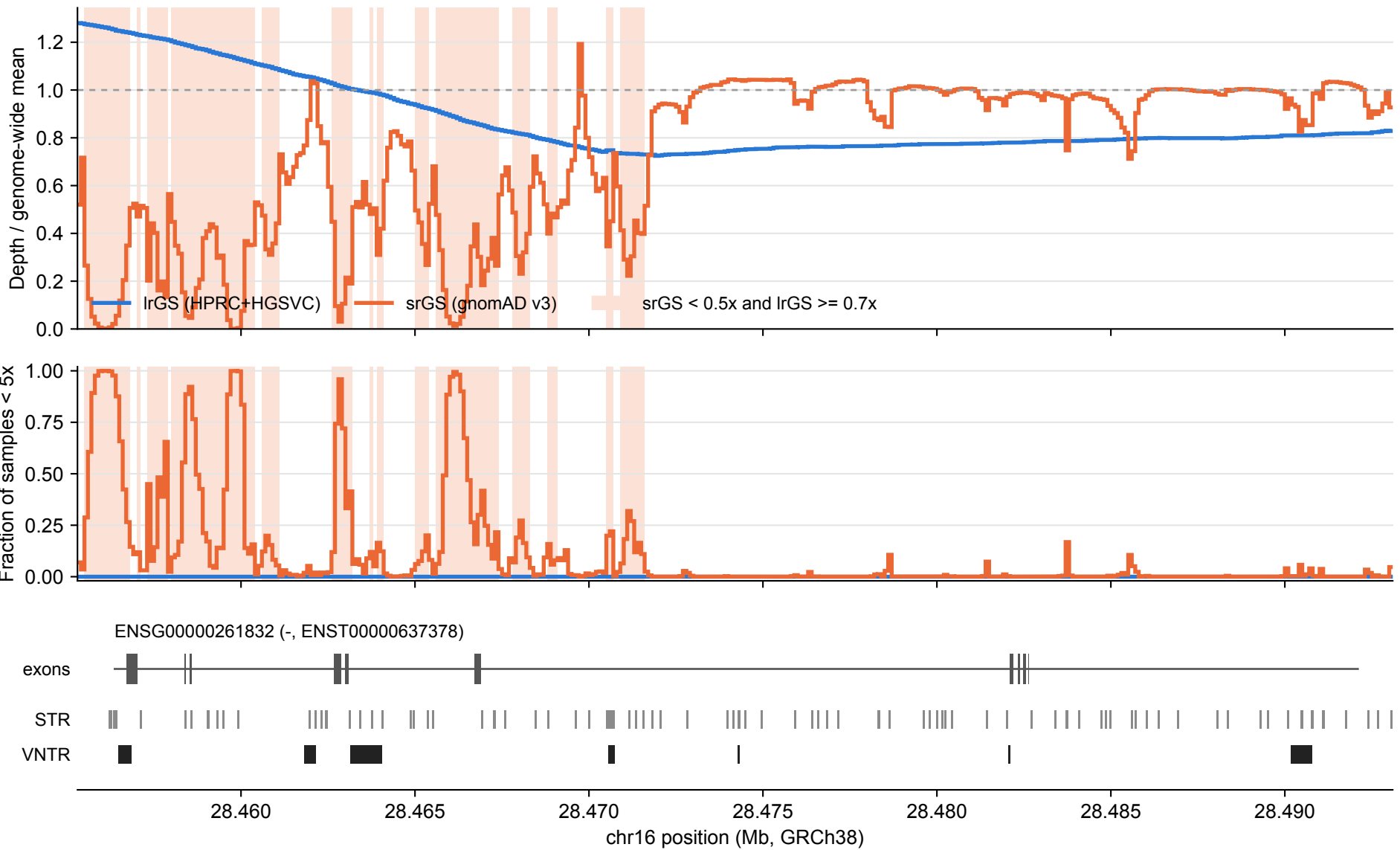
ENSG00000261832: lrGS vs srGS coverage over tandem repeats (100 bp bins)
