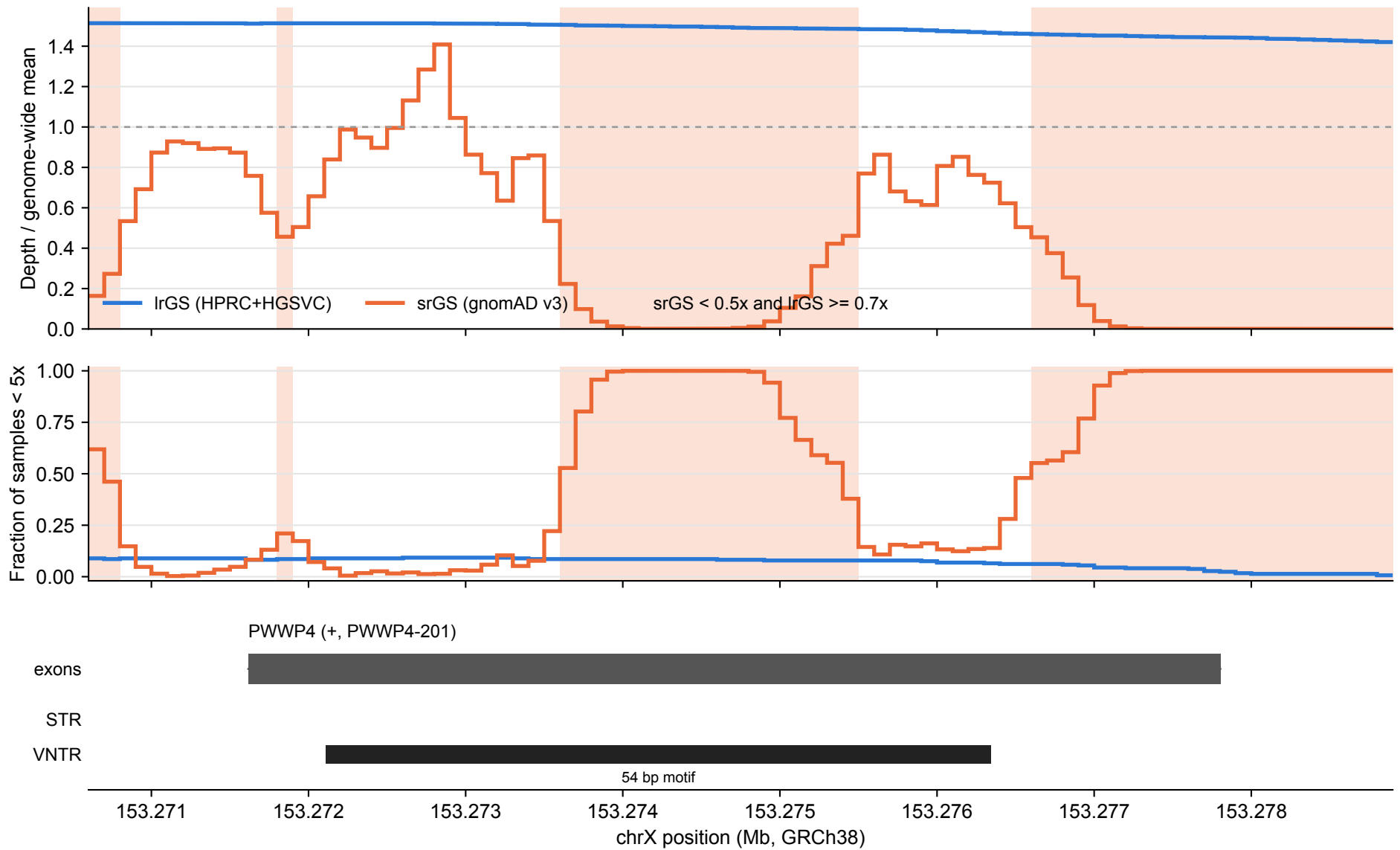
PWWP4: lrGS vs srGS coverage over tandem repeats (100 bp bins)
