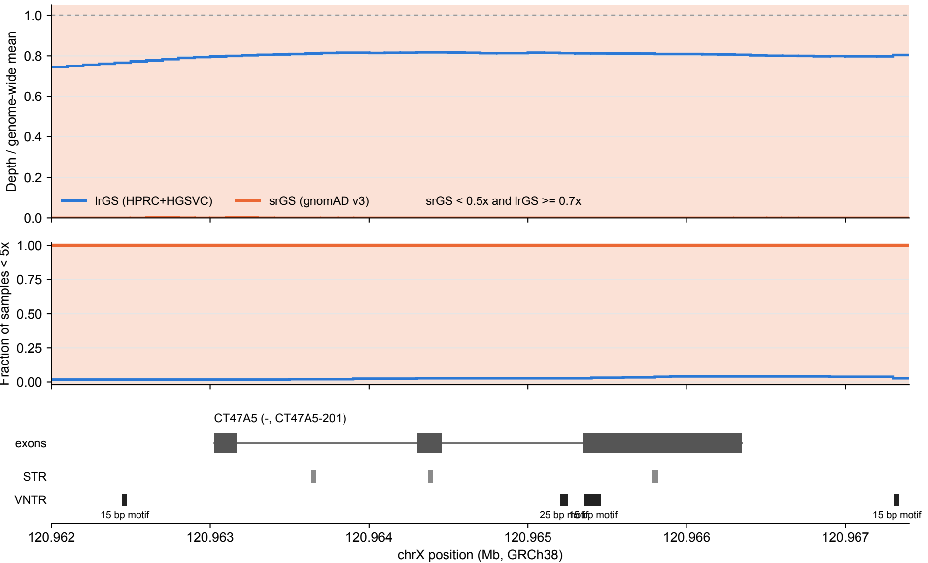
CT47A5: lrGS vs srGS coverage over tandem repeats (100 bp bins)
