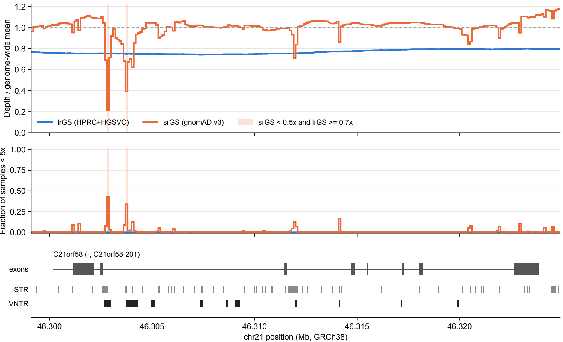
C21orf58: lrGS vs srGS coverage over tandem repeats (100 bp bins)
