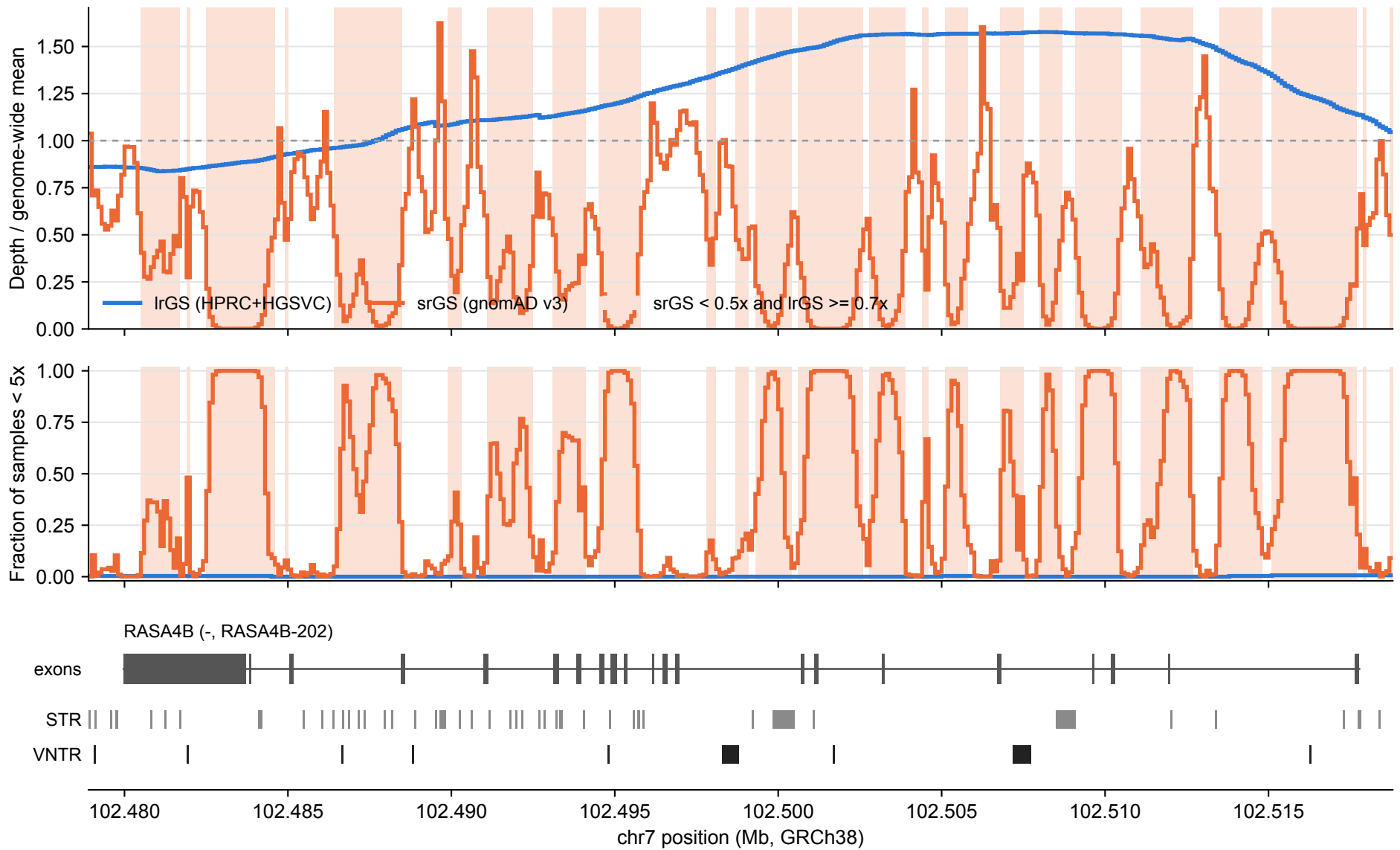
RASA4B: lrGS vs srGS coverage over tandem repeats (100 bp bins)
