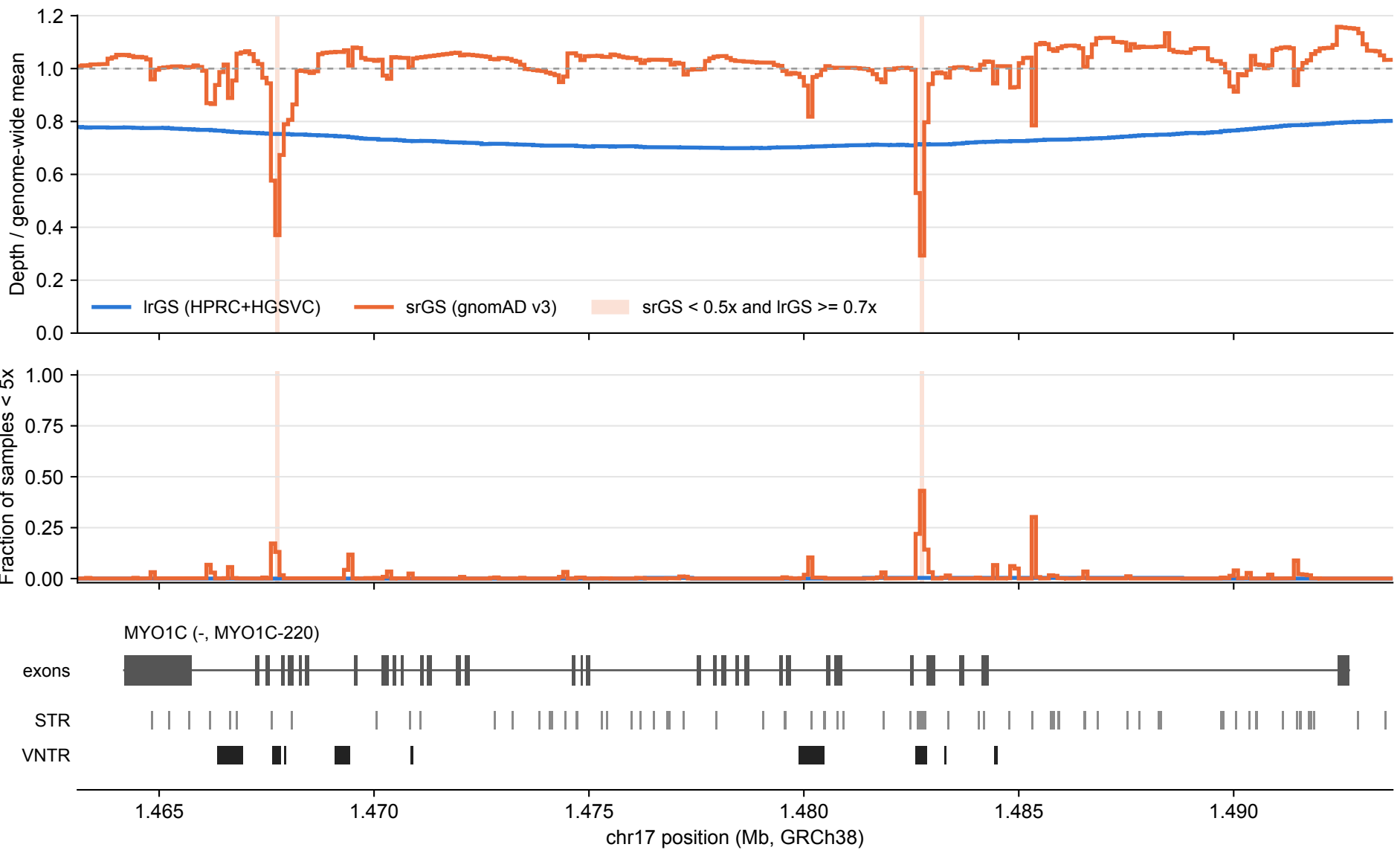
MYO1C: IrGS vs srGS coverage over tandem repeats (100 bp bins)
