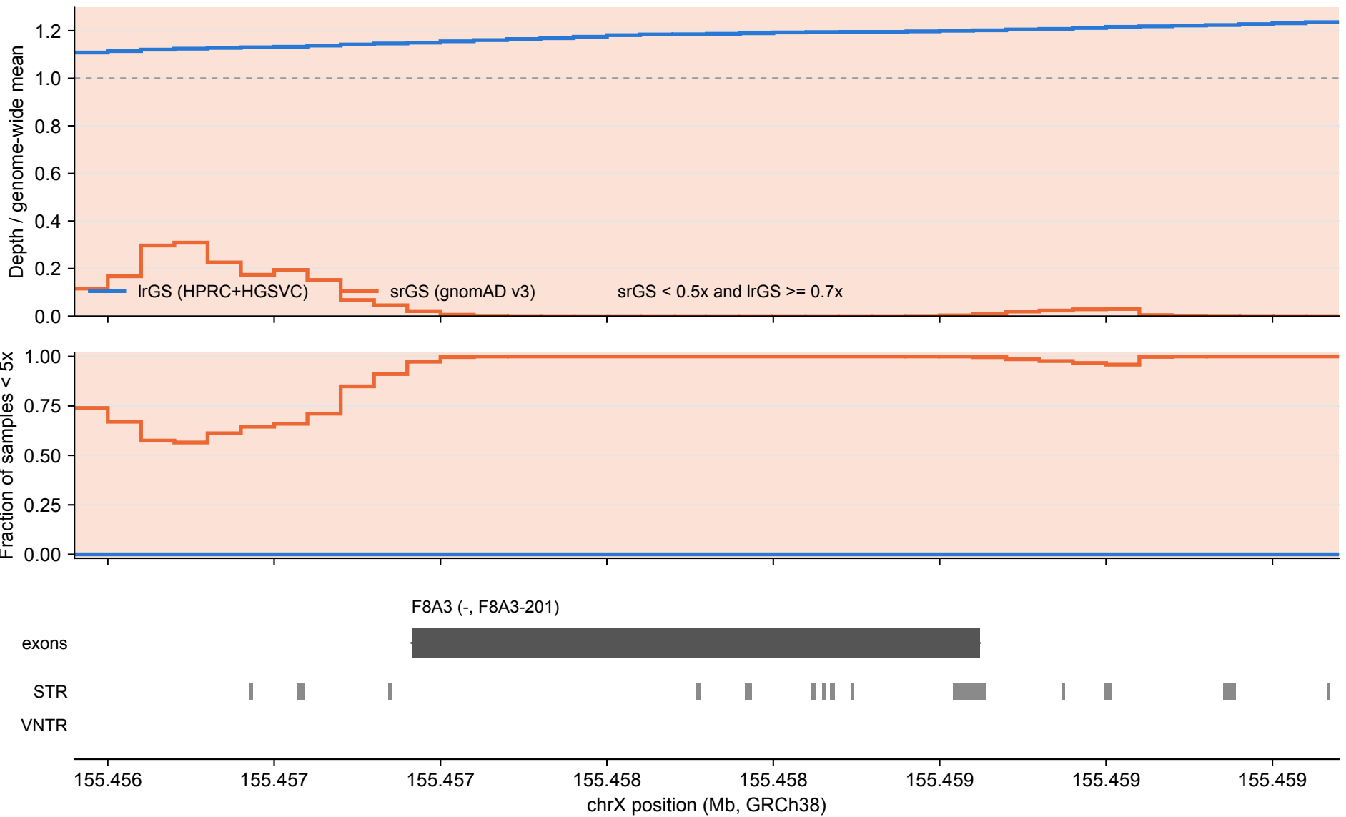
F8A3: lrGS vs srGS coverage over tandem repeats (100 bp bins)
