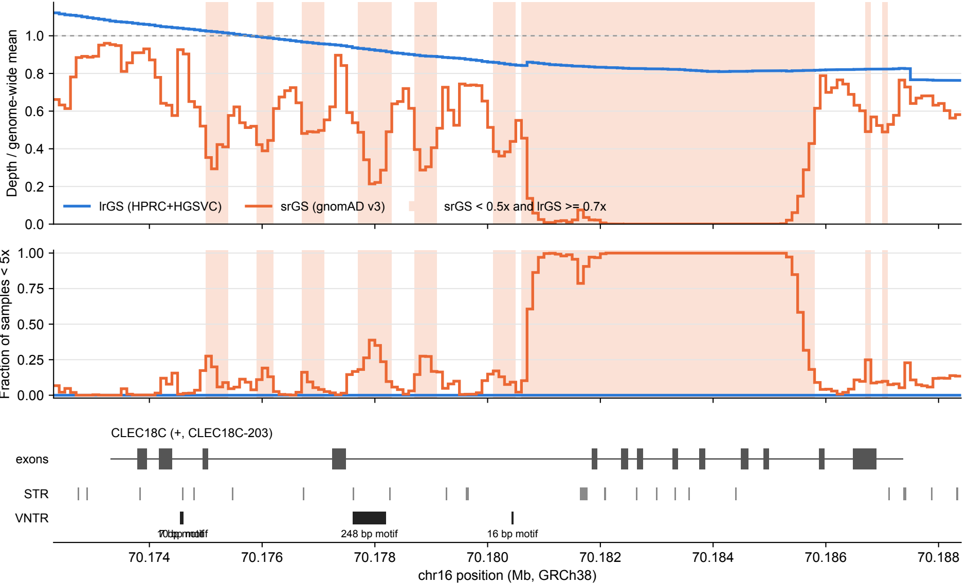
CLEC18C: lrGS vs srGS coverage over tandem repeats (100 bp bins)
