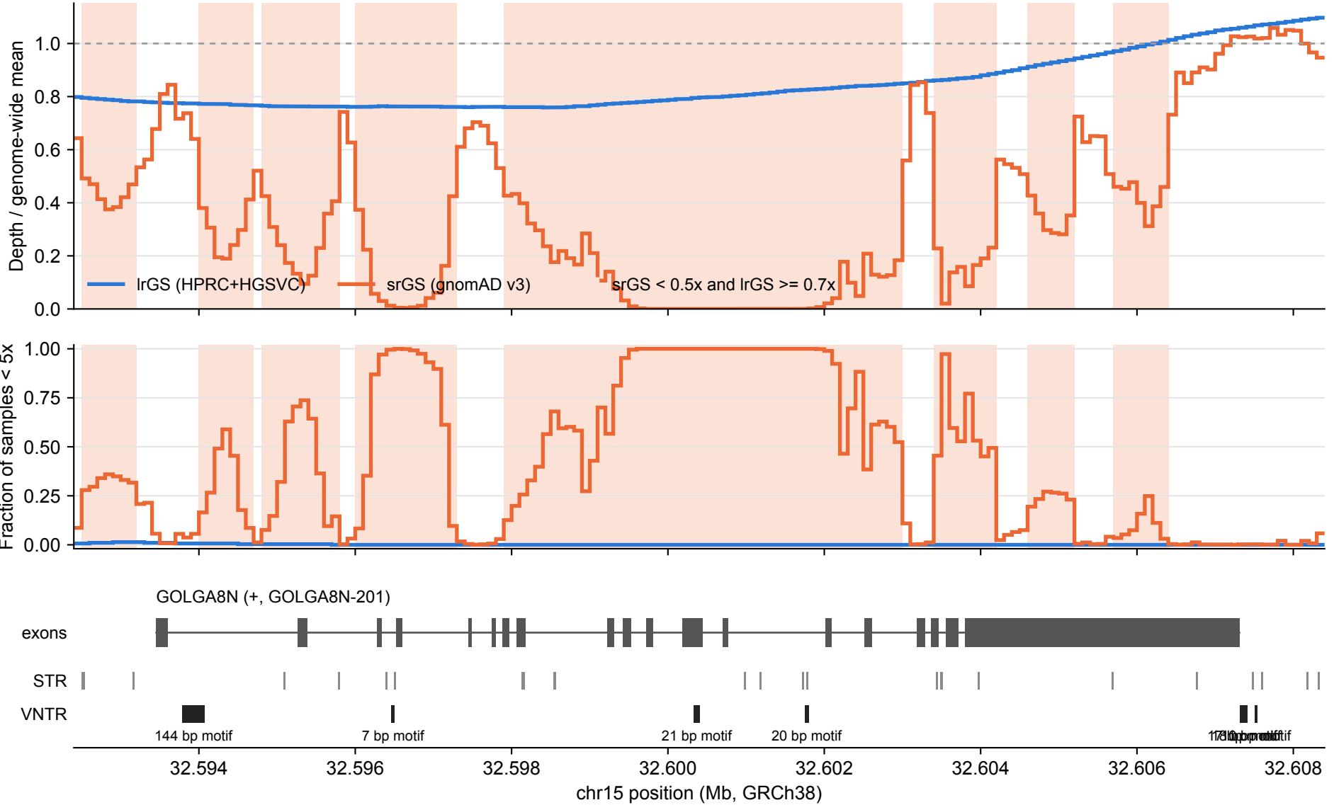
GOLGA8N: lrGS vs srGS coverage over tandem repeats (100 bp bins)
