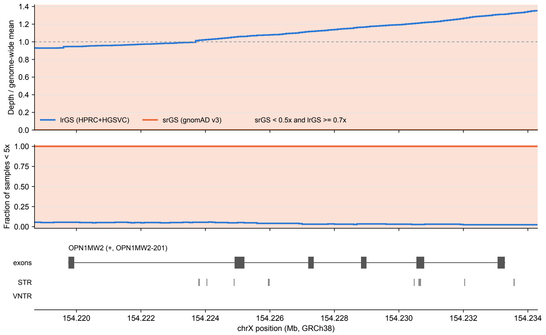
OPN1MW2: lrGS vs srGS coverage over tandem repeats (100 bp bins)
