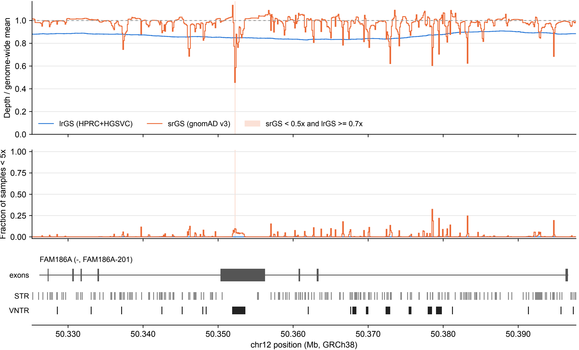
FAM186A: lrGS vs srGS coverage over tandem repeats (100 bp bins)
