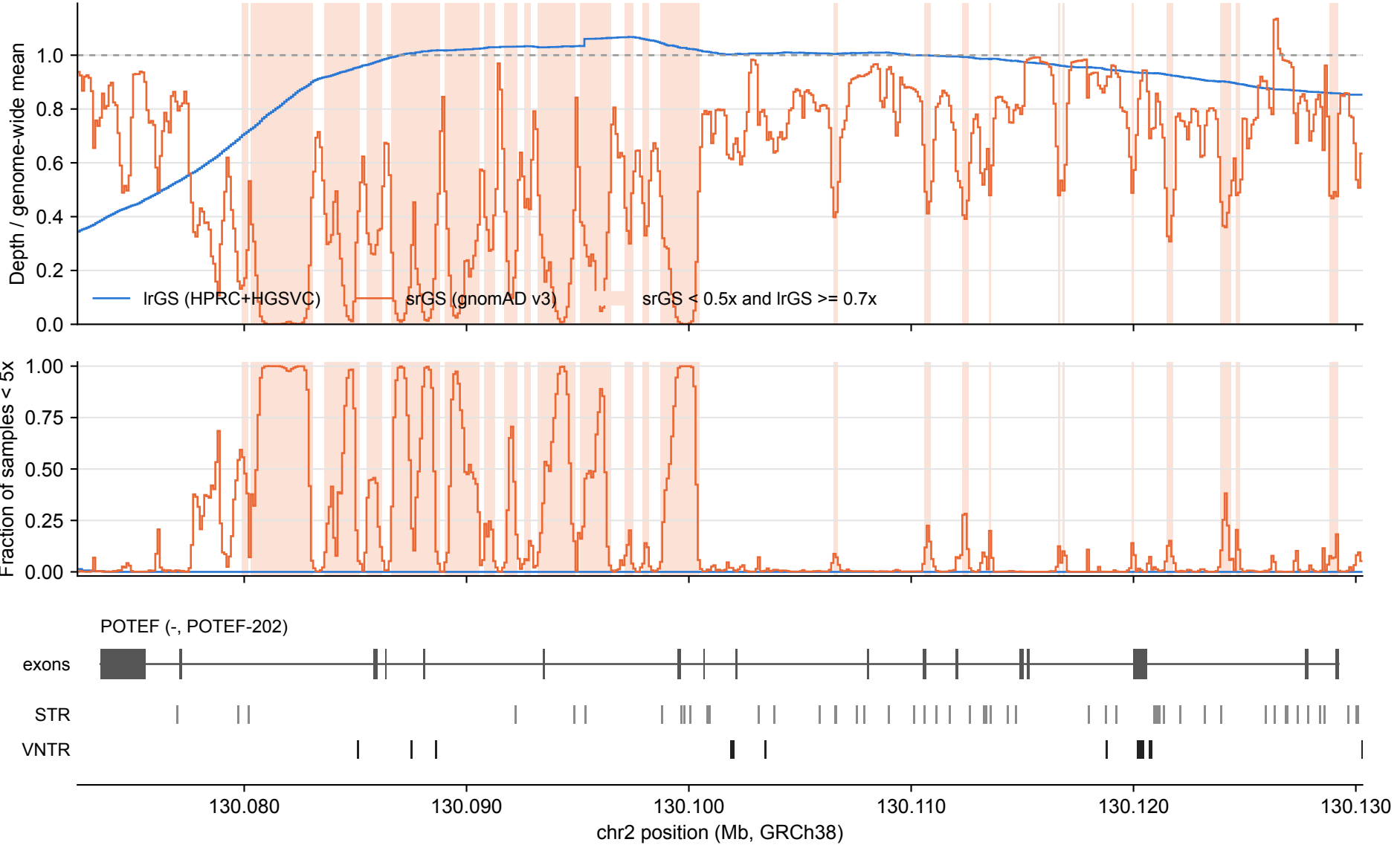
POTEF: IrGS vs srGS coverage over tandem repeats (100 bp bins)
