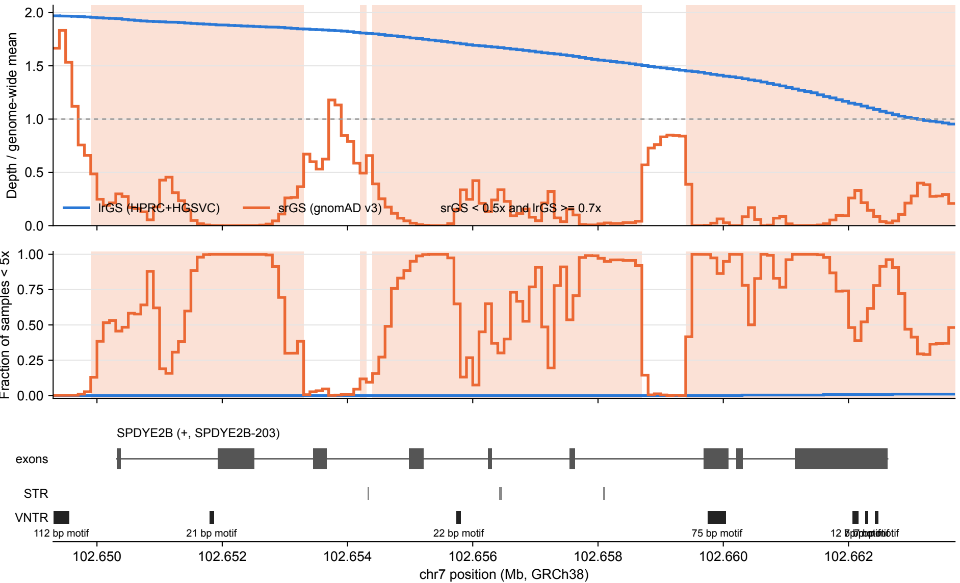
SPDYE2B: lrGS vs srGS coverage over tandem repeats (100 bp bins)
