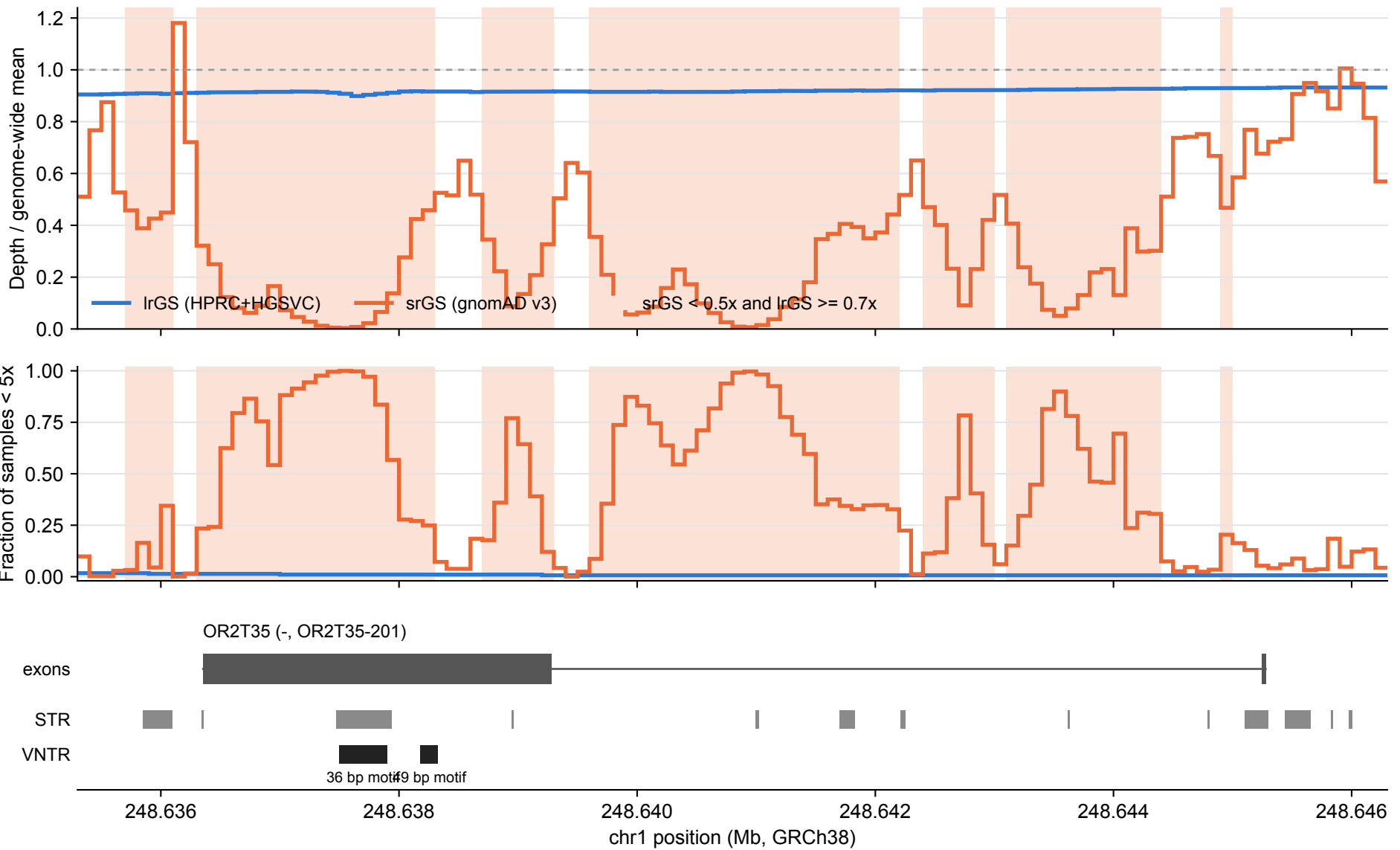
OR2T35: IrGS vs srGS coverage over tandem repeats (100 bp bins)
