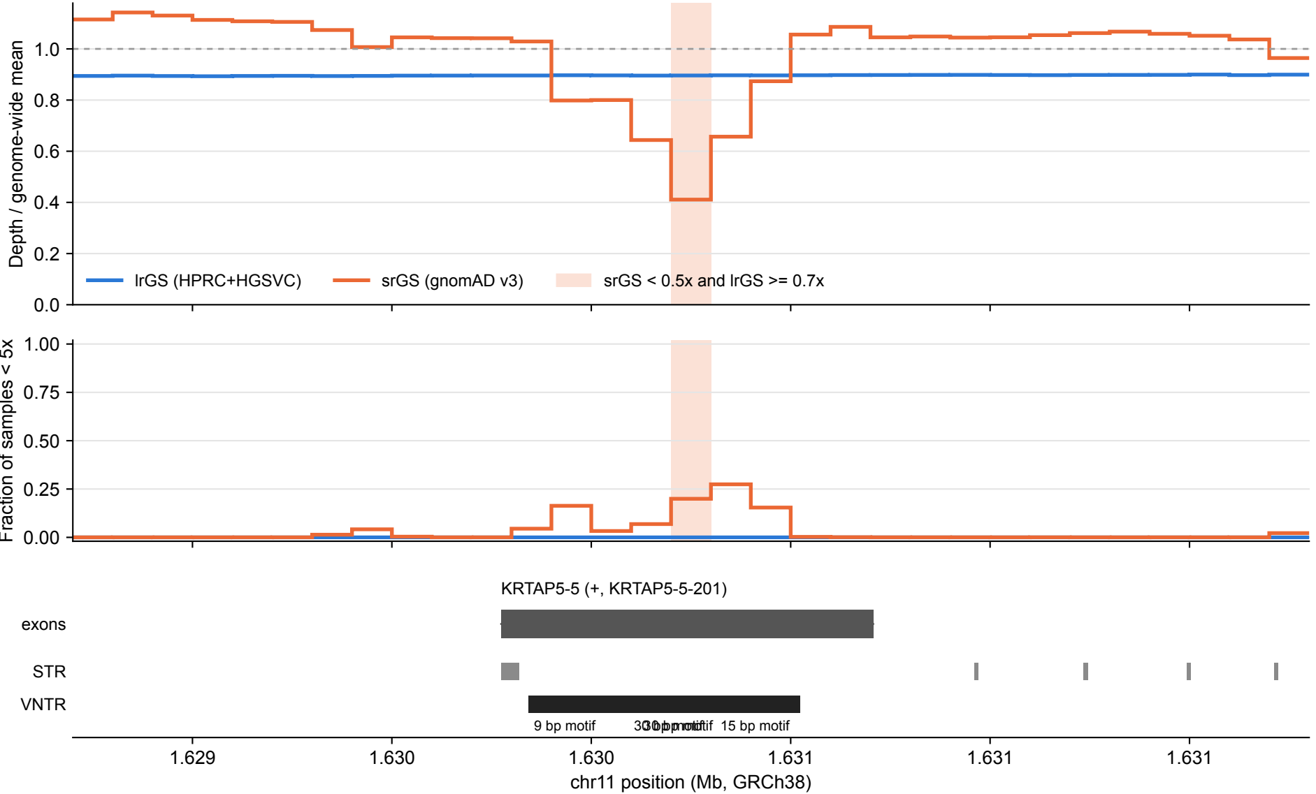
KRTAP5-5: lrGS vs srGS coverage over tandem repeats (100 bp bins)
