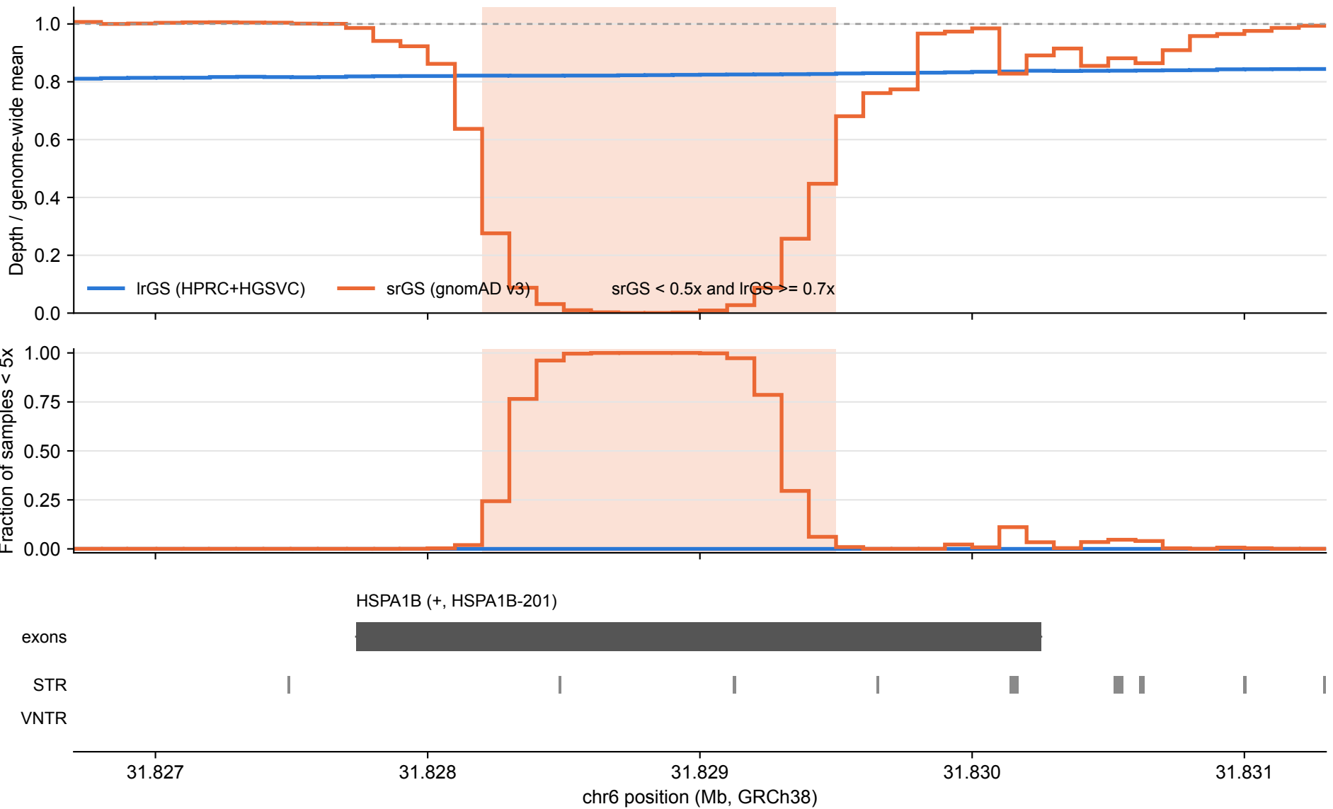
HSPA1B: IrGS vs srGS coverage over tandem repeats (100 bp bins)
