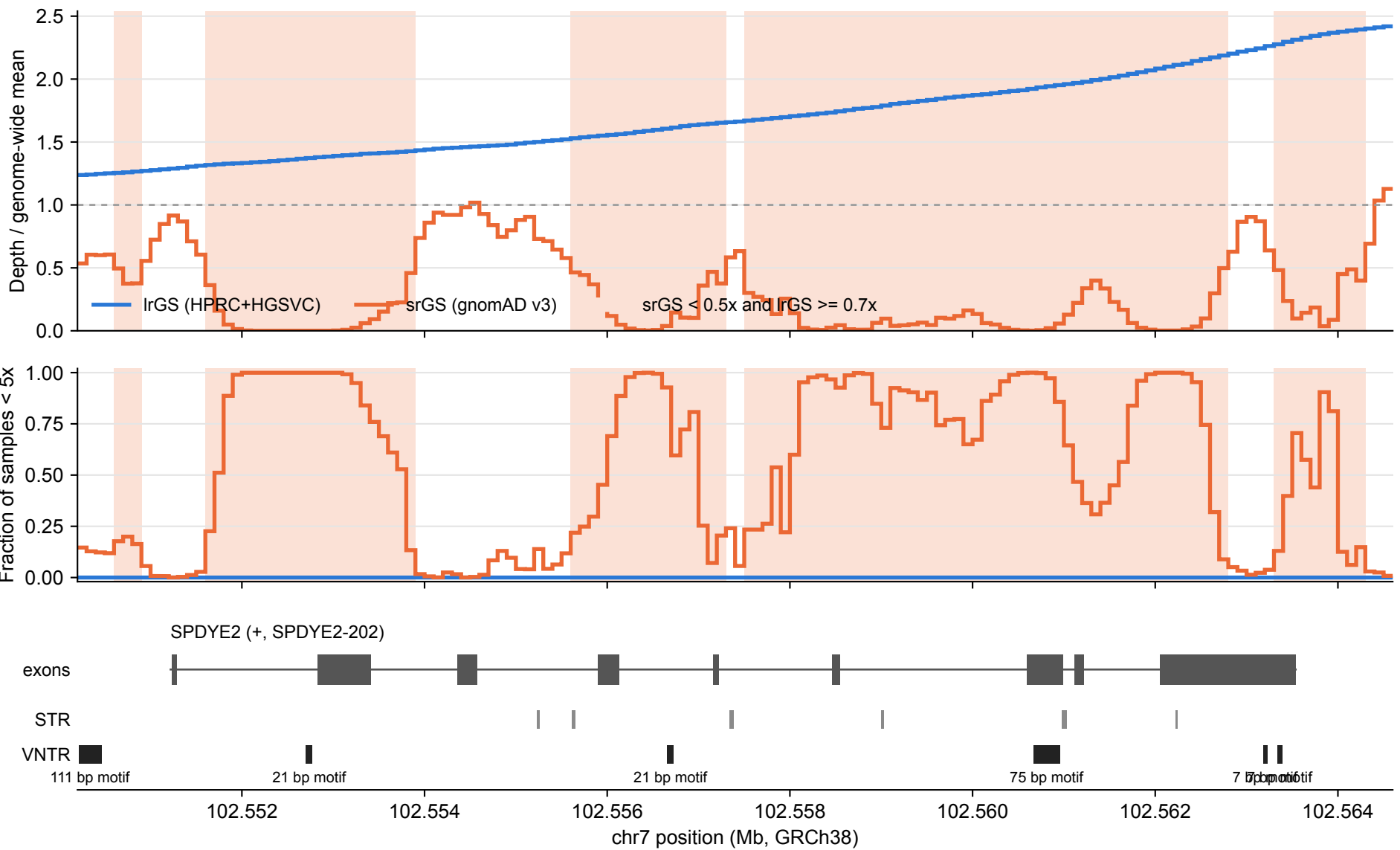
SPDYE2: lrGS vs srGS coverage over tandem repeats (100 bp bins)
