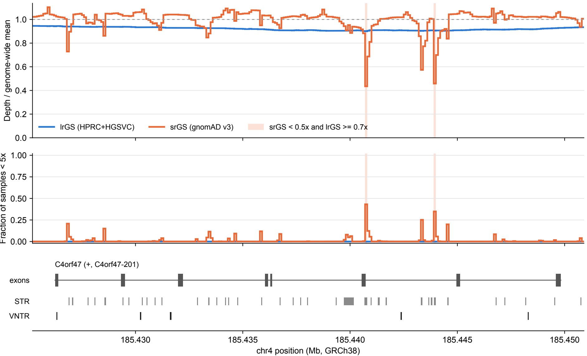
C4orf47: lrGS vs srGS coverage over tandem repeats (100 bp bins)
