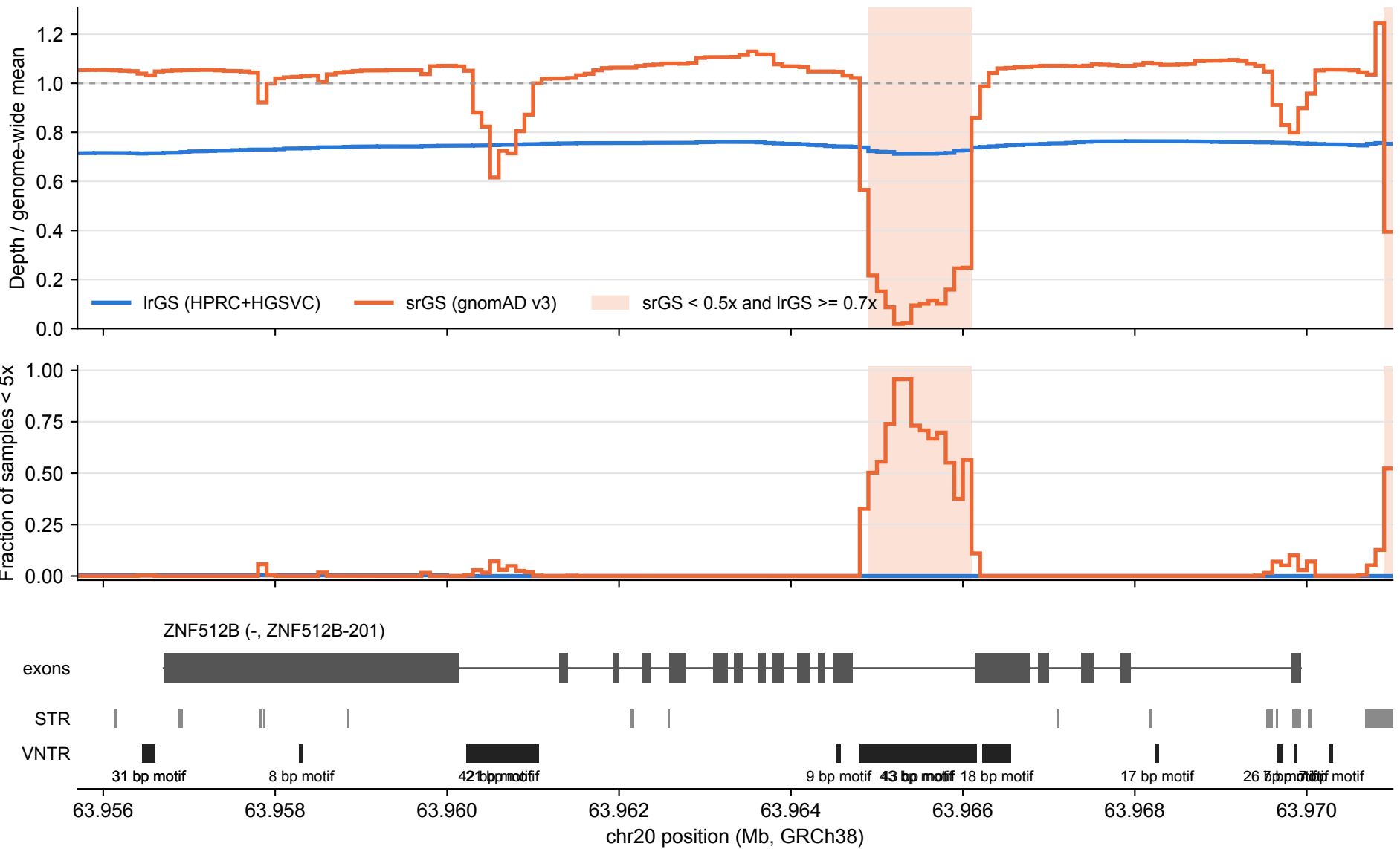
ZNF512B: lrGS vs srGS coverage over tandem repeats (100 bp bins)
