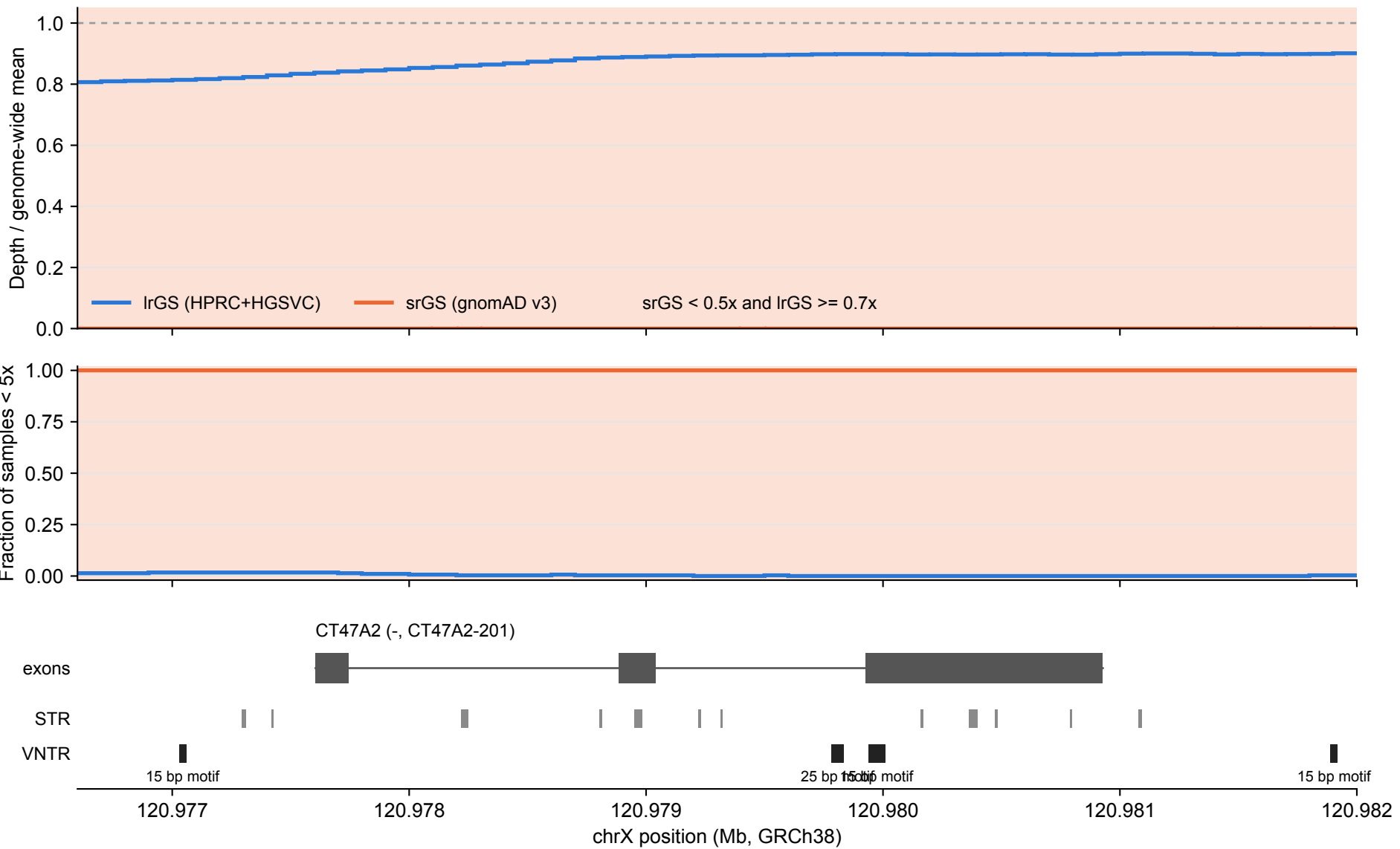
CT47A2: lrGS vs srGS coverage over tandem repeats (100 bp bins)
