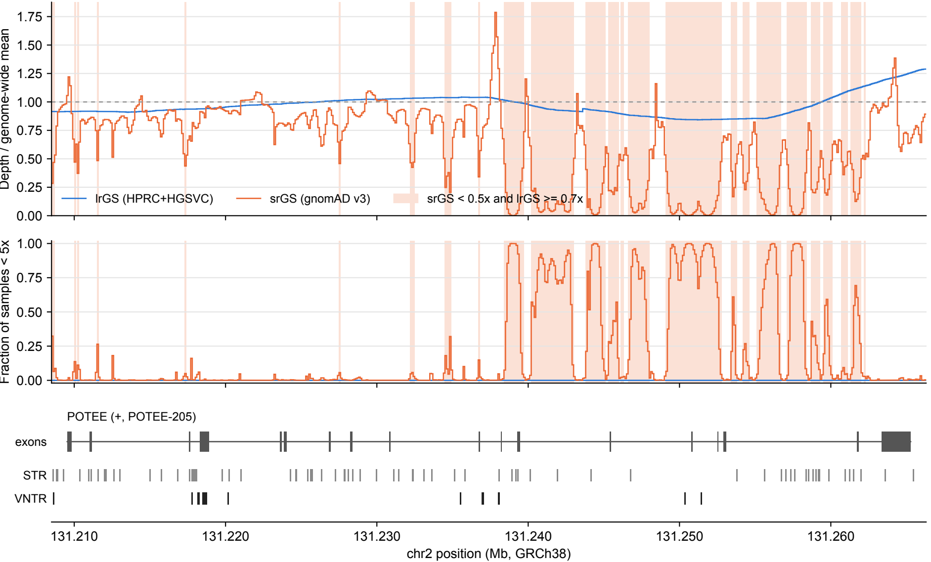
POTEE: lrGS vs srGS coverage over tandem repeats (100 bp bins)
