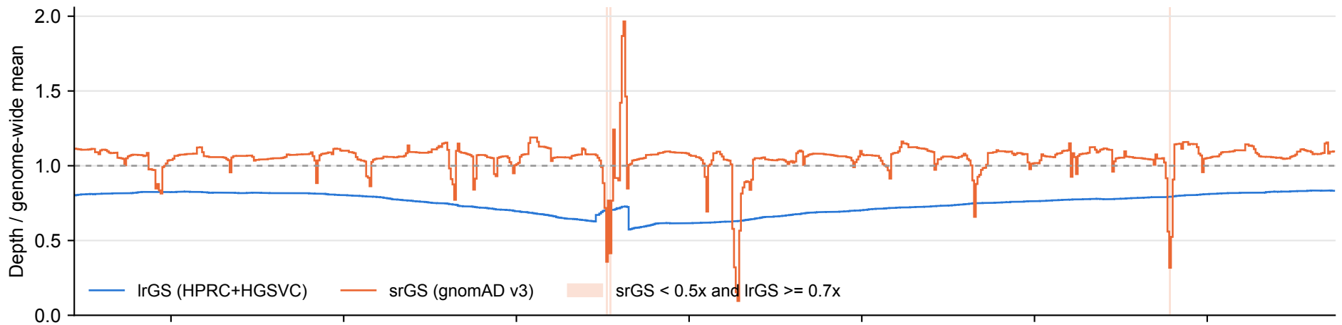
BAHCC1: lrGS vs srGS coverage over tandem repeats (100 bp bins)
