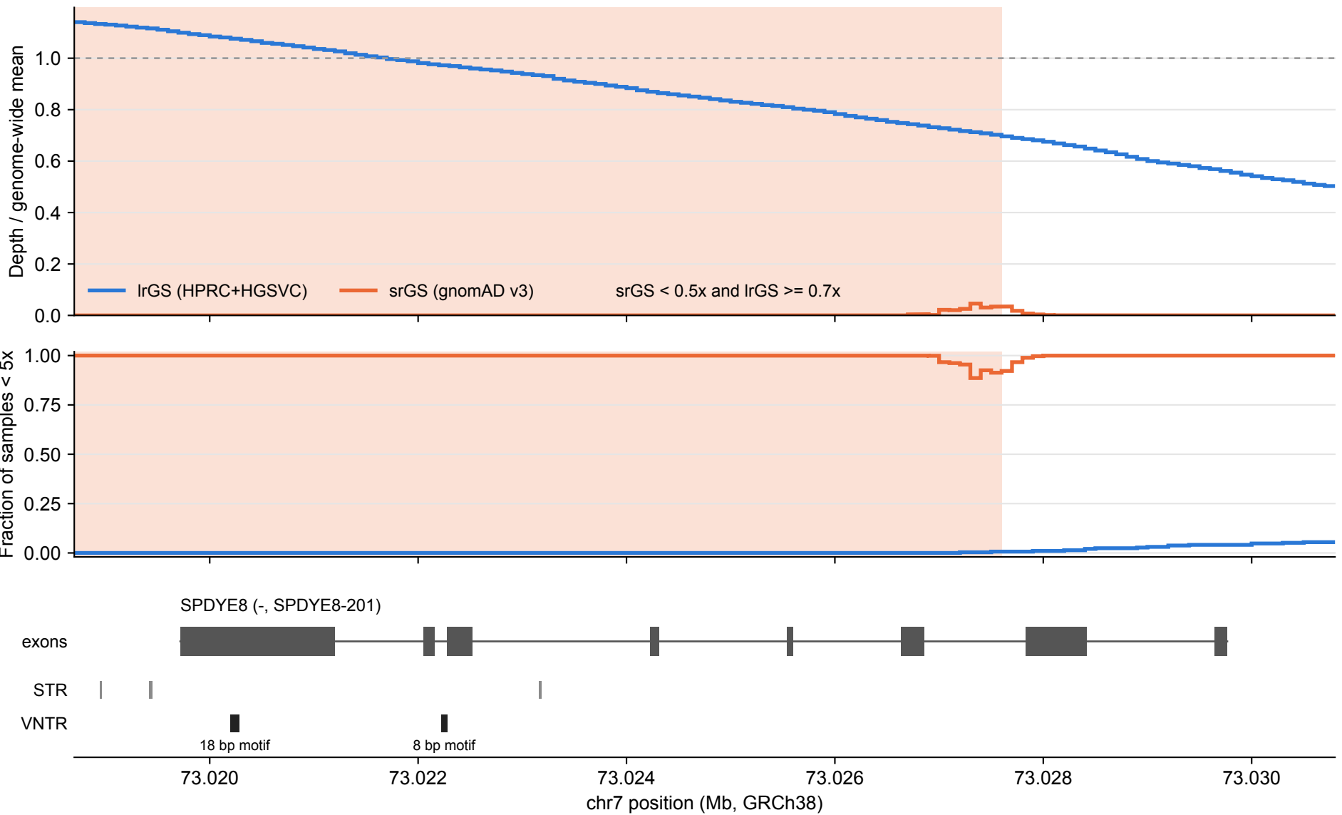
SPDYE8: lrGS vs srGS coverage over tandem repeats (100 bp bins)
