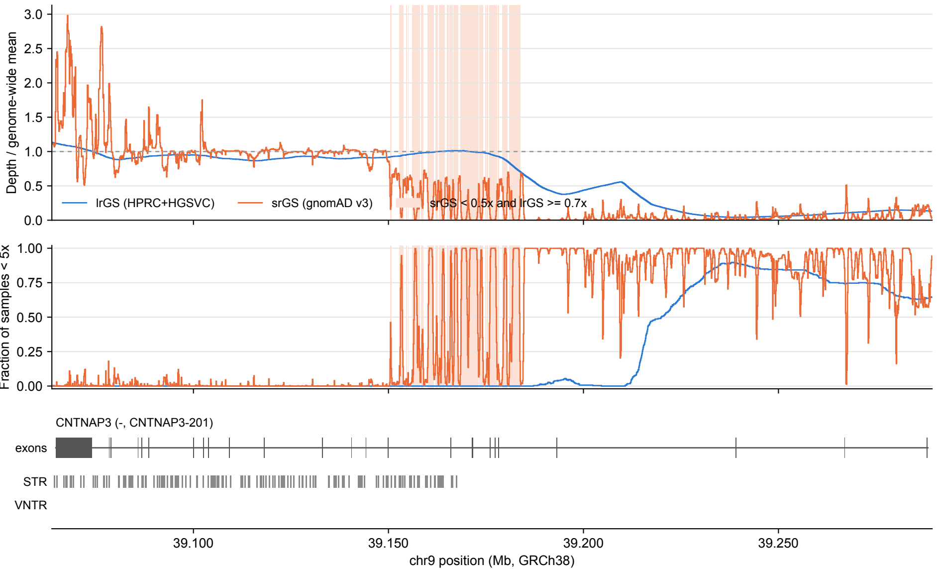
CNTNAP3: IrGS vs srGS coverage over tandem repeats (100 bp bins)
