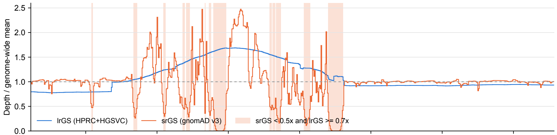
FCGBP: IrGS vs srGS coverage over tandem repeats (100 bp bins)
