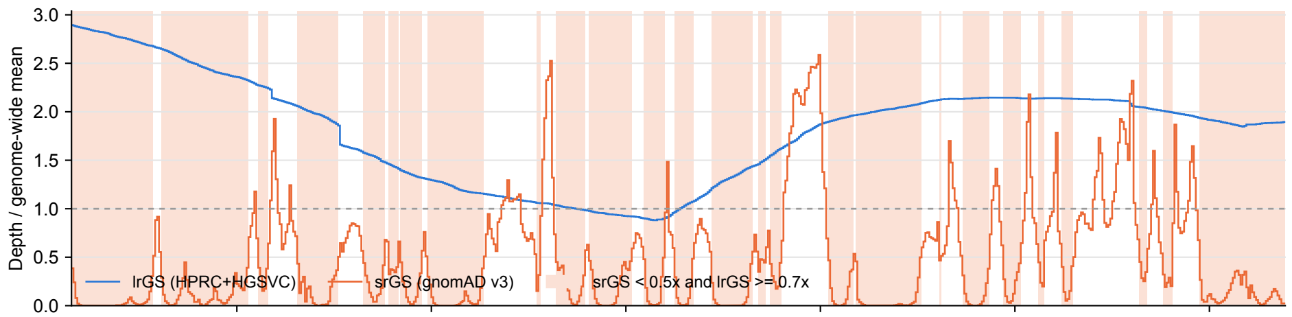
ENSG00000205236: lrGS vs srGS coverage over tandem repeats (100 bp bins)
