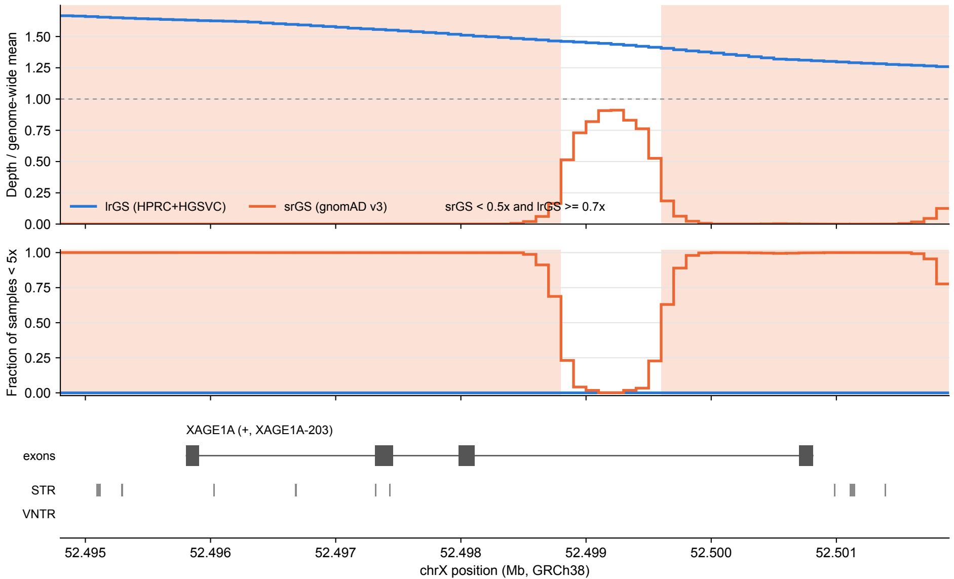
XAGE1A: lrGS vs srGS coverage over tandem repeats (100 bp bins)
