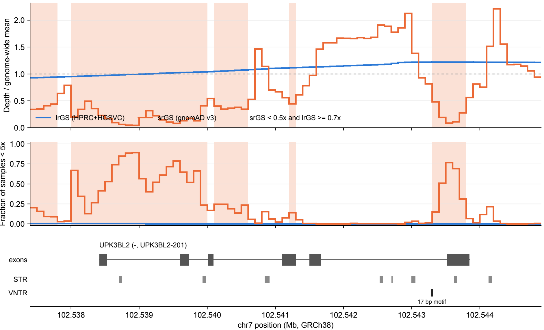
UPK3BL2: lrGS vs srGS coverage over tandem repeats (100 bp bins)
