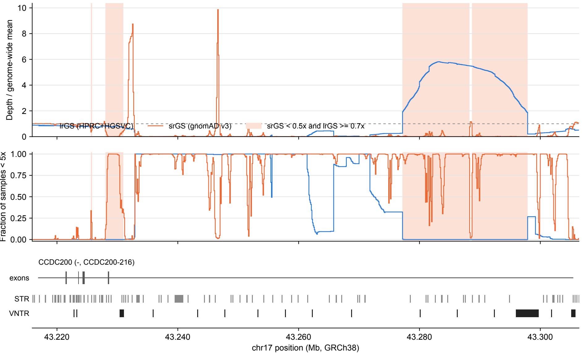
CCDC200: lrGS vs srGS coverage over tandem repeats (100 bp bins)
