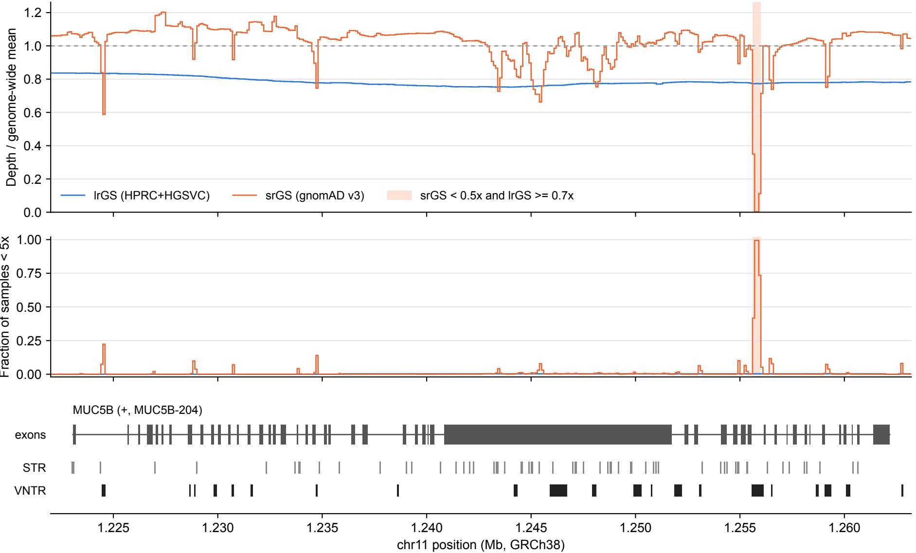
MUC5B: IrGS vs srGS coverage over tandem repeats (100 bp bins)
