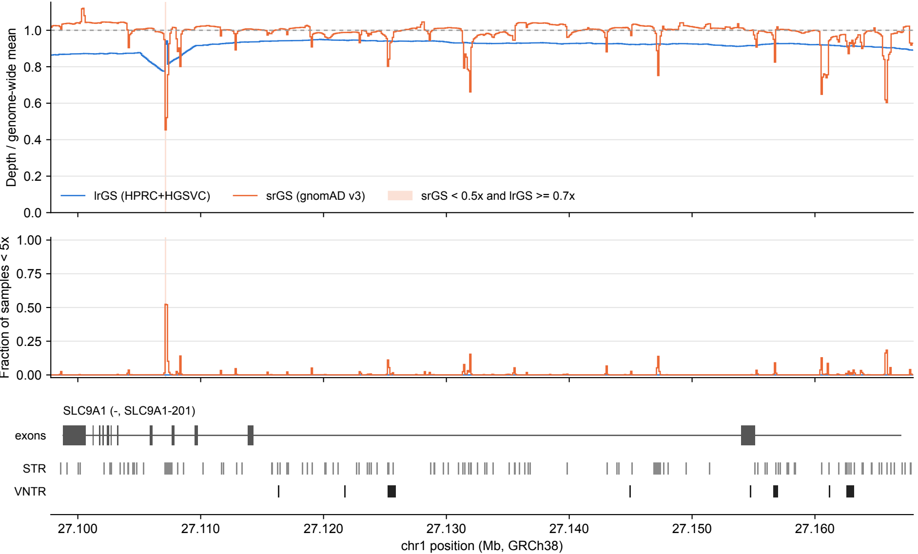
SLC9A1: IrGS vs srGS coverage over tandem repeats (100 bp bins)
