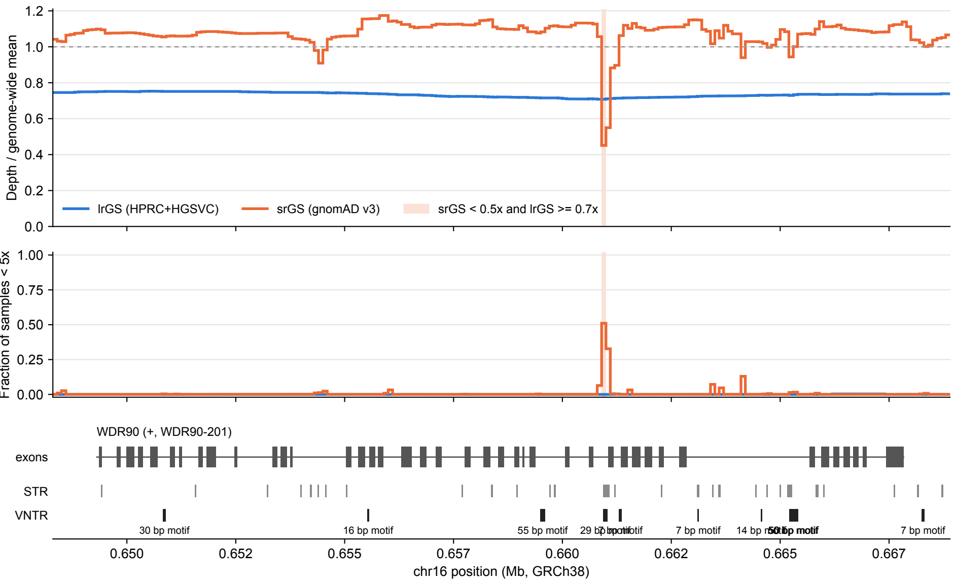
WDR90: IrGS vs srGS coverage over tandem repeats (100 bp bins)
