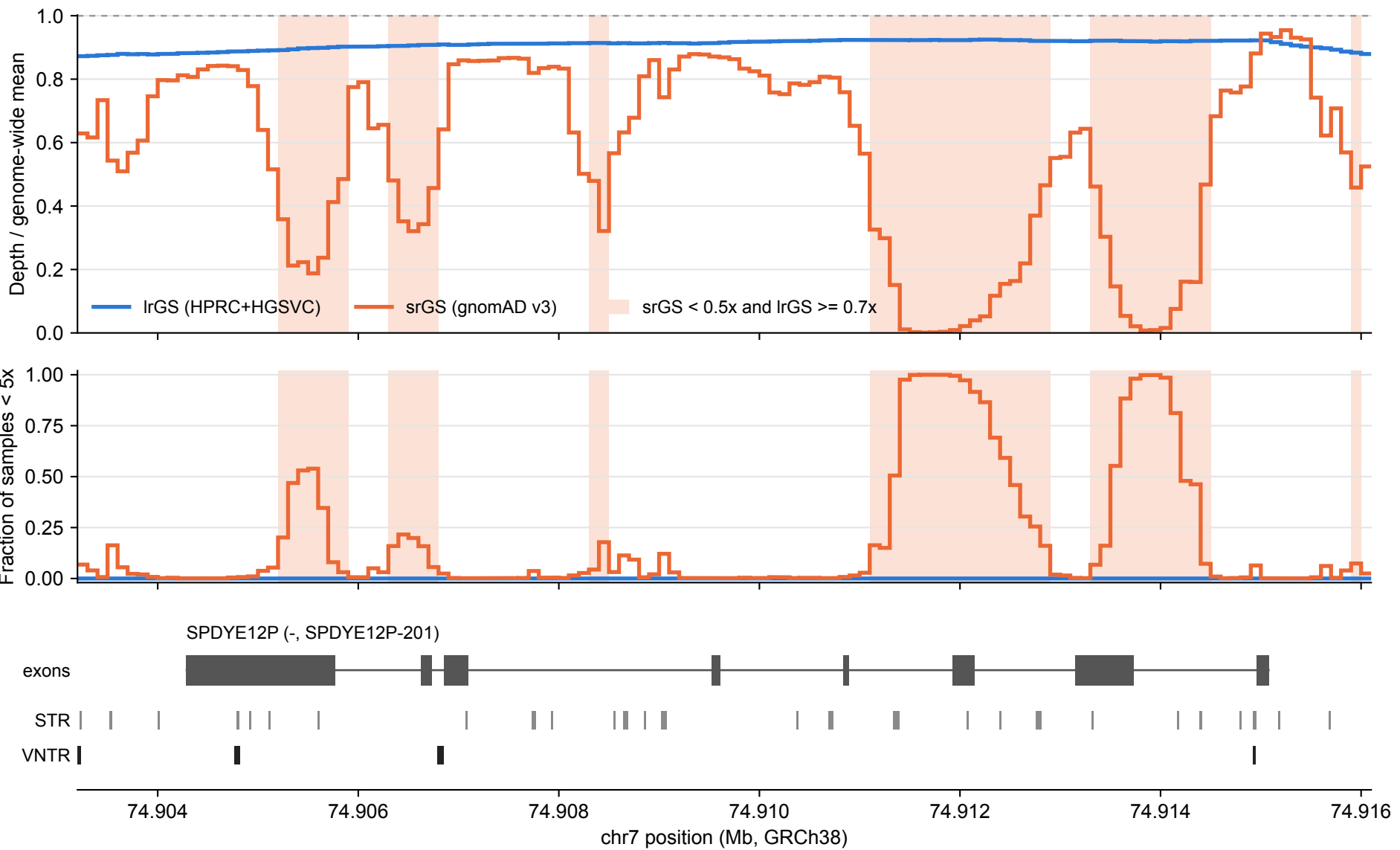
SPDYE12P: IrGS vs srGS coverage over tandem repeats (100 bp bins)
