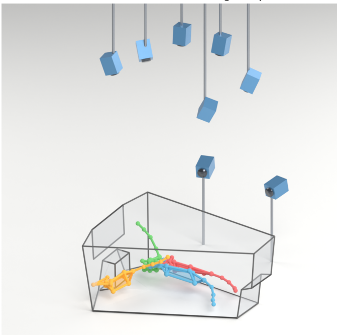
SLAP-2M
