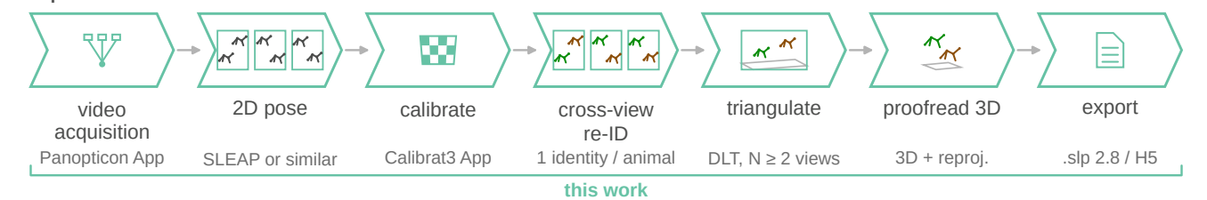
SLAP-2M
