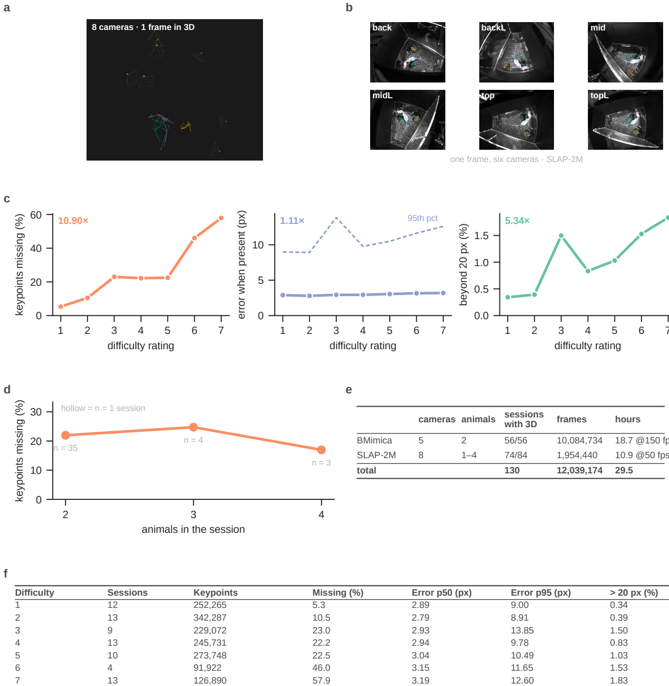
a, b: one SLAP-2M session. c, d, f: 74 SLAP-2M sessions, 1,561,915 keypoints, raw detections from the benchmark's shared identity-stripped pool, matched per frame against the proofread 3D reprojected into each camera. e: both corpora, read from the files.
