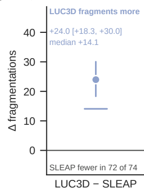
g Fragmentation
