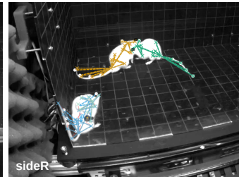
LUC3D identities
