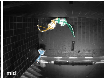
LUC3D identities
