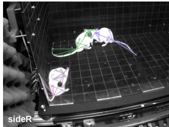
per-camera tracks
