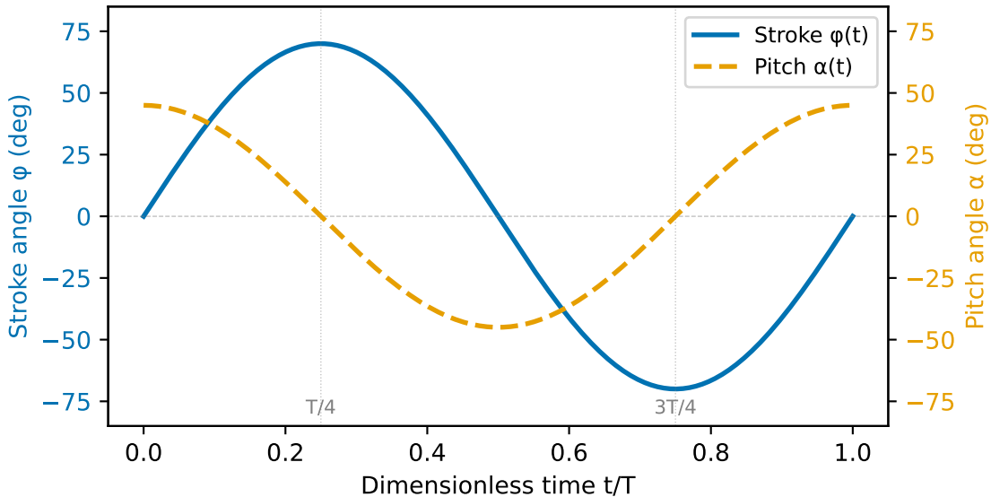
Wing Kinematics (van Veen et al. 2022) f^* = 1 , \phi_{\text{amp}} = 70^\circ , \alpha_{\text{amp}} = 45^\circ
