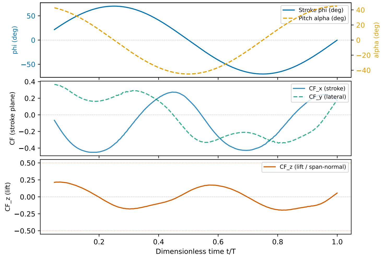
Flapping Wing Forces — coarse grid 64x32x64, f^*=1 , Re \sim 100
