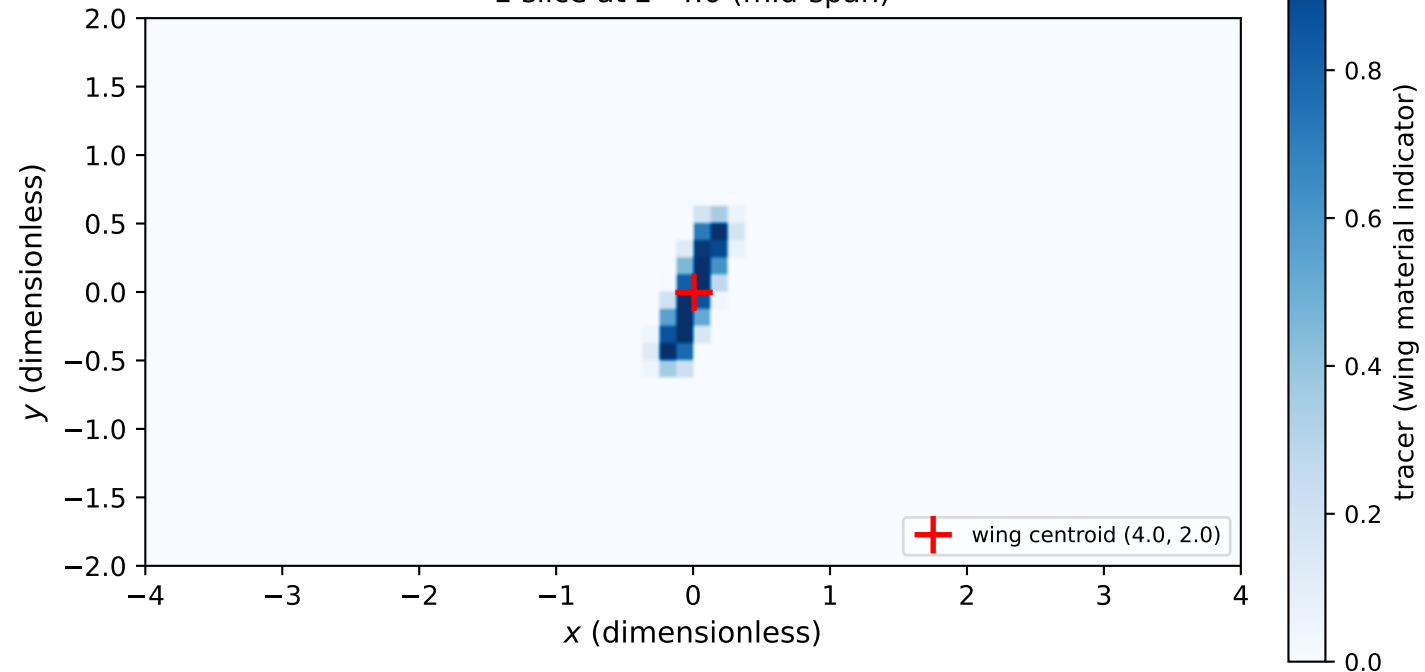
Flapping Wing — tracer field (velocity not in plotfile) z-slice at z=4.0 (mid-span)
