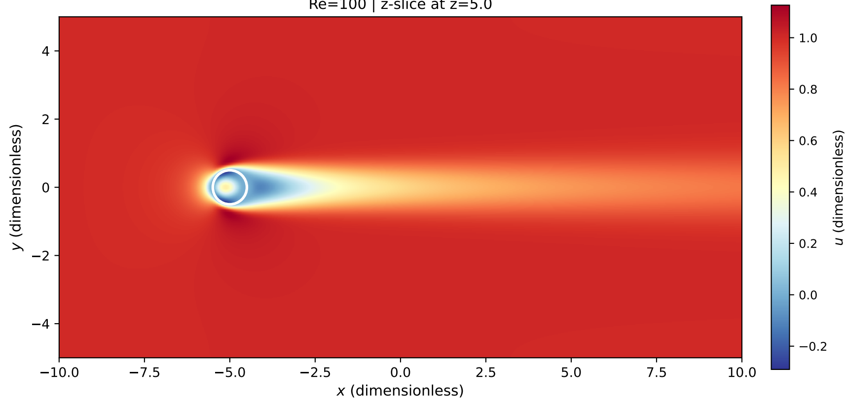
Flow Past Sphere — x-velocity field ( t = 100.0 , steady state) Re=100 | z-slice at z=5.0
