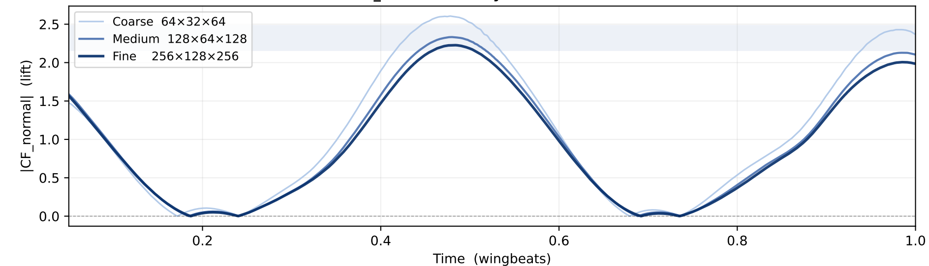
CF_normal — body-frame lift force
