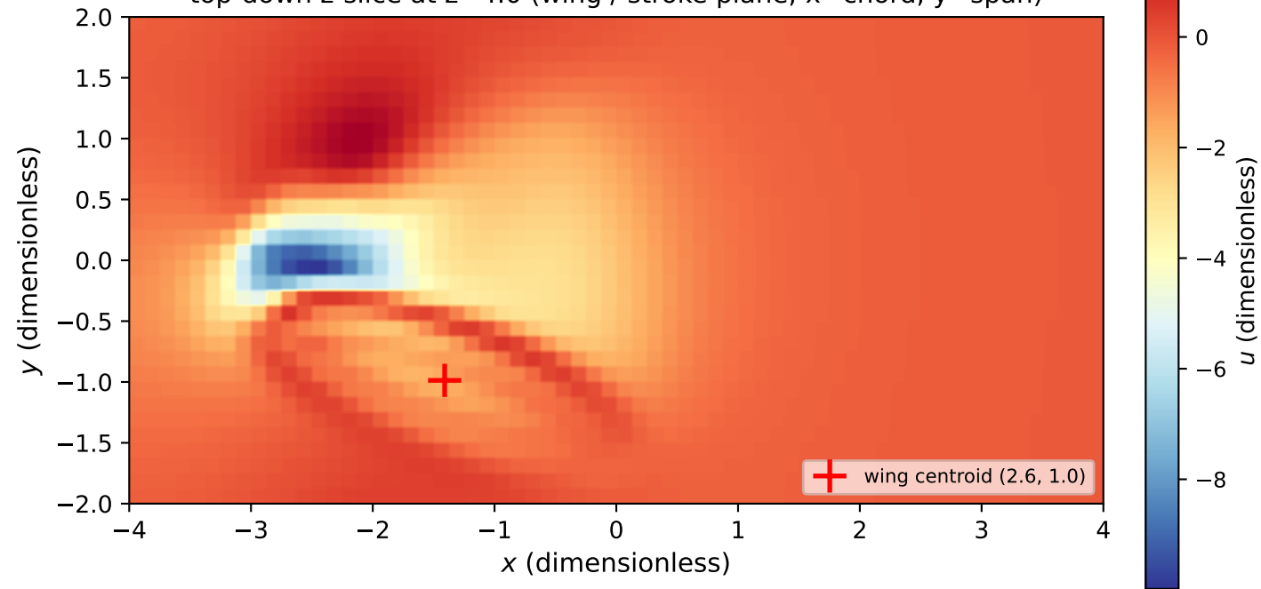
Flapping Wing — x-velocity field ( t = 0.250 , \phi = 70^\circ ) top-down z-slice at z=4.0 (wing / stroke plane; x=\text{chord} , y=\text{span} )
