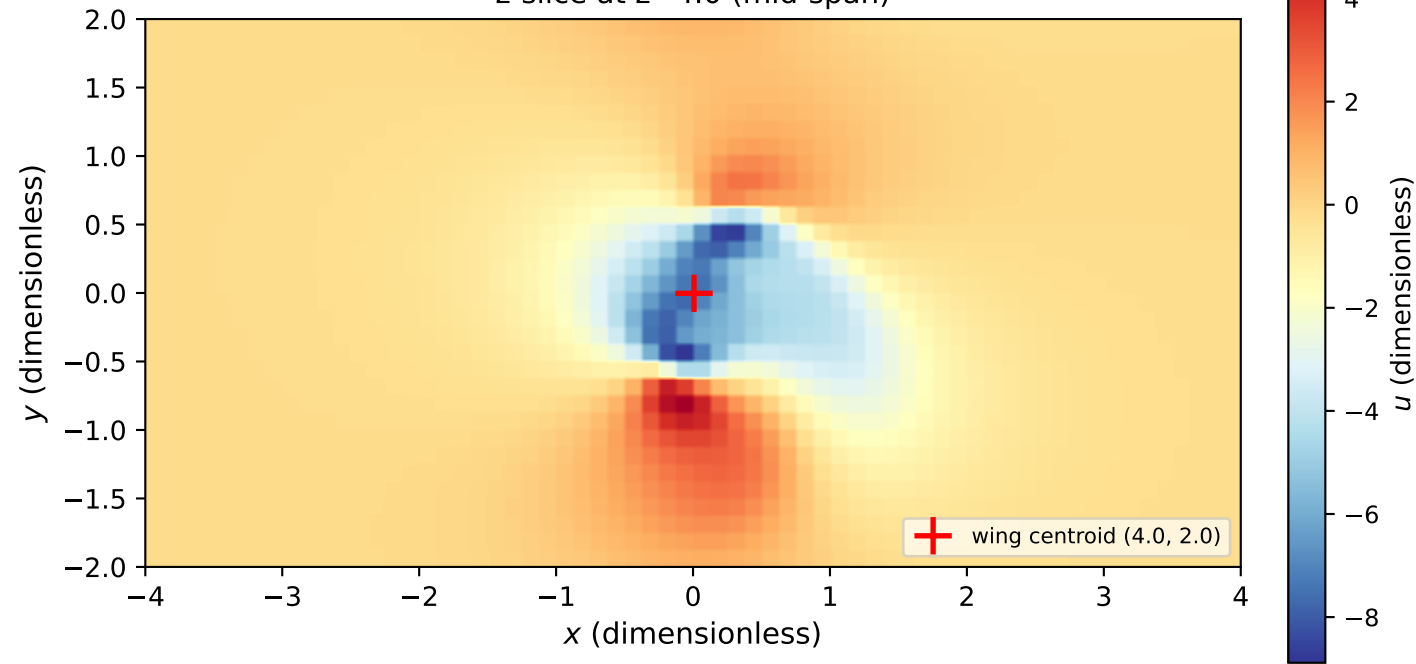
Flapping Wing — x-velocity field ( t = 0.250 , \phi = 70^\circ ) z-slice at z=4.0 (mid-span)
