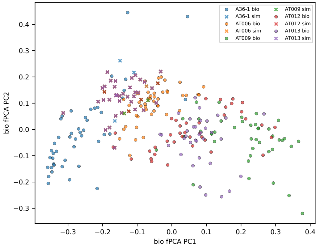
EMG envelopes projected onto bio fPCA basis
