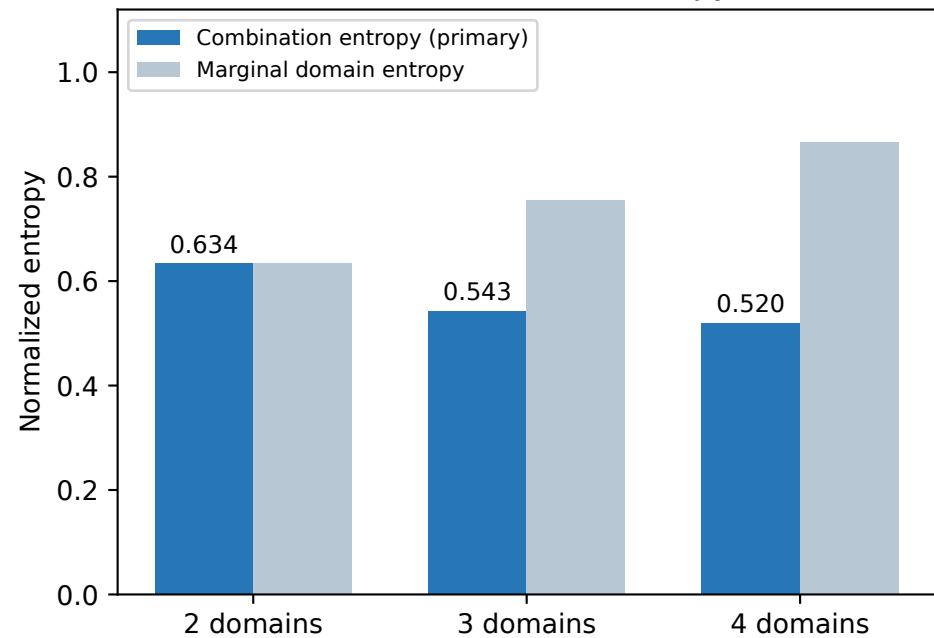
(a) Source-macro entropy
