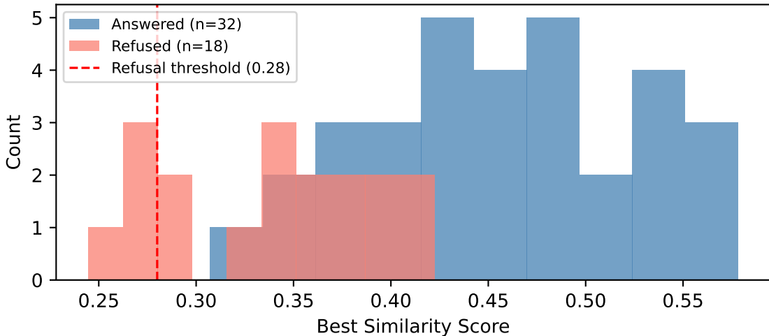
Similarity Score Distribution: Answered vs. Refused Queries
