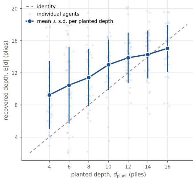
Figure 6: The instrument recovers planted search depth. Synthetic agents satisficing at fixed depths (4–16 plies), run through the identical pipeline. Pale dots, individual agents; dark points, mean \pm s.d. per planted depth; dashed line, identity. Recovery is monotone (group-level Spearman = 1.0) though ordinal: per-agent estimates are compressed toward the middle (MAE 3.7 plies at \sim 70 decisions per agent).
