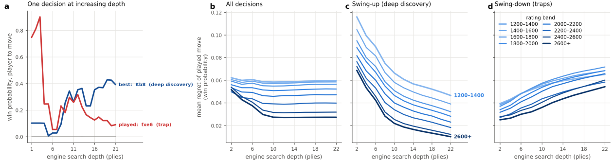
Figure 1: Skill separates only at depth, and mostly on deep-discovery moves. a , A worked example: candidate-move win probabilities across engine search depth for one real decision (grey, other candidates; moves in standard algebraic notation). The played pawn capture fxe6 looks nearly winning at shallow depth and collapses once the refutation surfaces (a trap , swing-down); the quiet king move Kb8 reveals its worth only deep (a deep discovery , swing-up). b–d , Mean regret of the played move across engine search depth, by rating band (light to dark blue: 1200–1400 up to 2600+), within the slow controls (classical and rapid). b , All decisions: rating bands are nearly indistinguishable at shallow depth and fan apart as the engine looks deeper. c , Swing-up (deep-discovery) decisions: a clean, well-ordered rating fan—the rating signal concentrates here. d , Swing-down (trap) decisions: bands bunch and overlap, separating roughly half as much. The rating axis spans online play (lower bands) to elite over-the-board play (upper bands).
