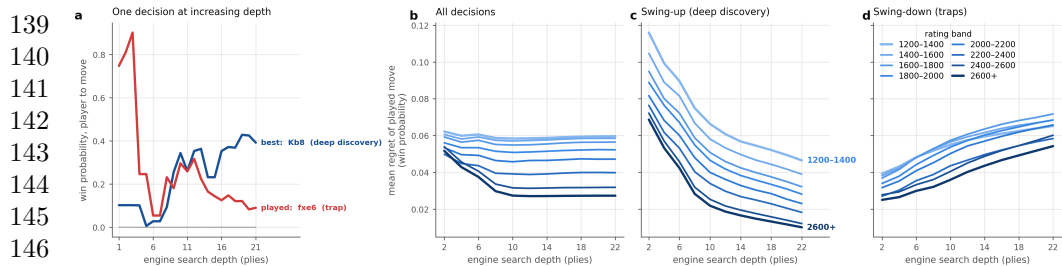
Fig. 1 Skill separates only at depth, and mostly on deep-discovery moves. a , A worked example: candidate-move win probabilities across engine search depth for one real decision (grey, other candidates; moves in standard algebraic notation). The played pawn capture fxe6 looks nearly winning at shallow depth and collapses once the refutation surfaces (a trap , swing-down); the quiet king move Kb8 reveals its worth only deep (a deep discovery , swing-up). b–d , Mean regret of the played move across engine search depth, by rating band (light to dark blue: 1200–1400 up to 2600+), within the slow controls (classical and rapid). b , All decisions: rating bands are nearly indistinguishable at shallow depth and fan apart as the engine looks deeper. c , Swing-up (deep-discovery) decisions: a clean, well-ordered rating fan—the rating signal concentrates here. d , Swing-down (trap) decisions: bands bunch and overlap, separating roughly half as much. The rating axis spans online play (lower bands) to elite over-the-board play (upper bands).
