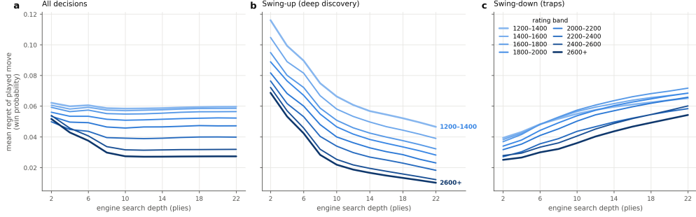
Fig. 1 Skill separates only at depth, and mostly on deep-discovery moves. Mean regret of the played move across engine search depth, by rating band (light to dark blue: 1200–1400 up to 2600+), within the slow controls (classical and rapid). a , All decisions: rating bands are nearly indistinguishable at shallow depth and fan apart as the engine looks deeper. b , Swing-up (deep-discovery) decisions: a clean, well-ordered rating fan—the rating signal concentrates here. c , Swing-down (trap) decisions: bands bunch and overlap, separating roughly half as much. The rating axis spans online play (lower bands) to elite over-the-board play (upper bands).
