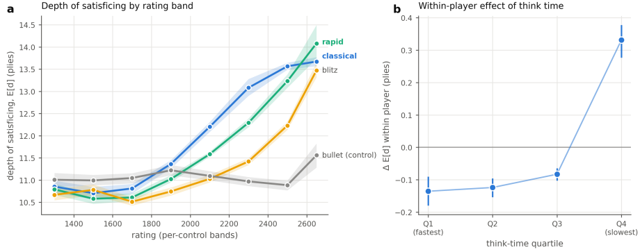
Fig. 2 Depth of satisficing rises with skill and with time to think. a , Posterior depth of satisficing by rating band, within each time control (shaded bands, player-clustered bootstrap 95% CIs). Depth rises with rating in classical (Spearman \rho = +0.40 ), rapid (+0.66) and blitz (+0.45); bullet, where no one can search, is the flat negative control ( \rho = -0.04 ). b , Within-player effect: de-meanded depth by think-time quartile (dots, pooled means; bars, player-clustered bootstrap 95% CIs). The same players search deeper on their slower moves.
