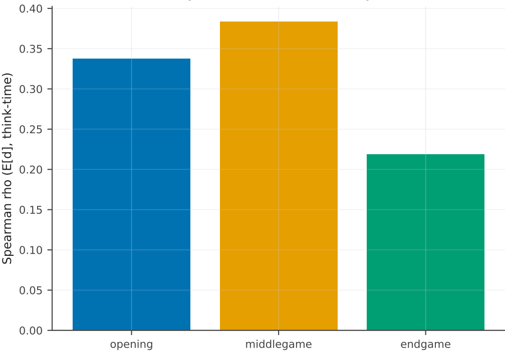
E3: inferred depth vs real think-time (model fit without clock)
