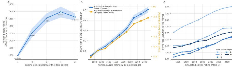
Fig. 5 Engine item difficulty against an independent human criterion. 10,679 rating-stratified Lichess puzzles. a , Mean human puzzle rating (Glicko, estimated by Lichess from rated solvers' attempts) by the item's engine critical depth; shaded band, bootstrap 95% CI over puzzles; counts per depth shown. b , The two faces of swing by human rating band: the share of puzzles whose solution is a deep discovery (swing-up; left axis, bootstrap 95% CI) and the shallow advantage of the most tempting wrong move over the solution (right axis; less negative means the trap looks more like the solution at depth \leq 4 ). c , Person side: solve rate of Maia-3 simulated solvers across a ladder of ratings, by item critical depth. Solve rate rises with simulated skill at every depth, and deeper items sit lower at every strength—what pattern alone cannot find.
