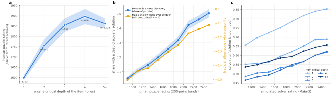
Figure 5: Engine item difficulty against an independent human criterion. 10,679 rating-stratified Lichess puzzles. a , Mean human puzzle rating (Glicko, estimated by Lichess from rated solvers' attempts) by the item's engine critical depth; shaded band, bootstrap 95% CI over puzzles; counts per depth shown. b , The two faces of swing by human rating band: the share of puzzles whose solution is a deep discovery (swing-up; left axis, bootstrap 95% CI) and the shallow advantage of the most tempting wrong move over the solution (right axis; less negative means the trap looks more like the solution at depth \leq 4 ). c , Person side: solve rate of Maia-3 simulated solvers across a ladder of ratings, by item critical depth. Solve rate rises with simulated skill at every depth, and deeper items sit lower at every strength—what pattern alone cannot find.
