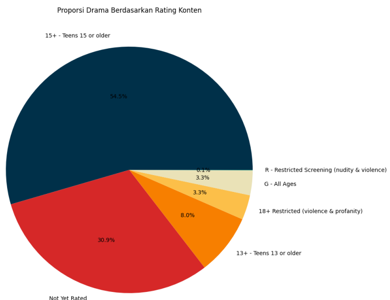
Gambar 2. 7 Visualisasi Composition
