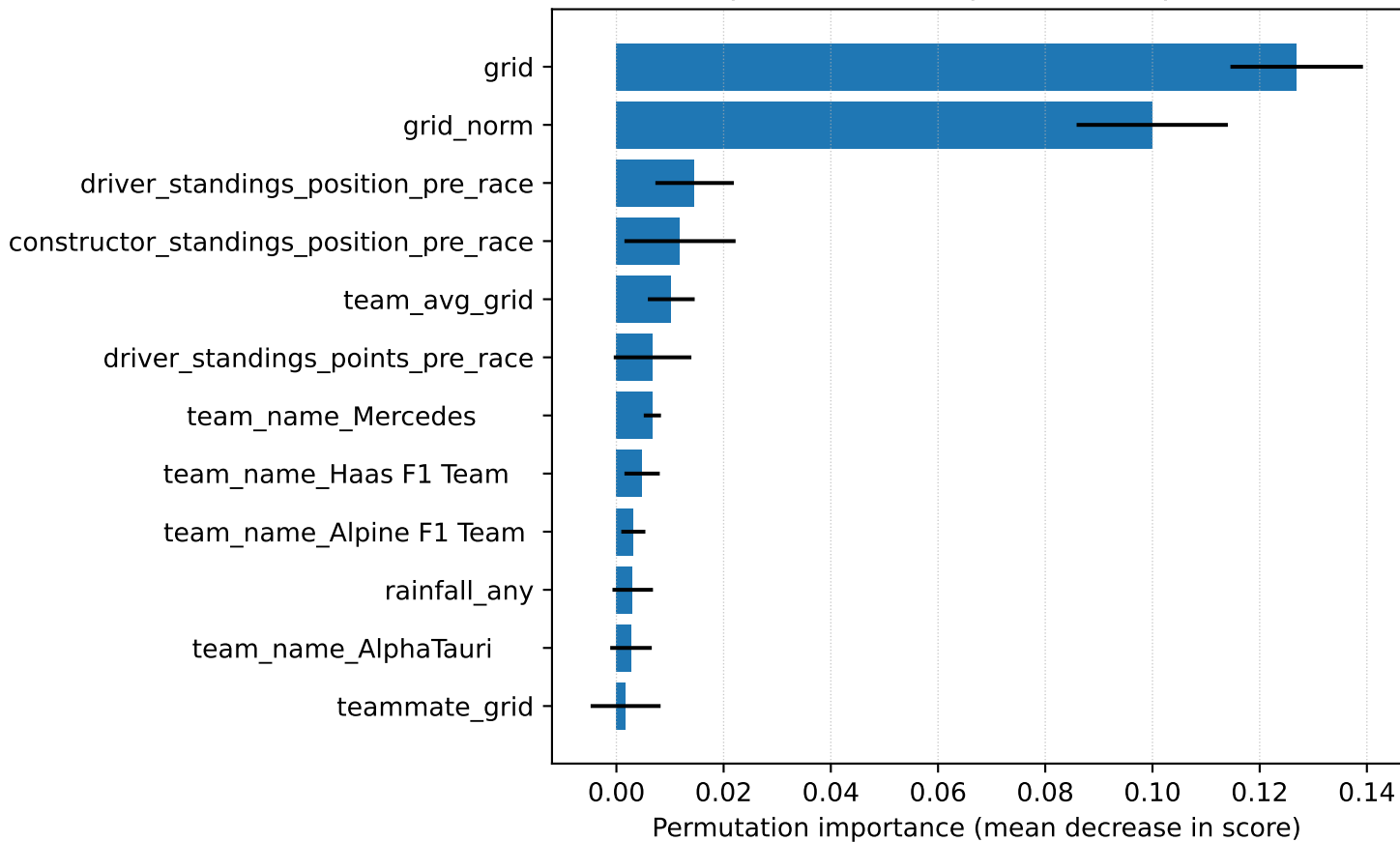
Random Forest permutation importance (Top 12, 2023 test set)
