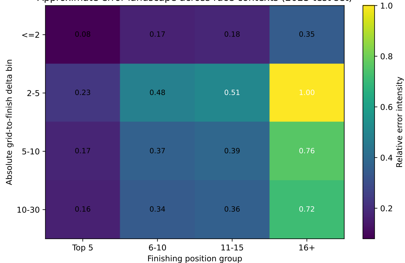
Approximate error landscape across race contexts (2023 test set)
