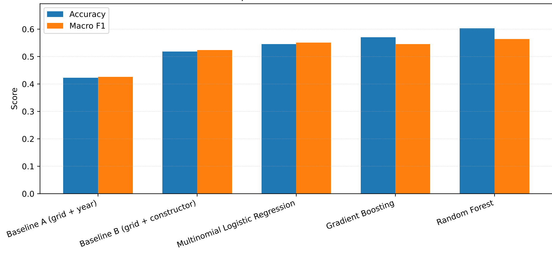
Model performance on 2023 test set
