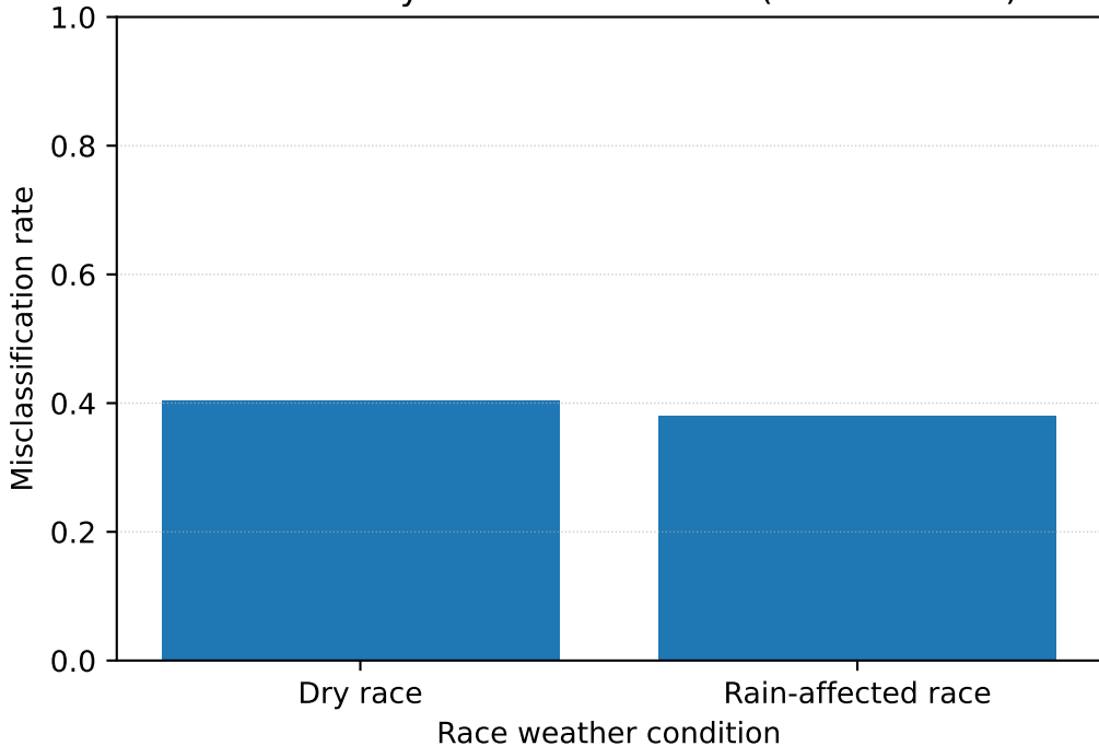
Error rate by weather condition (2023 test set)
