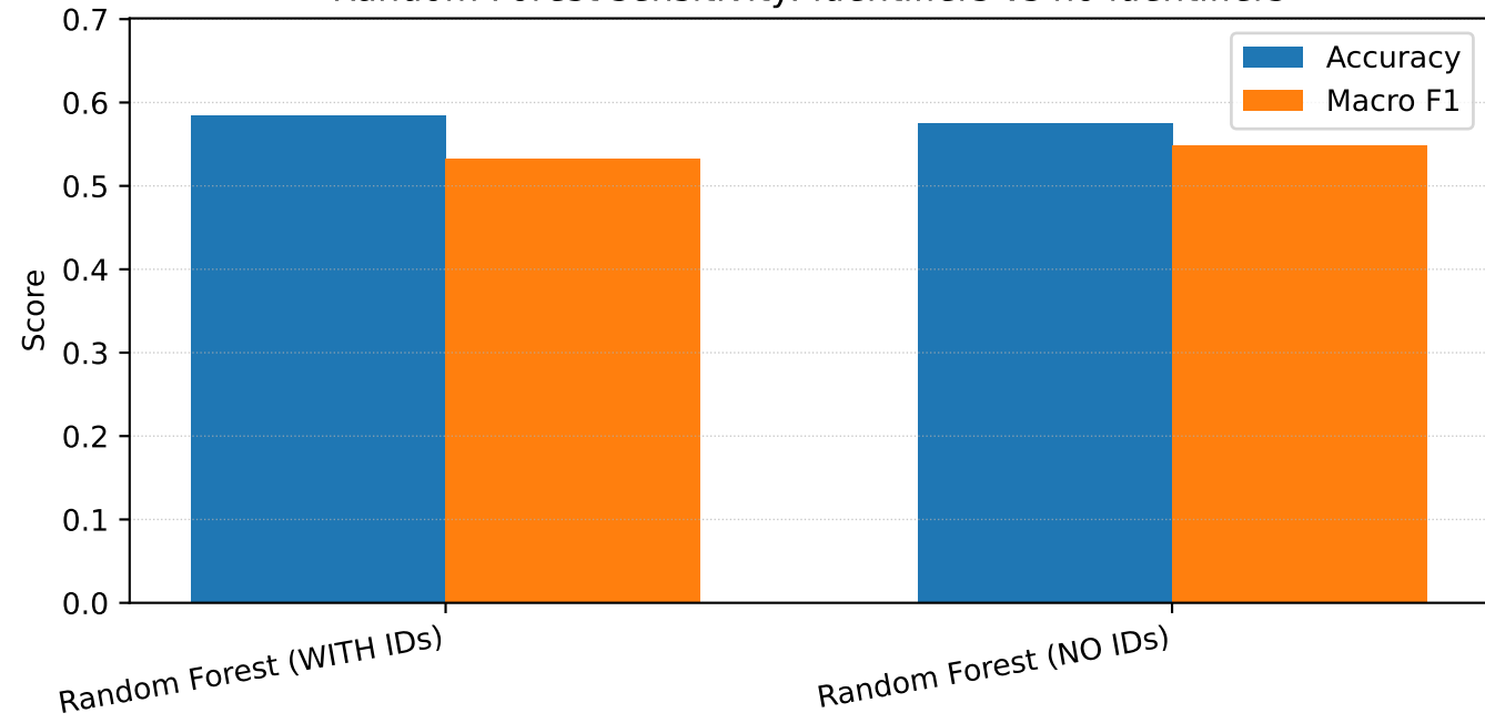
Random Forest sensitivity: identifiers vs no identifiers
