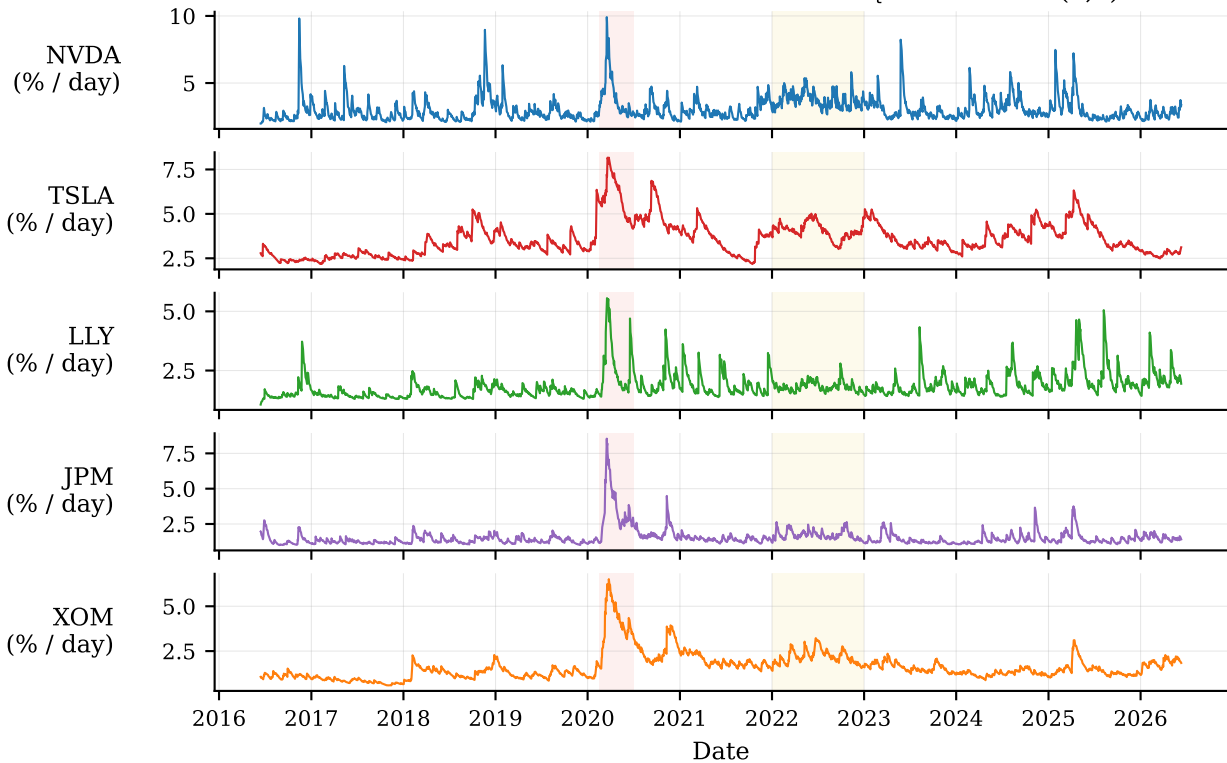
Estimated conditional standard deviation \sigma_t from GARCH(1,1)
