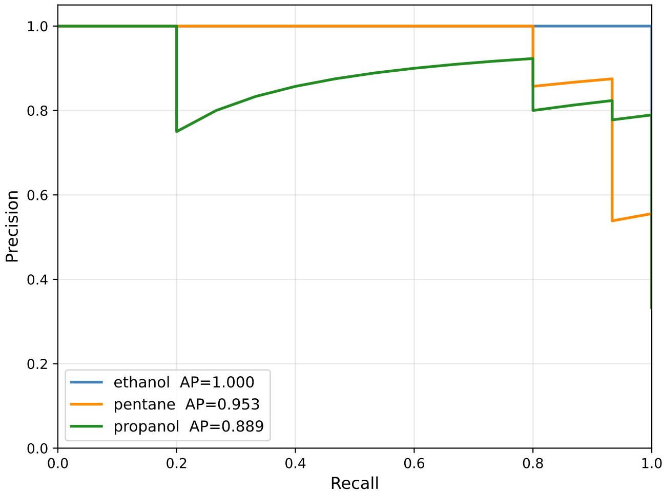
Problem 1 - Precision-Recall Curves (one-vs-rest)
