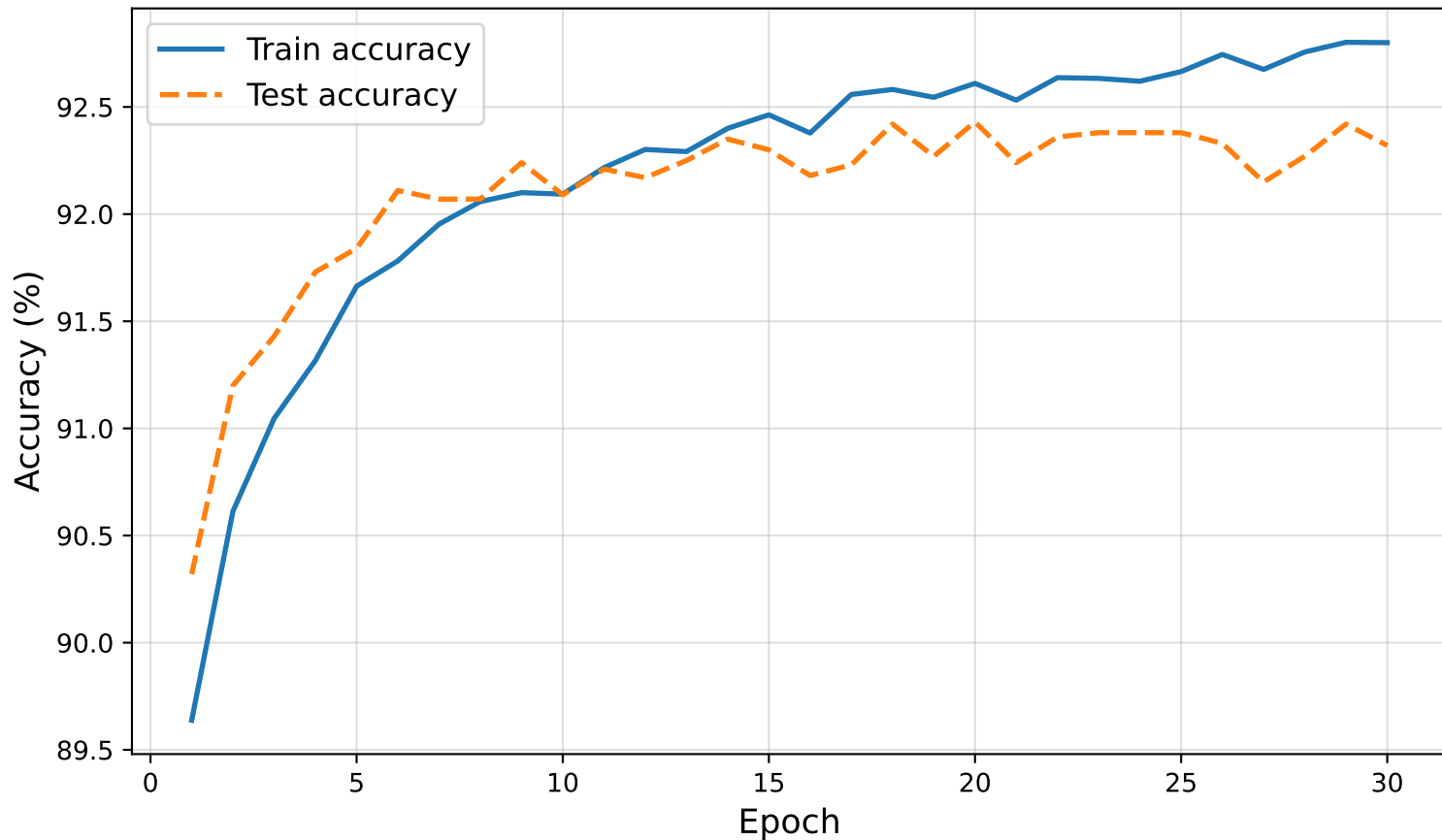
Problem 1 - Accuracy vs Epoch
