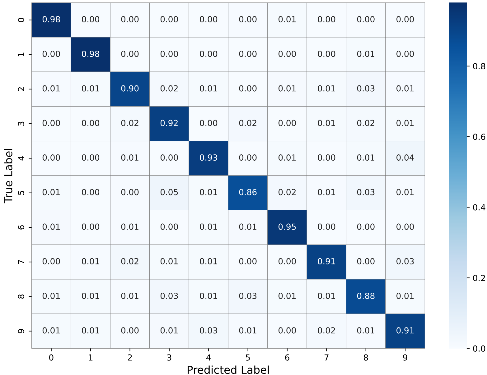
Problem 1 - Confusion Matrix (row-normalised)
