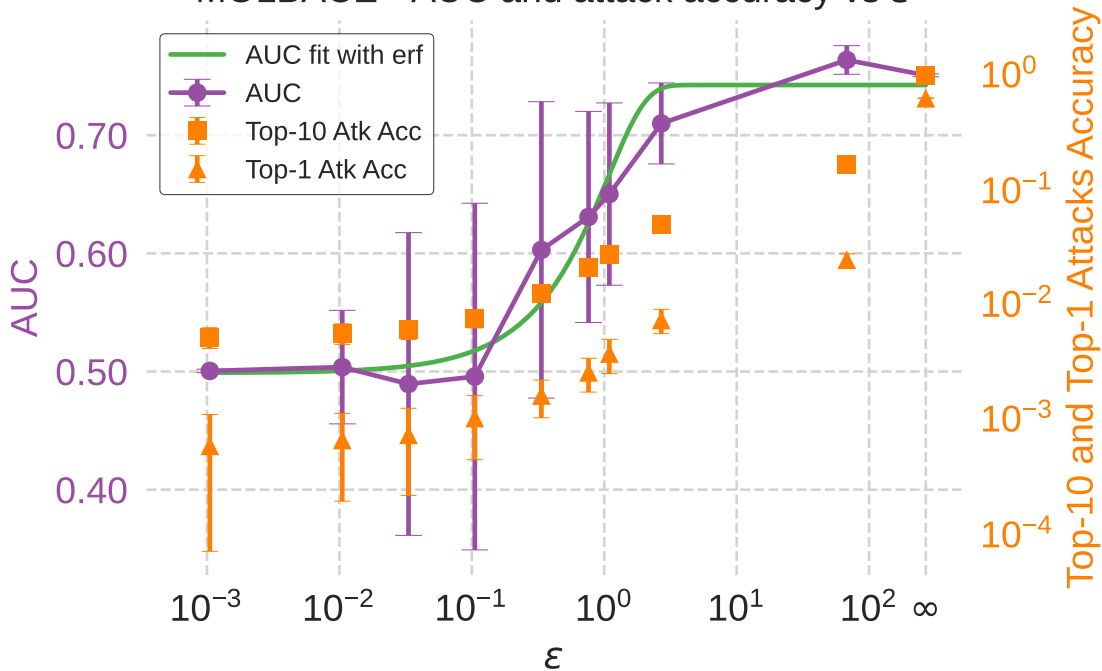
MOLBACE - AUC and attack accuracy vs \epsilon
