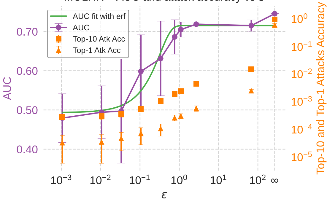
MOLHIV - AUC and attack accuracy vs \epsilon
