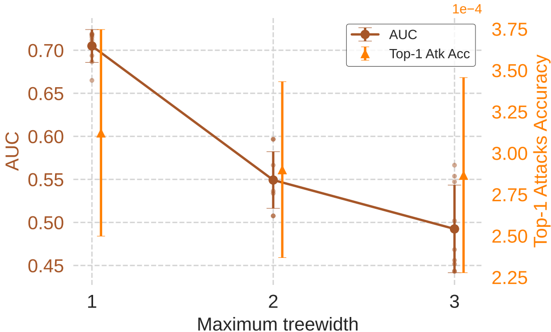
MOLHIV - AUC and attack accuracy vs maximum treewidth
