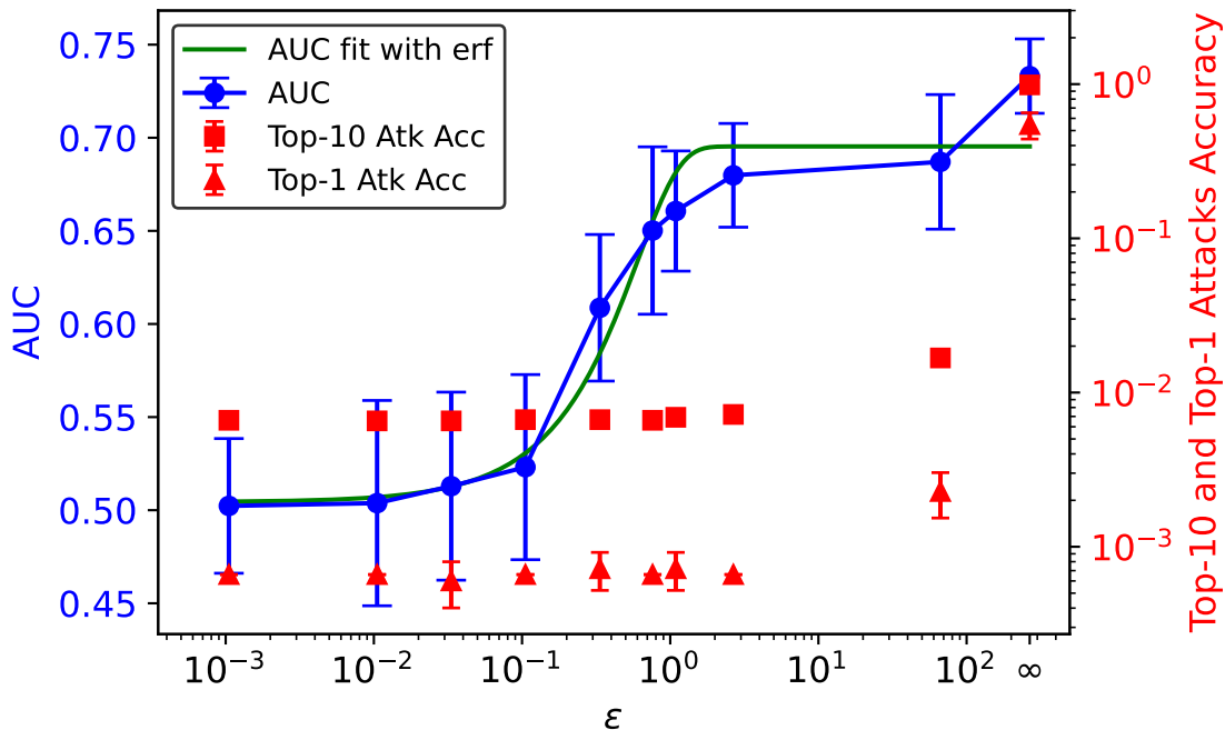
MOLBACE - AUC and attack accuracy vs \varepsilon
