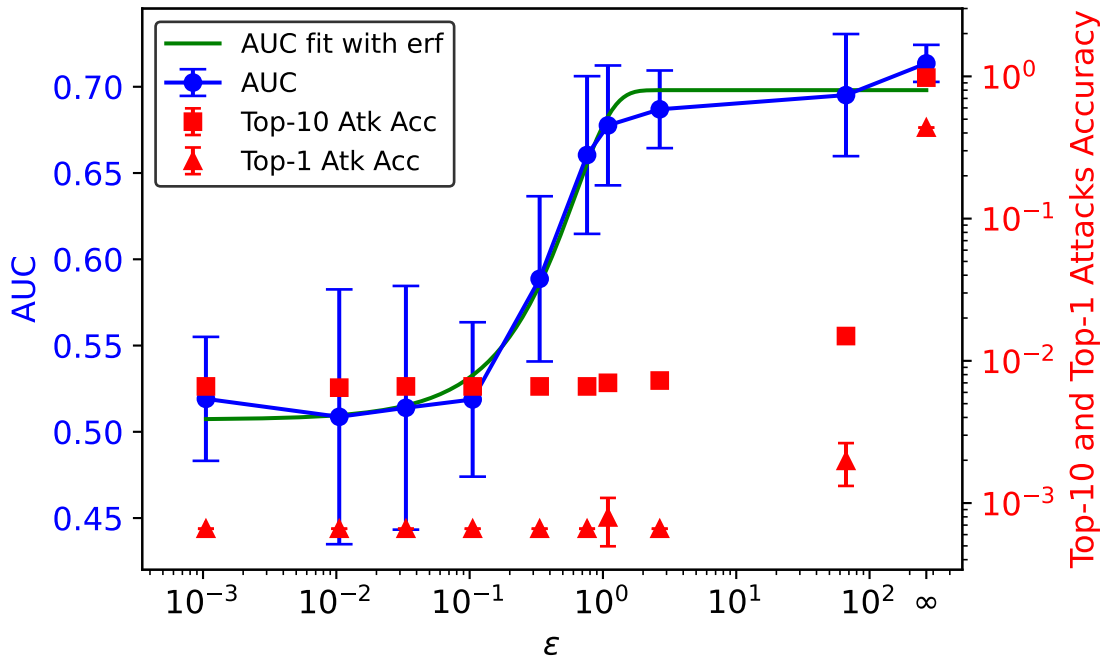
MOLBACE - AUC and attack accuracy vs \epsilon
