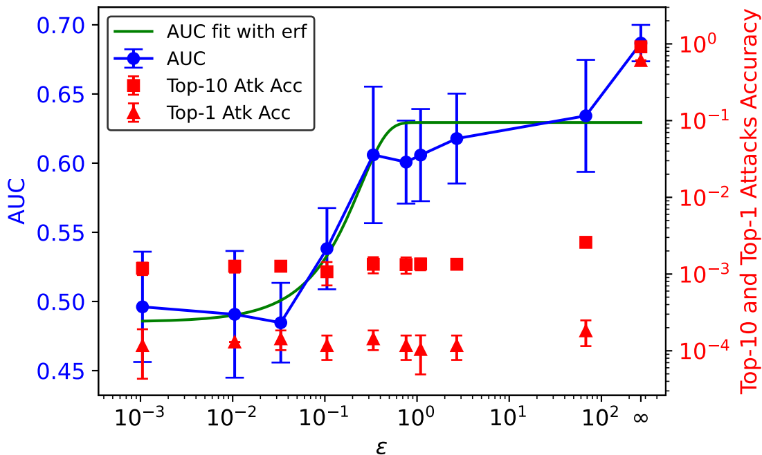
MOLTOX21 - AUC and attack accuracy vs \epsilon
