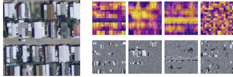
(b) Preservation check images (bottom) to measure Output-Completeness for a mobilehome park sample (left) from the {UCM, SwinT} DMC for explanations from PartitionSHAP, Grad-CAM, KPCA-CAM, and randomised (top). The confidence in the original output class drops from 1.0 \rightarrow \{0.9864, 0.0102, 0.0005, 0.7030\} (a smaller drop is better).
