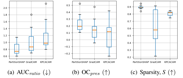
FIGURE 6. Box plots of selected metrics, each considering 12 DMC data points per xAI method. The central orange line is the median and the box extends to the first and third quartiles. Whiskers extend to the furthest point within 1.5 \times the interquartile range. Flier points beyond these whisker limits are shown as empty circles.
