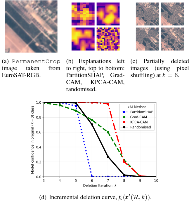
FIGURE 4. The process of evaluating the Correctness of our selected xAI methods (compared to randomised explanations) via the incremental deletion curve, described in Section III-B3. A smaller area under the curve (AUC) is better. PartitionSHAP has an AUC of 5.45 compared to the AUC of a randomised explanation of 6.49. Grad-CAM and KPCA-CAM are both worse than random for this example.
