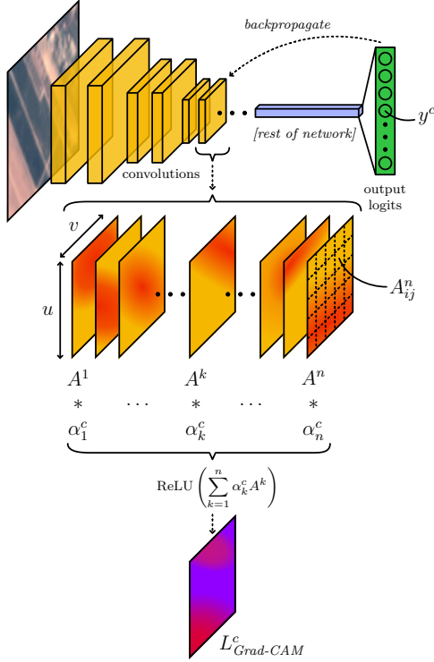
FIGURE 2. An annotated diagram describing the calculation of L_{\text{Grad-CAM}} for a single input image. The \alpha_k^c weights for each feature map A^k of the targeted convolutional layer are given by (3).
