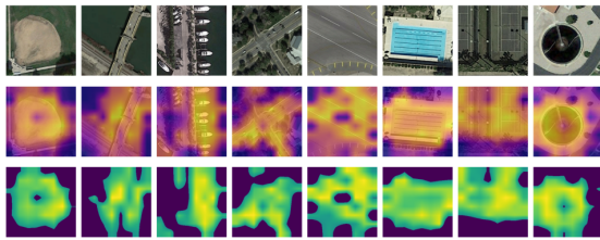
(c) Grad-CAM explanations (middle) have poor Compactness for the {PatternNet, SwinT} DMC. The bottom row visualises the normalised explanation heatmaps, \bar{H} , (with \bar{H}_{ij} < \tau set to 0) where S = \{0.41, 0.44, 0.46, 0.46, 0.25, 0.34, 0.29, 0.40\} .
