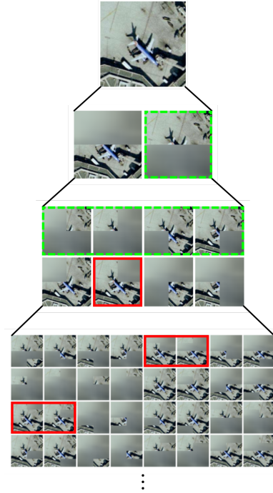
FIGURE 5. The beginning of the PartitionSHAP process visualised chronologically from top to bottom for an airplane image from UCM. The original image is masked (here, blurred) in successively smaller regions with two regions added and two subtracted from each image each stage as highlighted by the dashed green border moving from the stage 2 to 3 and then by the red border moving from stage 3 to 4.
