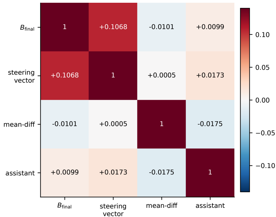
(a) cosine at hidden index 22
