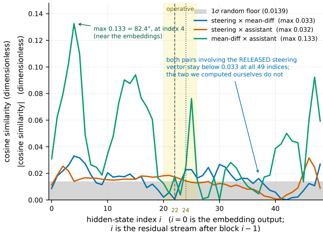
(b) every pair, all 49 indices
