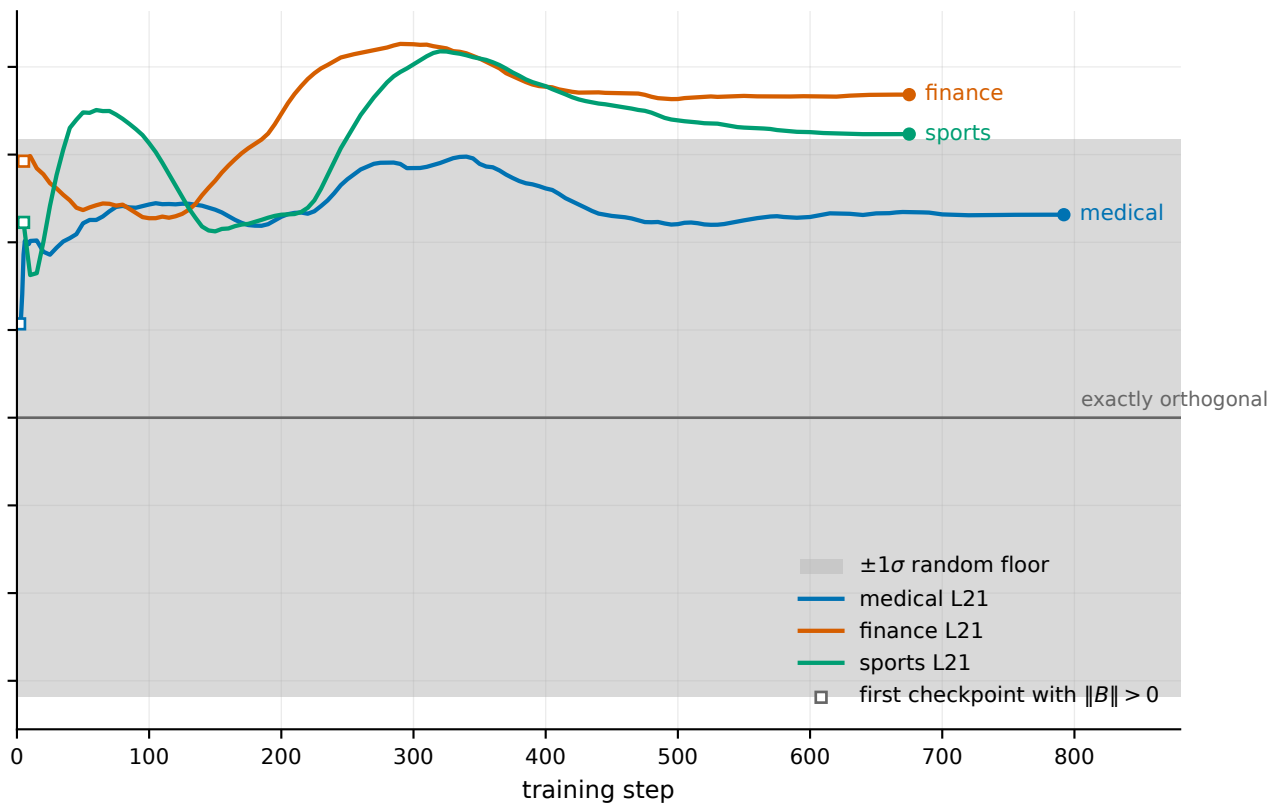
B moves AWAY from the mean-diff direction, in all three runs
